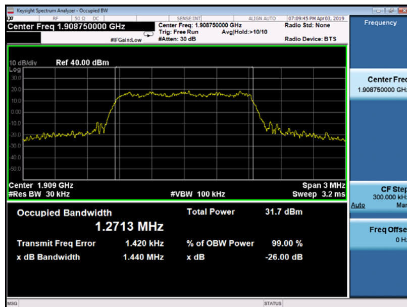
99% &amp; 26dB Occupied Bandwidth Plot on Channel 1175
