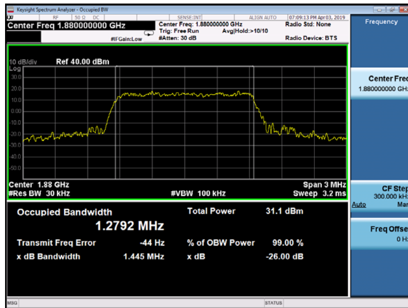
99% &amp; 26dB Occupied Bandwidth Plot on Channel 600
