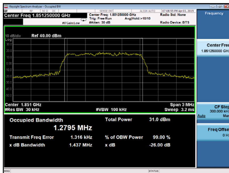
99% &amp; 26dB Occupied Bandwidth Plot on Channel 25
