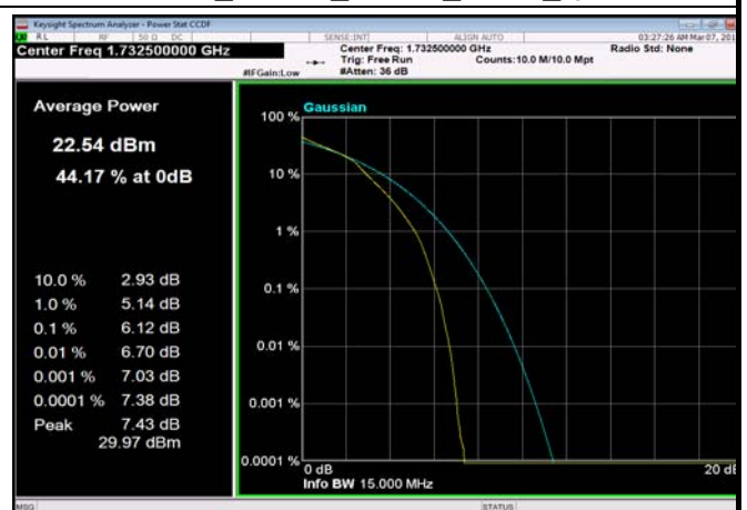
FDD04_15MHz_1732.5_fullRB_Q16
