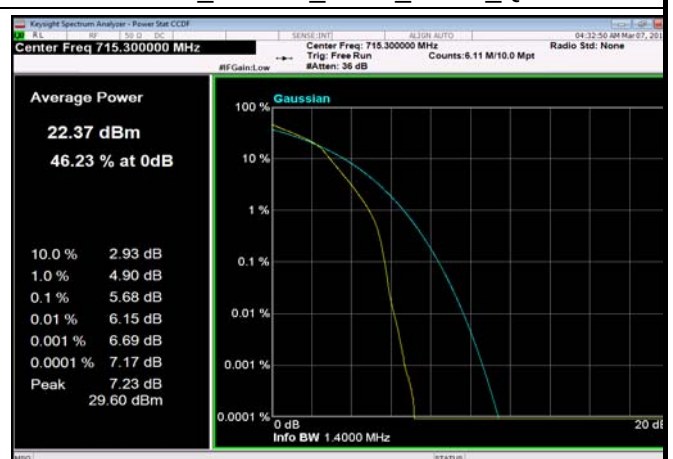
FDD12_1.4MHz_715.3_fullRB_Q16
