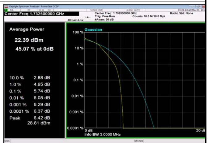
FDD04_3MHz_1732.5_fullRB_Q16
