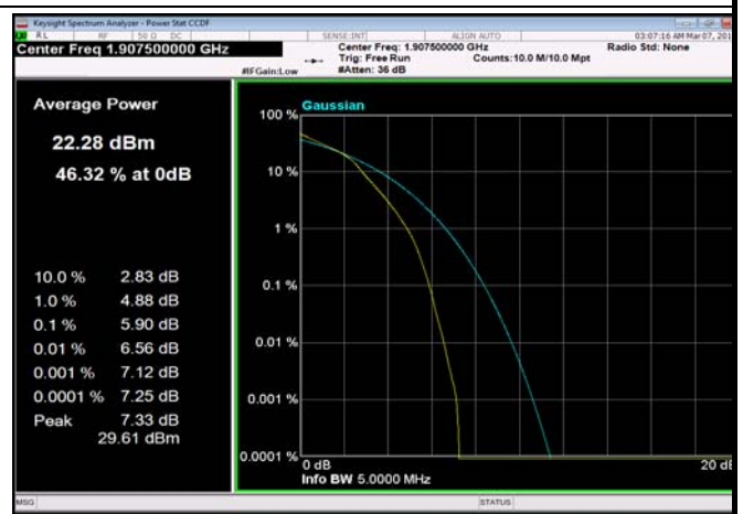
FDD02_5MHz_1907.5_fullRB_Q16
