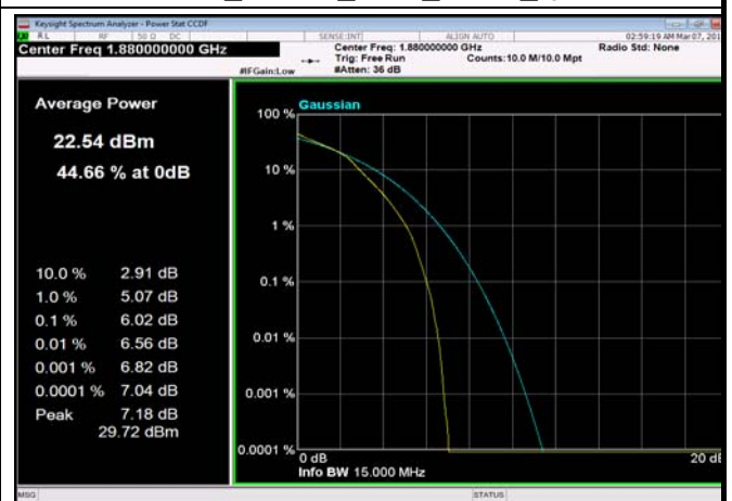
FDD02_20MHz_1880_fullRB_Q16
