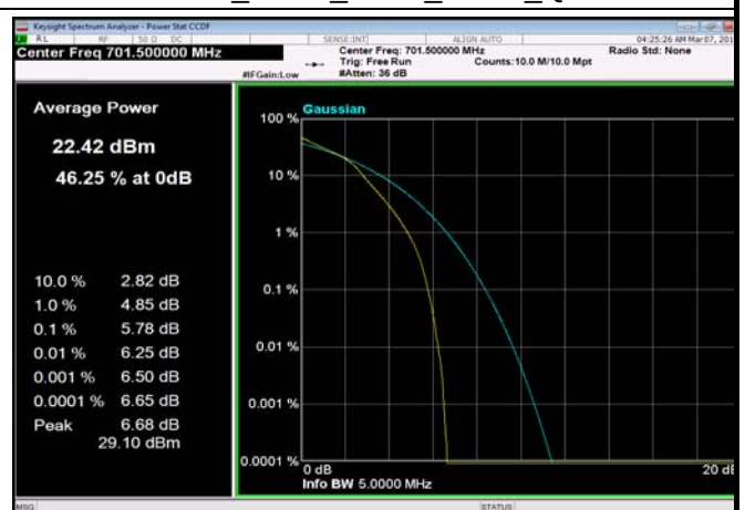
FDD12_5MHz_701.5_fullRB_Q16
