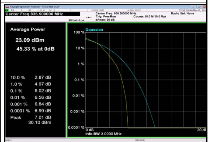
FDD05_5MHz_836.5_fullRB_Q16
