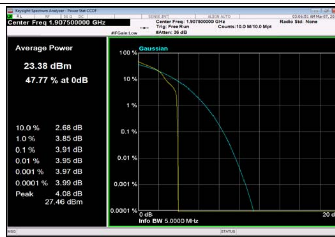
FDD02_5MHz_1907.5_OneRB_high_Q16
