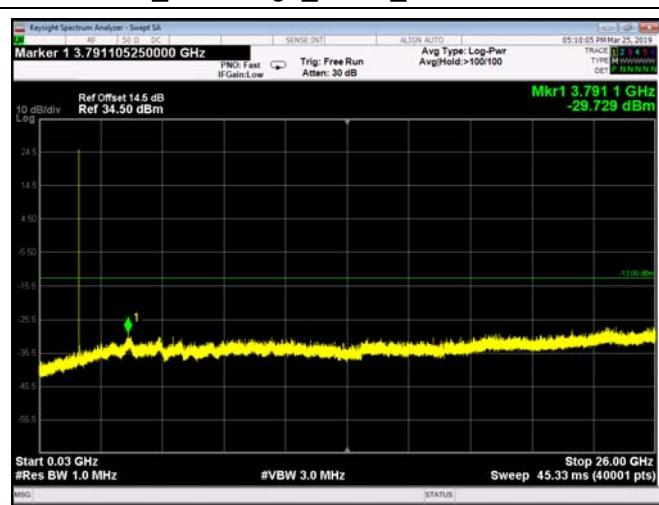
FDD66_LowRange_5MHz_30MHz~26GHz
