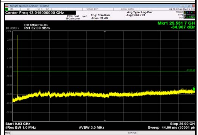
FDD12_MidRange_10MHz_30MHz~26GHz
