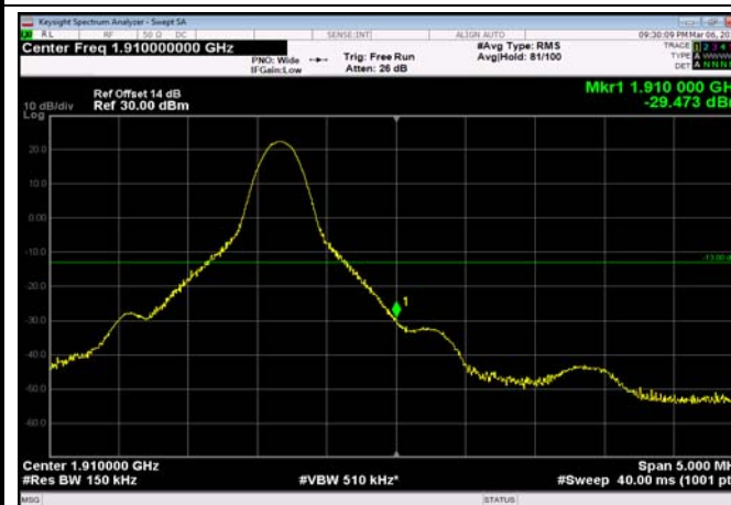
HighRange_FDD02_15MHz_1902.5_OneRB _high_QPSK
