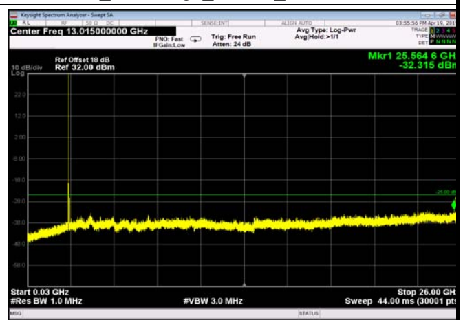
TDD41_LowRange_5MHz_30MHz~26GHz
