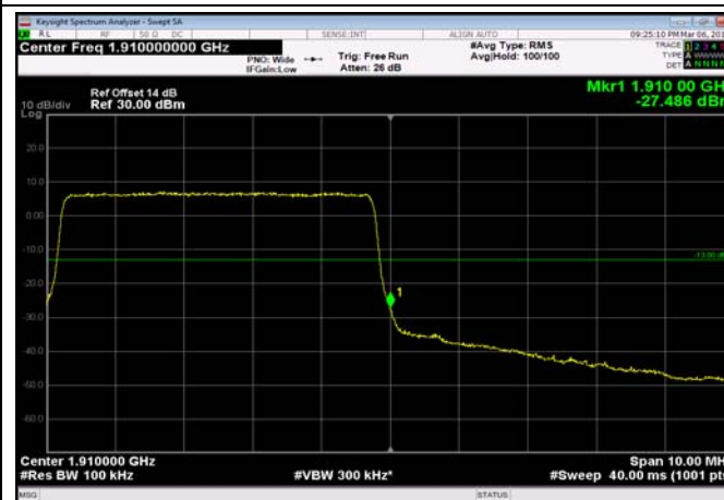
HighRange_FDD02_5MHz_1907.5_fullRB _High_QPSK
