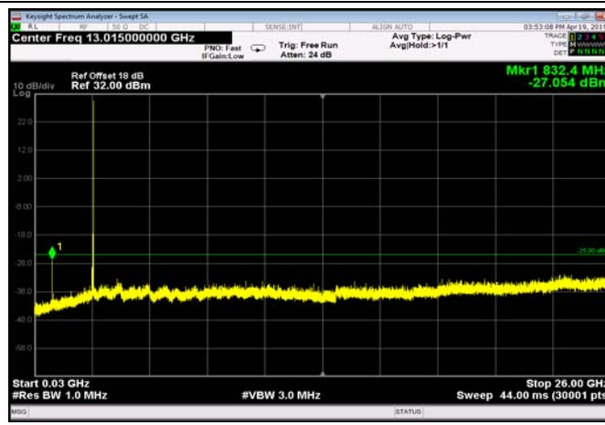
TDD41_HighRange_10MHz_30MHz~26GHz
