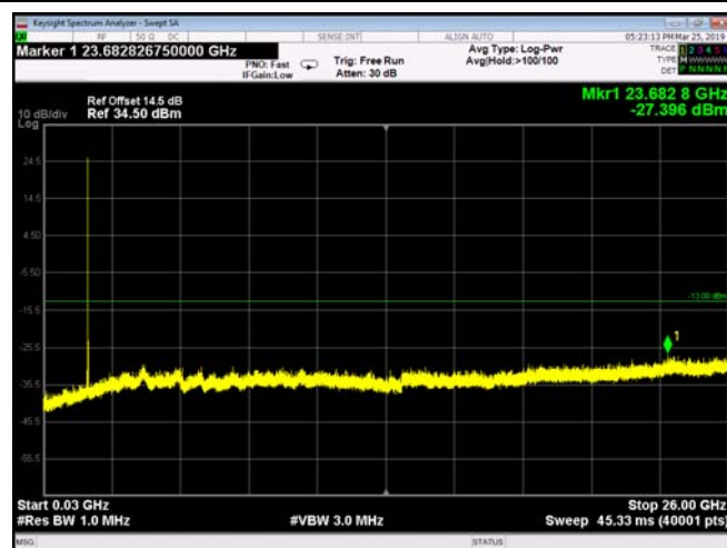
FDD66_LowRange_15MHz_30MHz~26GHz
