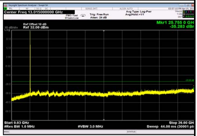
TDD41_HighRange_15MHz_30MHz~26GHz
