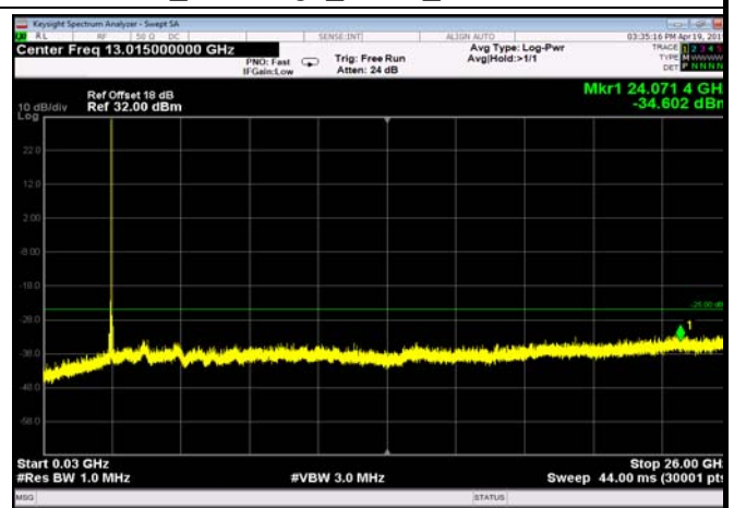
FDD30_HighRange_5MHz_30MHz~26GHz
