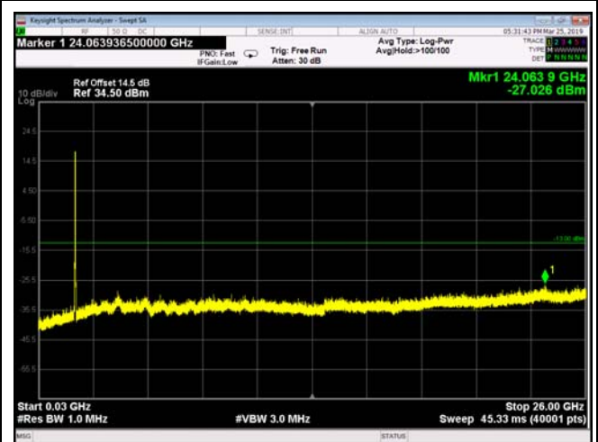
FDD66_HighRange_20MHz_30MHz~26GHz
