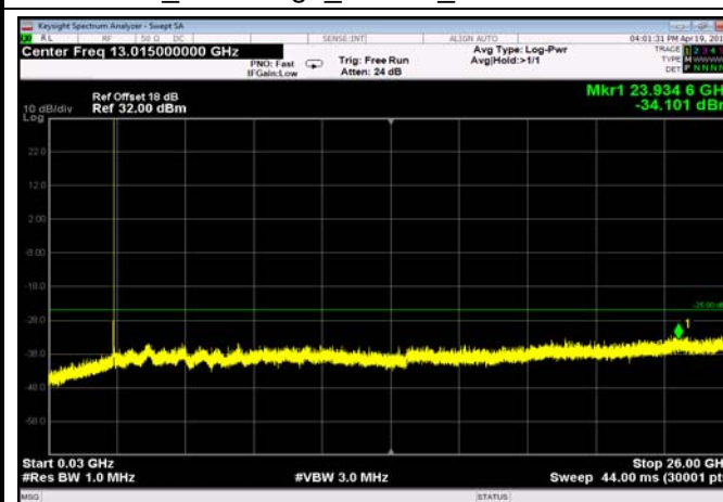
TDD41_LowRange_20MHz_30MHz~26GHz
