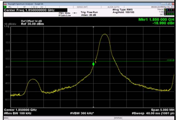
LowRange_FDD02_5MHz_1852.5_fullRB _Low_Q16
