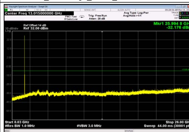
FDD25_LowRange_3MHz_30MHz~26GHz
