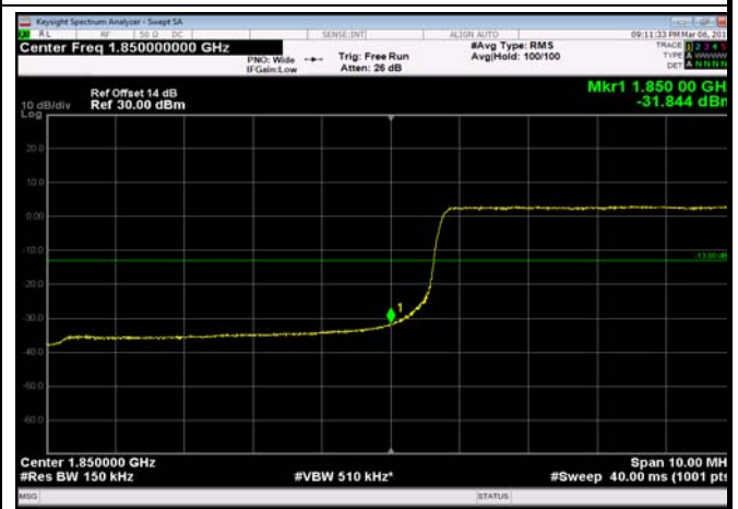
LowRange_FDD02_15MHz_1857.5_fullRB _Low_Q16
