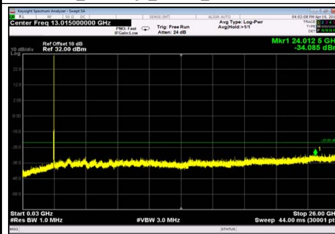
FDD30_HighRange_10MHz_30MHz~26GHz
