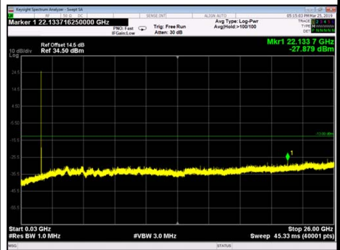
FDD66_HighRange_10MHz_30MHz~26GHz
