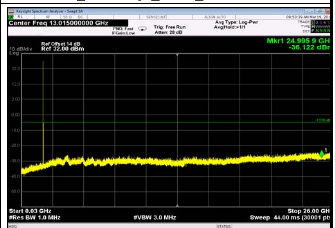
FDD25_LowRange_5MHz_30MHz~26GHz
