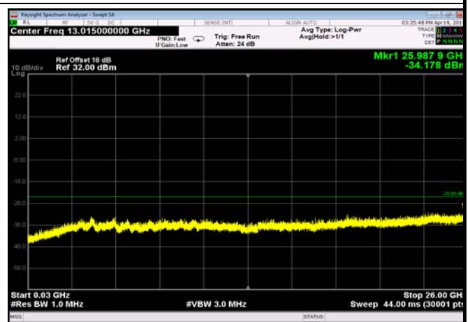
TDD41_LowRange_15MHz_30MHz~26GHz
