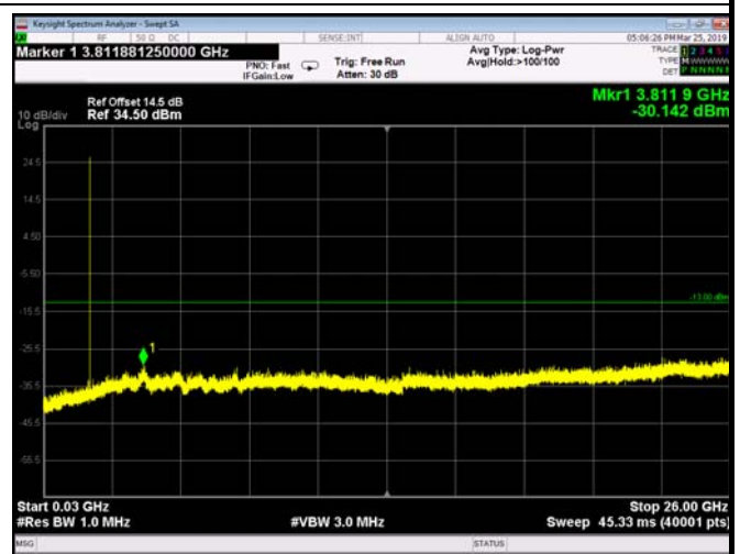
FDD66_HighRange_3MHz_30MHz~26GHz
