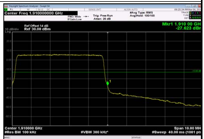
HighRange_FDD02_5MHz_1907.5_fullRB _High_Q16
