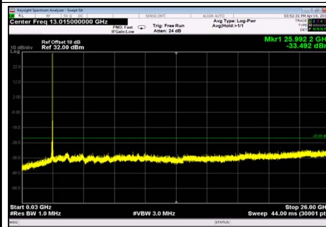
TDD41_MidRange_20MHz_30MHz~26GHz
