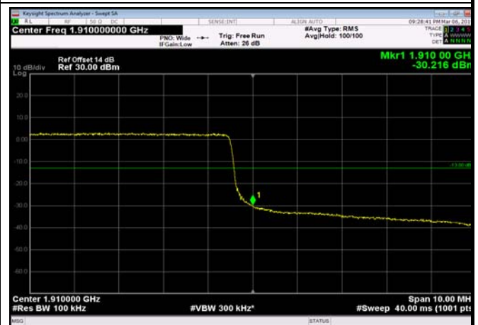
HighRange_FDD02_15MHz_1902.5_OneRB _high_Q16
