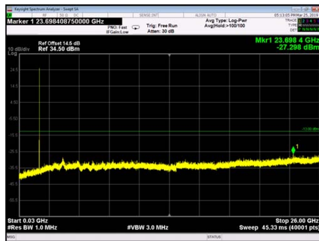
FDD26_MidRange_10MHz_30MHz~26GHz
