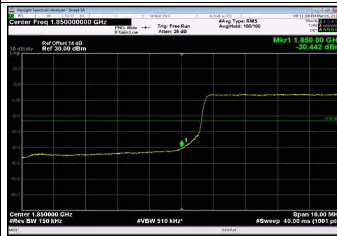
LowRange_FDD02_15MHz_1857.5_fullRB _Low_QPSK
