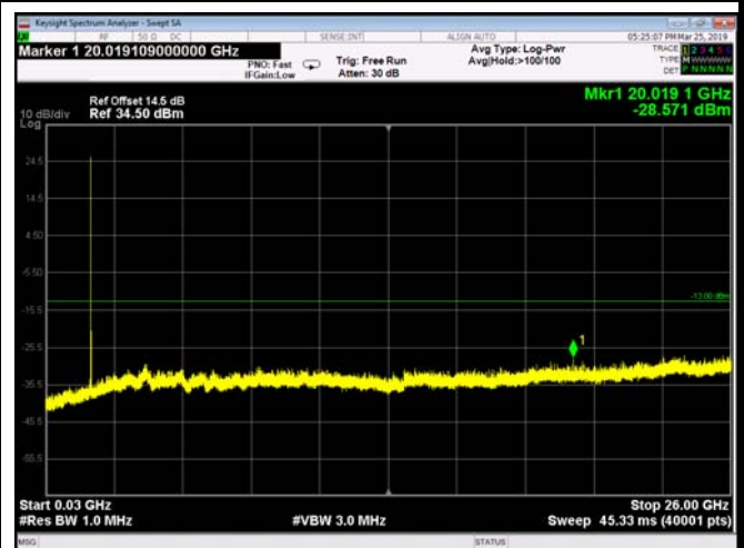
FDD26_MidRange_15MHz_30MHz~26GHz
