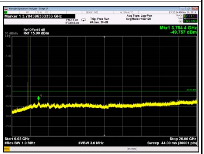
FDD30_HighRange_5MHz_30MHz~26GHz
