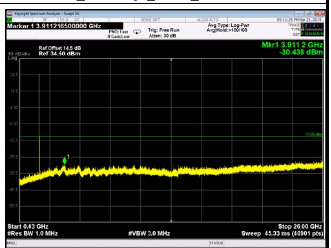
FDD26_MidRange_5MHz_30MHz~26GHz
