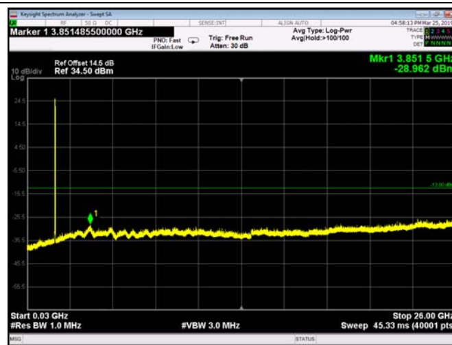
FDD26_MidRange_3MHz_30MHz~26GHz
