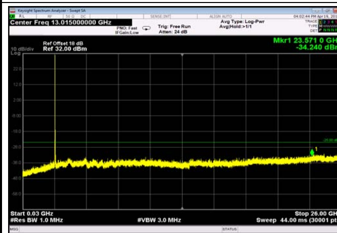
TDD41_LowRange_10MHz_30MHz~26GHz
