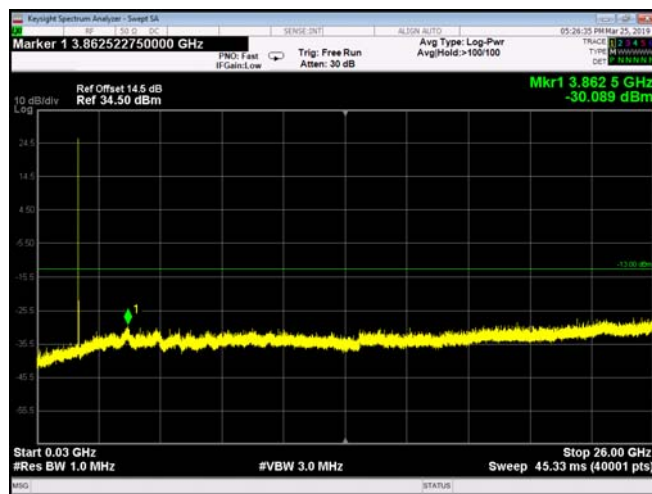
FDD66_MidRange_20MHz_30MHz~26GHz
