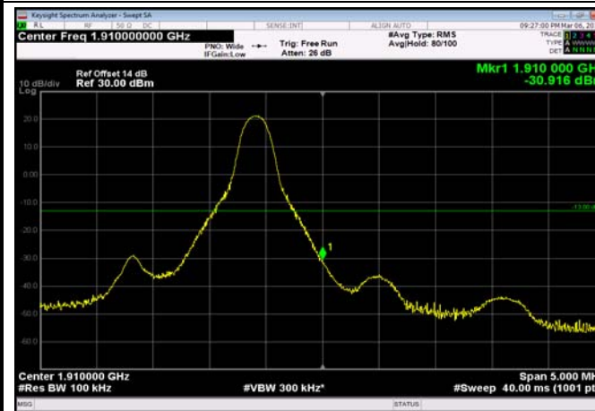
HighRange_FDD02_10MHz_1905_fullRB _High_QPSK
