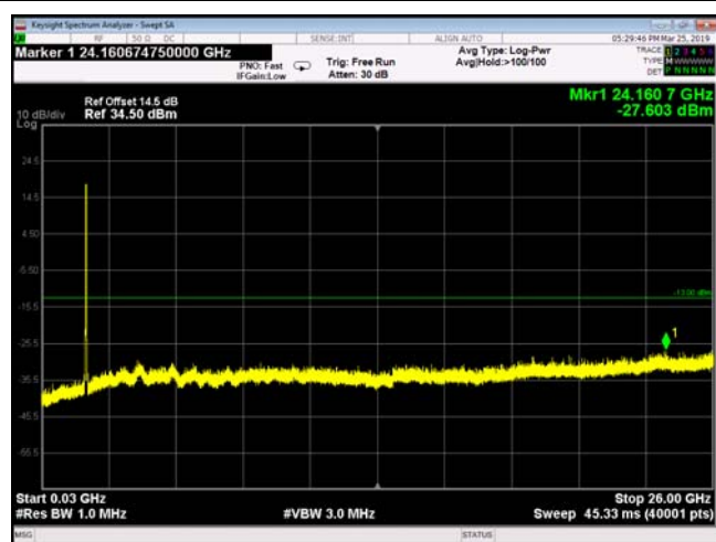
FDD66_MidRange_20MHz_30MHz~26GHz
