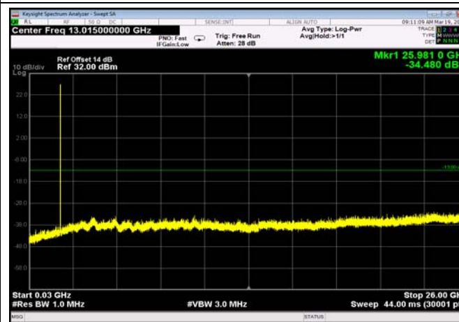
FDD25_MidRange_15MHz_30MHz~26GHz
