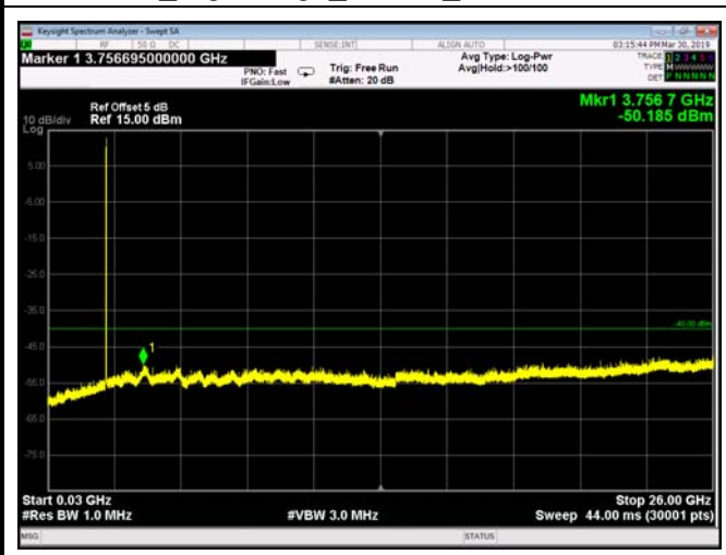
FDD30_HighRange_10MHz_30MHz~26GHz
