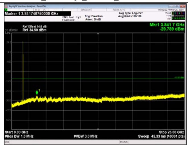
FDD26_MidRange_1.4MHz_30MHz~26GHz
