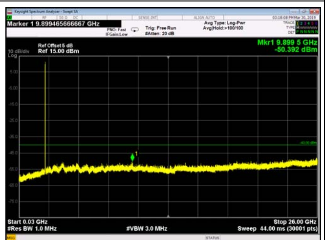
FDD30_MidRange_5MHz_30MHz~26GHz
