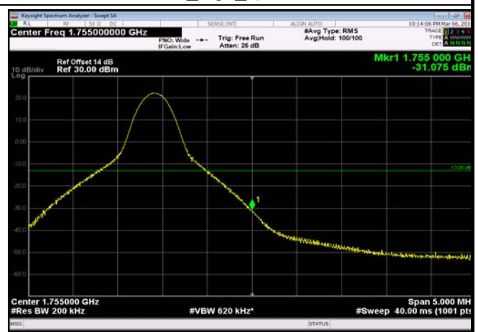
HighRange_FDD04_20MHz_1745_OneRB _high_Q16
