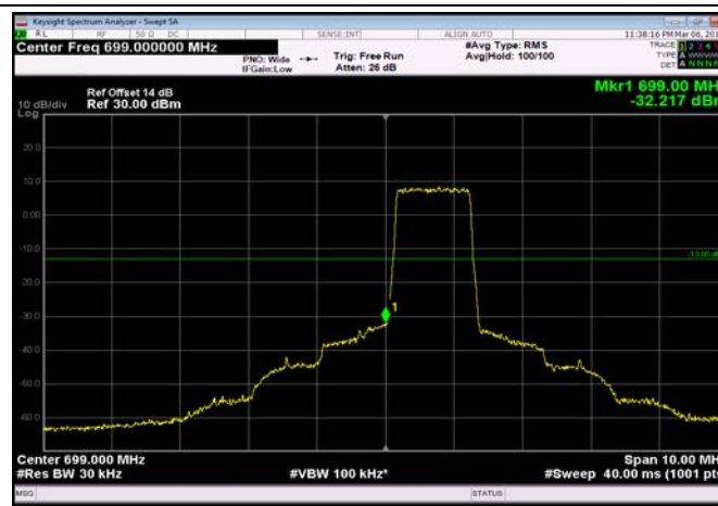
LowRange_FDD12_1.4MHz_699.7_fullRB _Low_QPSK
