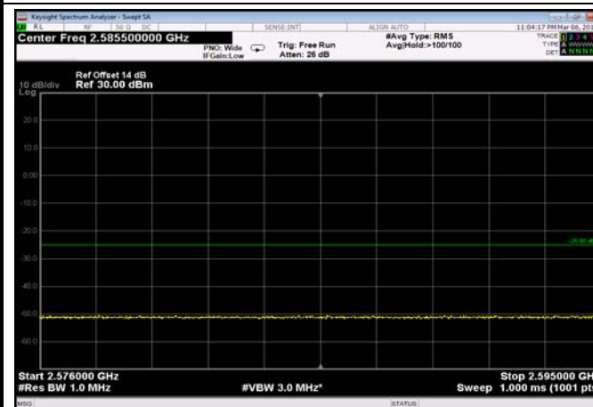
LowRange_FDD07_20MHz_2510_OneRB _low_Q16
