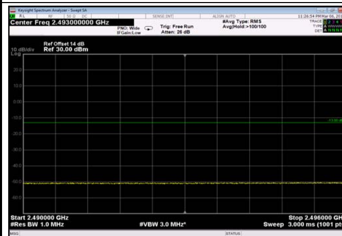
FDD07_15MHz_2562.5_QPSK_fullRB _ExtraBands_Range_2490~2496
