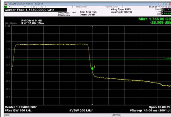
HighRange_FDD04_10MHz_1750_OneRB _high_QPSK
