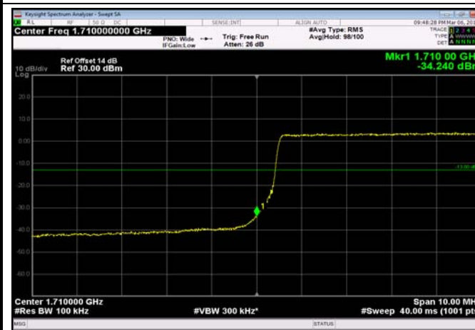
LowRange_FDD04_10MHz_1715_fullRB _Low_QPSK
