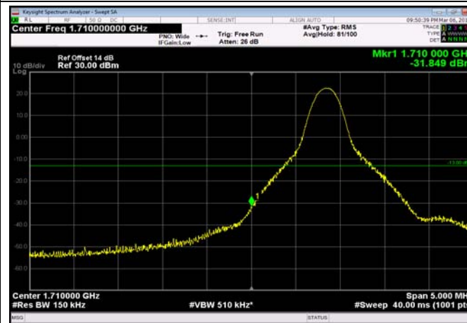
LowRange_FDD04_15MHz_1717.5_fullRB _Low_QPSK
