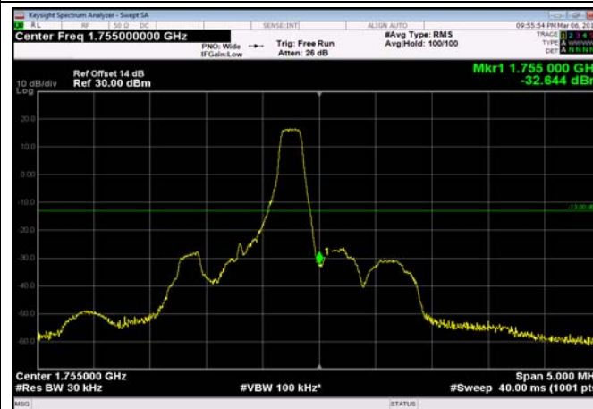
HighRange_FDD04_5MHz_1752.5_OneRB _high_QPSK
