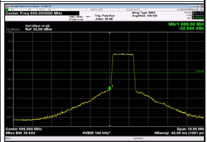
LowRange_FDD12_1.4MHz_699.7_fullRB _Low_Q16
