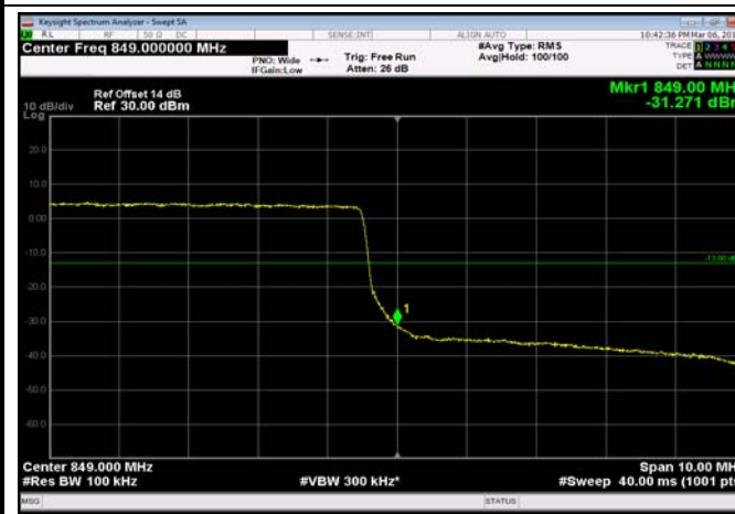
HighRange_FDD05_10MHz_844_fullRB _High_QPSK
