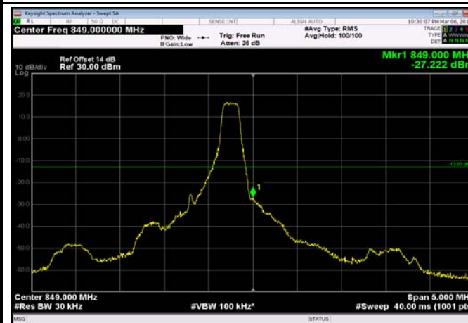
HighRange_FDD05_5MHz_846.5_OneRB _high_QPSK
