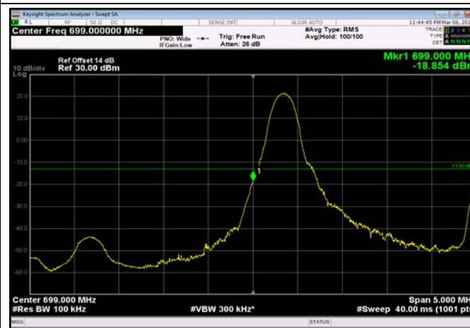
LowRange_FDD12_5MHz_701.5_OneRB _low_QPSK
