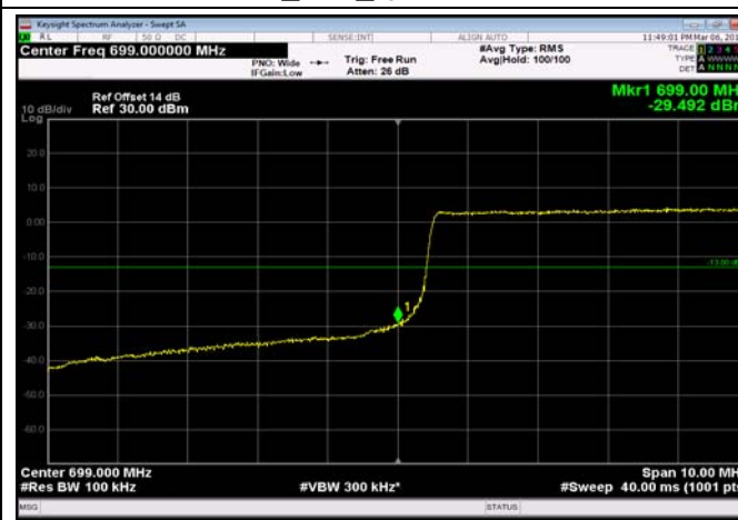
LowRange_FDD12_10MHz_704_fullRB _Low_QPSK
