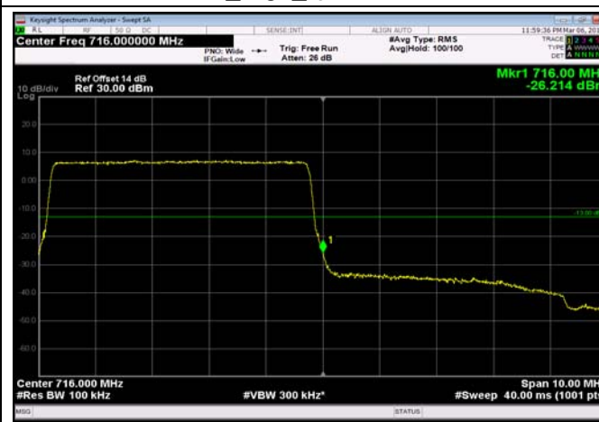
HighRange_FDD12_5MHz_713.5_fullRB _High_QPSK
