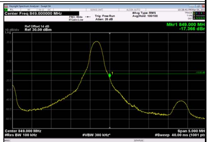
HighRange_FDD05_5MHz_846.5_OneRB _high_Q16
