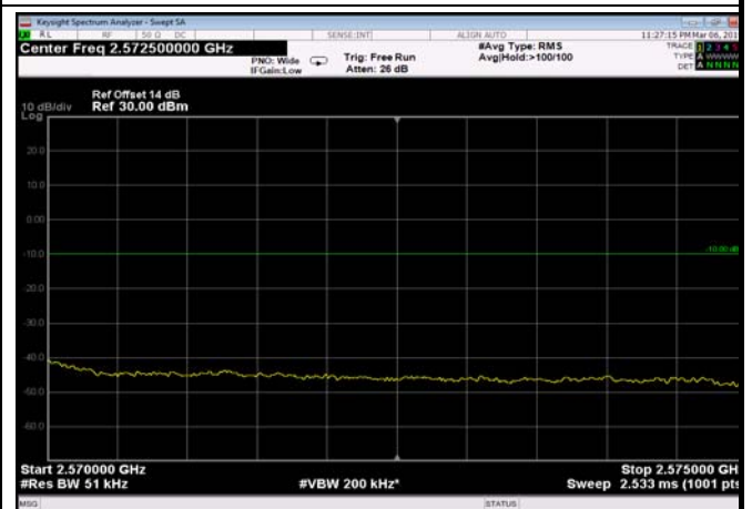
FDD07_15MHz_2562.5_QPSK_fullRB _ExtraBands_Range_2570~2575
