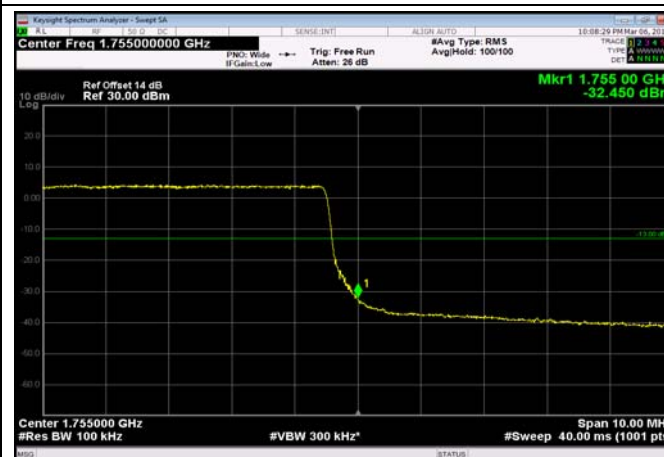
HighRange_FDD04_10MHz_1750_fullRB _High_QPSK
