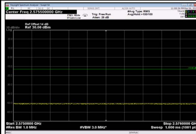
HighRange_FDD07_5MHz_2567.5_OneRB _high_QPSK
