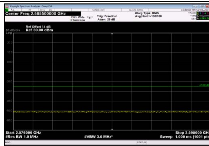
FDD07_10MHz_2505_QPSK_OneRB_high ExtraBands_Range_2576~2595
