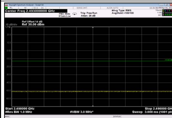
HighRange_FDD07_20MHz_2560_fullIRB _High_Q16
