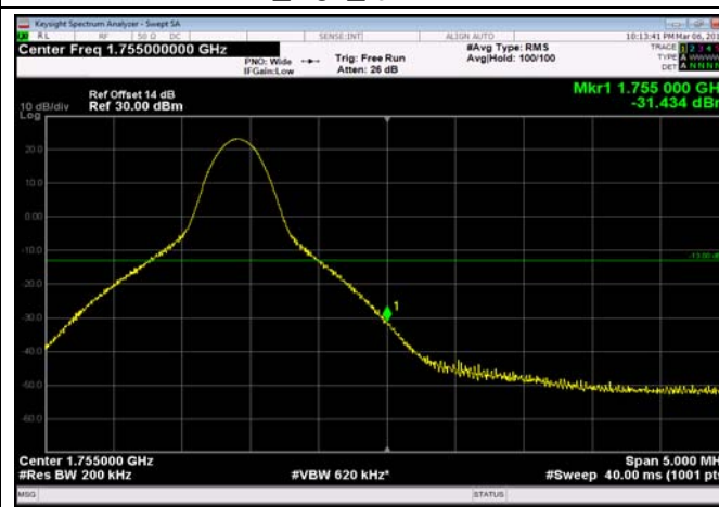
HighRange_FDD04_20MHz_1745_OneRB _high_QPSK
