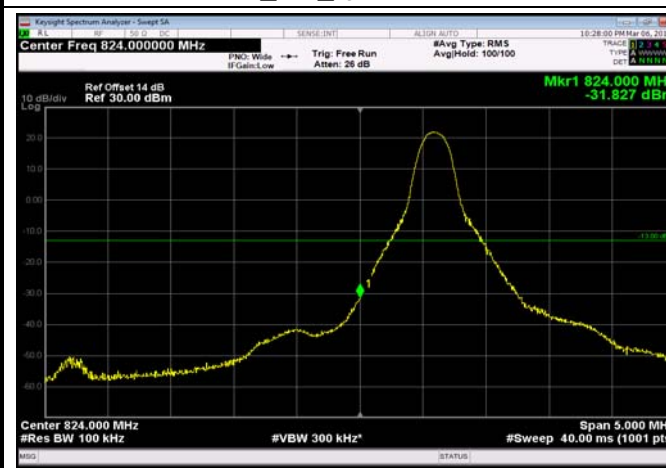
LowRange_FDD05_10MHz_829_OneRB _low_QPSK
