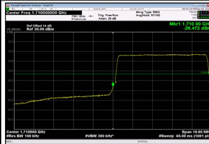
LowRange_FDD04_10MHz_1715_OneRB _low_QPSK
