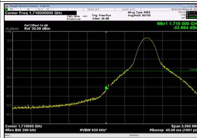
LowRange_FDD04_20MHz_1720_OneRB _low_QPSK
