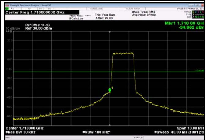
LowRange_FDD04_3MHz_1711.5_OneRB _low_Q16
