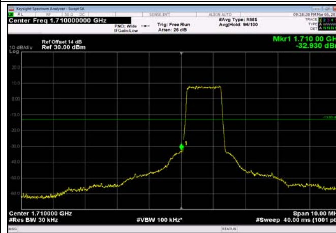
LowRange_FDD04_3MHz_1711.5_OneRB _low_QPSK
