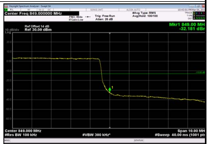
HighRange_FDD05_10MHz_844_fullRB _High_Q16
