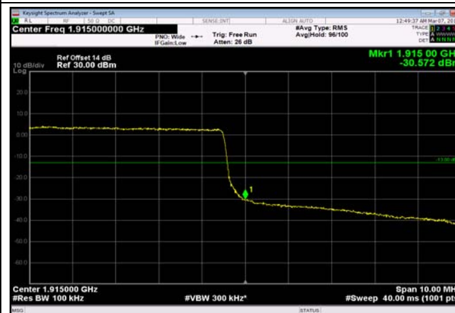
HighRange_FDD25_15MHz_1907.5_OneRB _high_QPSK
