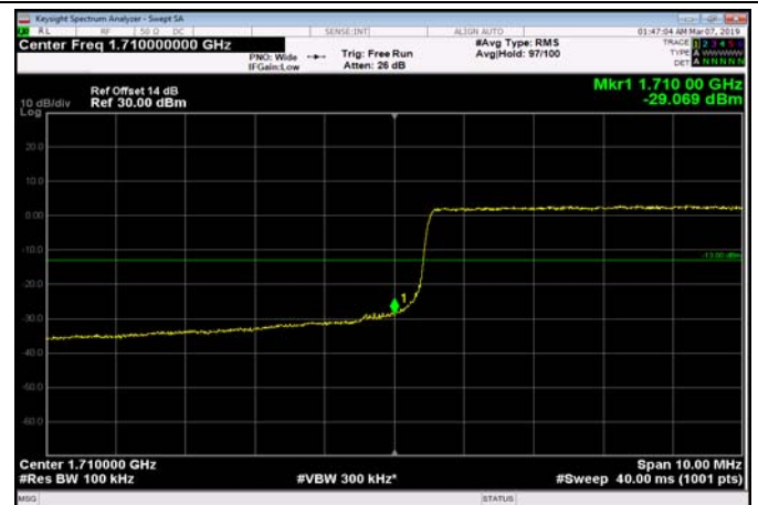
LowRange_FDD66_15MHz_1717.5_OneRB _low_Q16
