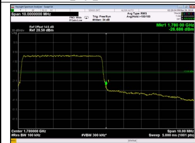
HighRange_FDD66_5MHz_1777.5_fullRB _High_QPSK252
