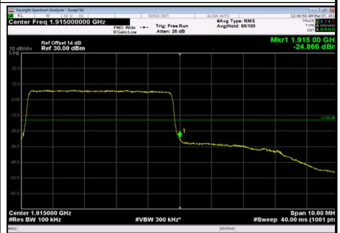
HighRange_FDD25_5MHz_1912.5_fullRB _High_Q16
