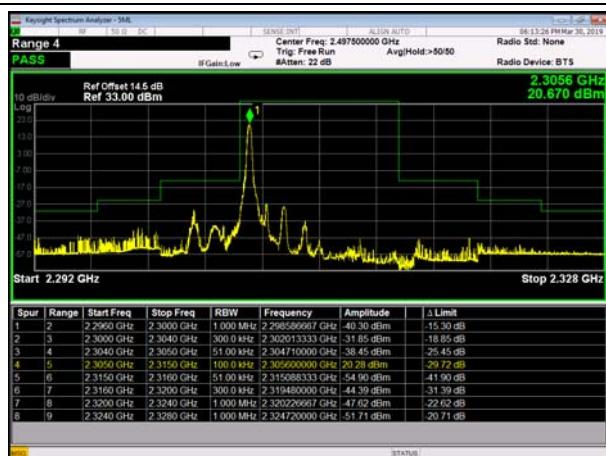
LowRange_FDD30_10MHz_2310_OneRB _low_QPSK
