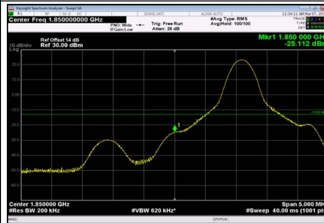
LowRange_FDD25_20MHz_1860_fullRB _Low_QPSK
