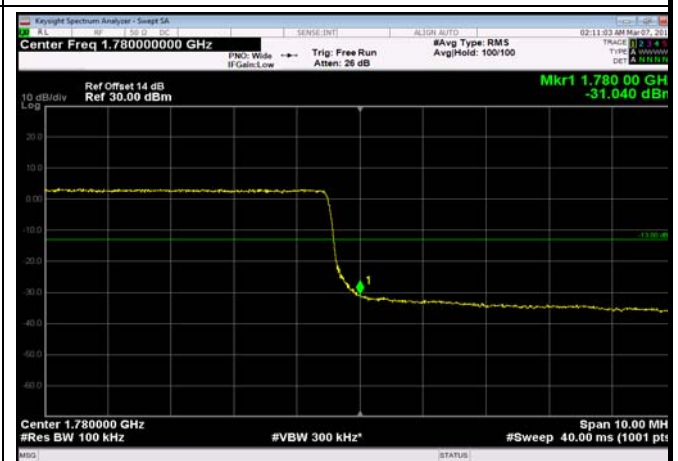
HighRange_FDD66_15MHz_1772.5_OneRB _high_Q16
