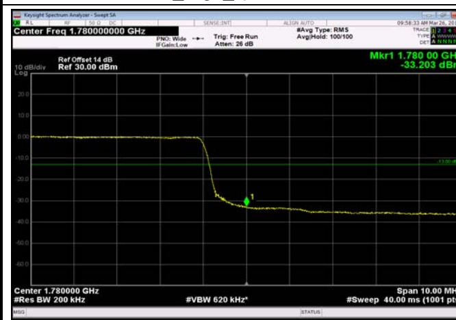
HighRange_FDD66_20MHz_1770_fullRB _High_QPSK
