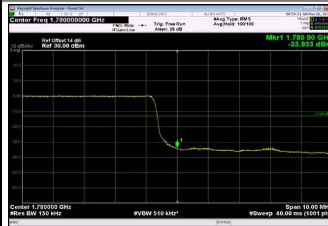
HighRange_FDD66_20MHz_1770_OneRB _high_QPSK
