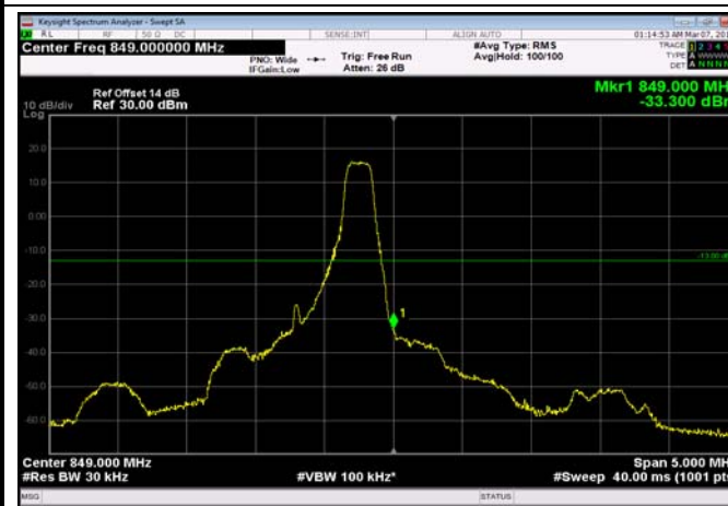
HighRange_FDD26_1.4MHz_848.3_OneRB _high_QPSK
