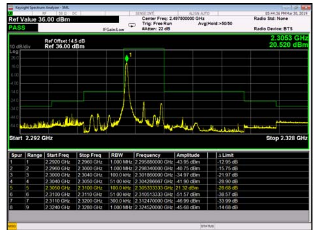
LowRange_FDD30_5MHz_2307.5_fullRB _Low_Q16
