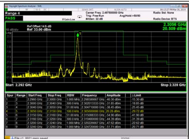
LowRange_FDD30_10MHz_2310_OneRB _low_Q16
