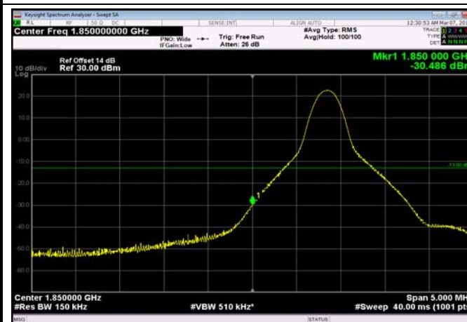
LowRange_FDD25_15MHz_1857.5_fullRB _Low_QPSK
