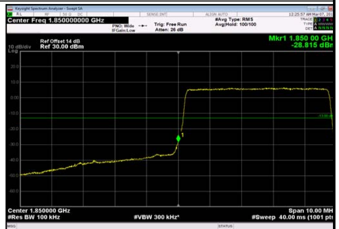
LowRange_FDD25_10MHz_1855_OneRB _low_Q16
