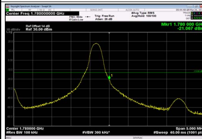
HighRange_FDD66_5MHz_1777.5_fullRB _High_QPSK252
