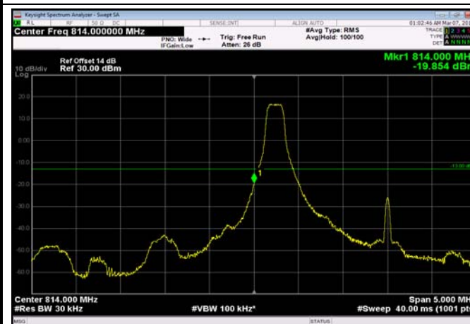
LowRange_FDD26_5MHz_816.5_OneRB _low_QPSK
