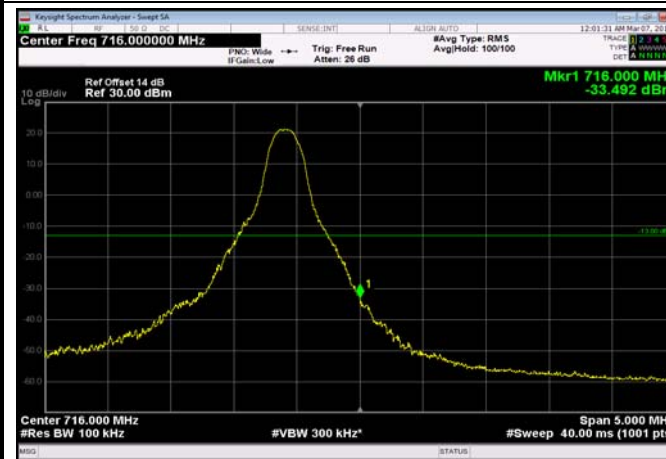
HighRange_FDD12_10MHz_711_fullRB _High_QPSK
