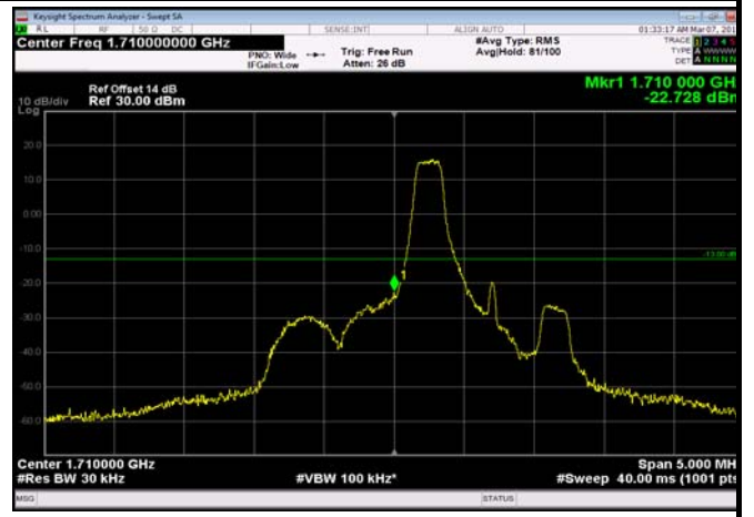
LowRange_FDD66_1.4MHz_1710.7_OneRB _low_Q16
