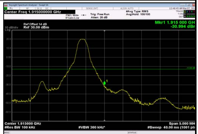
HighRange_FDD25_10MHz_1910_fullRB _High_Q16
