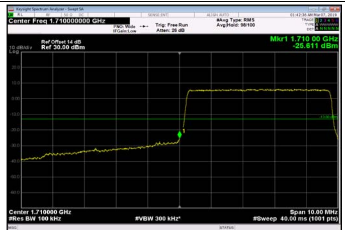
LowRange_FDD66_5MHz_1712.5_fullRB _Low_Q16
