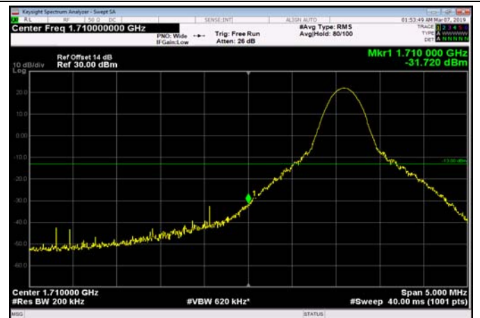
LowRange_FDD66_20MHz_1720_fullRB _Low_Q16
