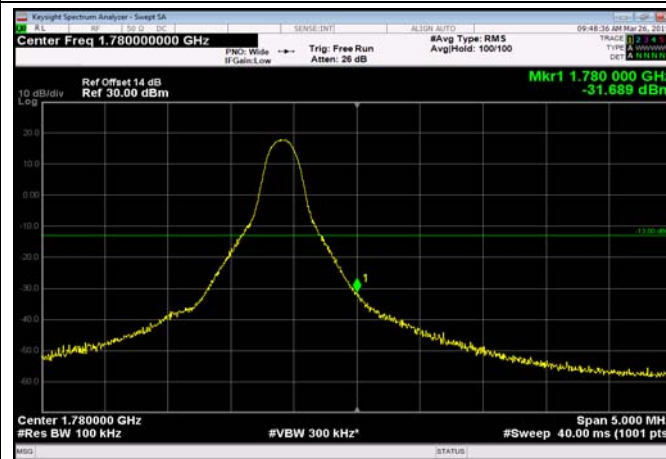
HighRange_FDD66_10MHz_1775_fullRB _High_QPSK 253
