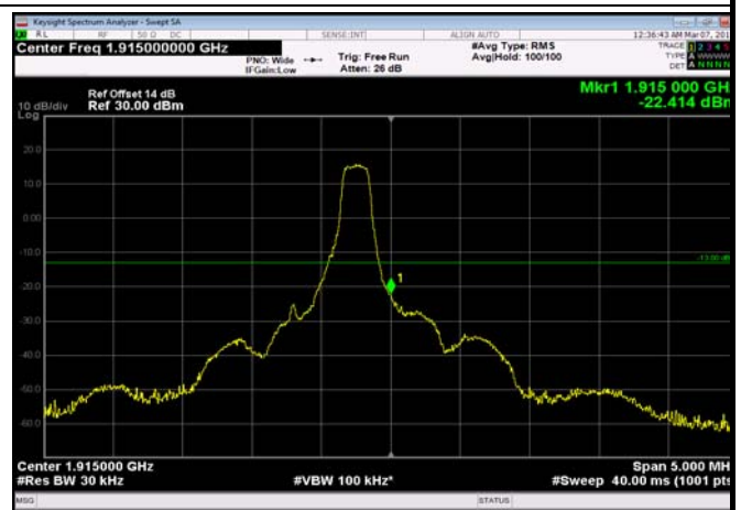
HighRange_FDD25_1.4MHz_1914.3_OneRB _high_Q16
