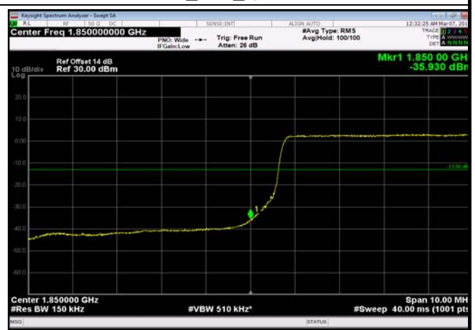
LowRange_FDD25_15MHz_1857.5_fullRB _Low_Q16
