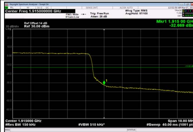
HighRange_FDD25_20MHz_1905_OneRB _high_QPSK
