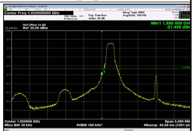
LowRange_FDD25_3MHz_1851.5_OneRB _low_Q16
