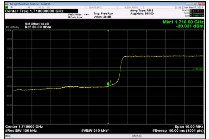
LowRange_FDD66_20MHz_1720_OneRB _low_Q16
