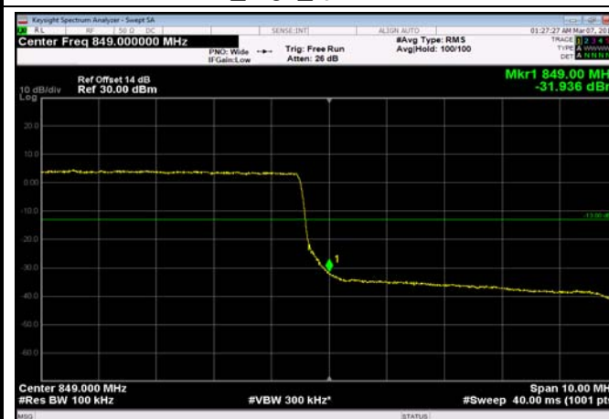
HighRange_FDD26_10MHz_844_fullRB _High_QPSK
