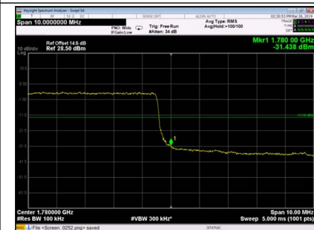
HighRange_FDD66_15MHz_1772.5_OneRB _high_QPSK 255
