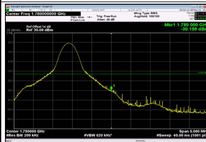
HighRange_FDD66_20MHz_1770_fullRB _High_QPSK
