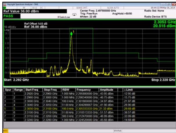
LowRange_FDD30_5MHz_2307.5_fullRB _Low_QPSK
