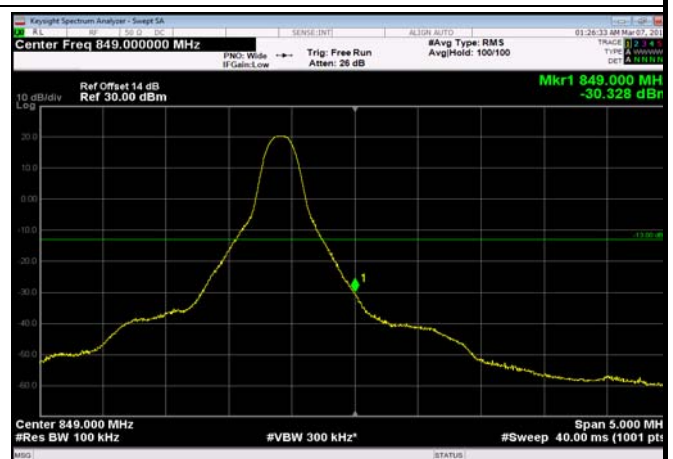
HighRange_FDD26_10MHz_844_fullRB _High_Q16
