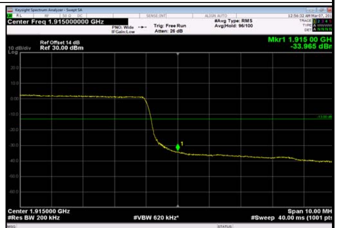
HighRange_FDD25_20MHz_1905_fullRB _High_Q16
