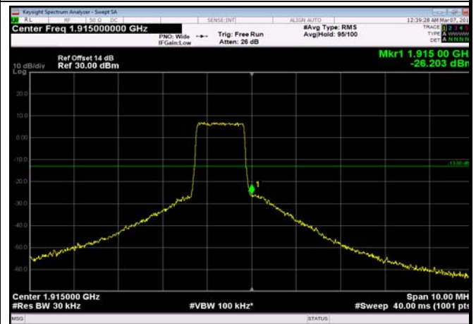
HighRange_FDD25_5MHz_1912.5_OneRB _high_Q16
