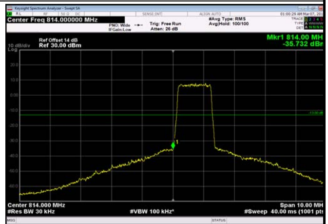
LowRange_FDD26_3MHz_815.5_OneRB _low_Q16
