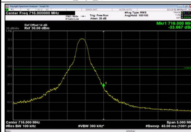
HighRange_FDD17_10MHz_711_OneRB _high_QPSK
