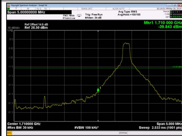
LowRange_FDD66_15MHz_1717.5_OneRB _low_QPSK 244
