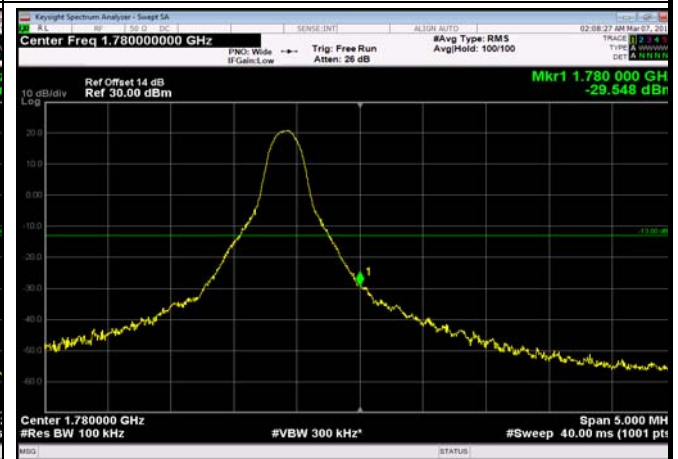
HighRange_FDD66_10MHz_1775_fullRB _High_Q16
