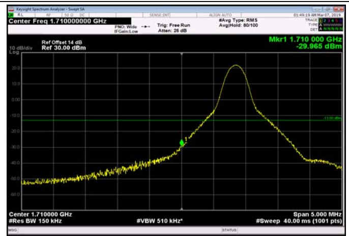
LowRange_FDD66_15MHz_1717.5_OneRB _low_Q16
