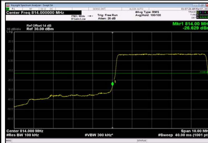
LowRange_FDD26_10MHz_820_OneRB _low_QPSK
