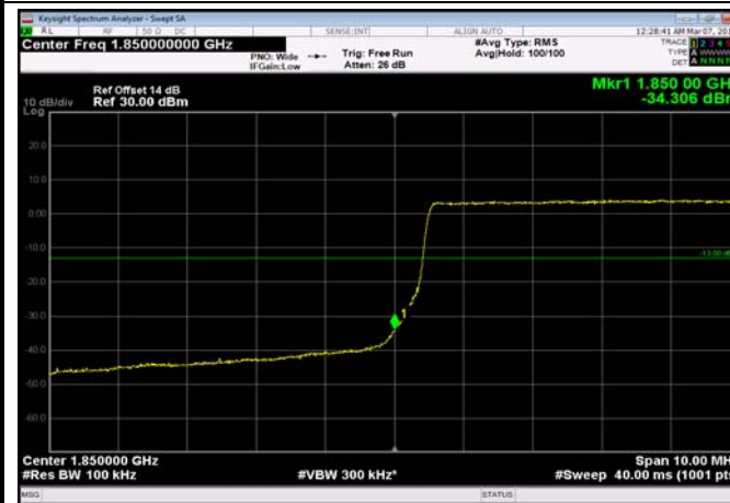
LowRange_FDD25_15MHz_1857.5_OneRB _low_QPSK
