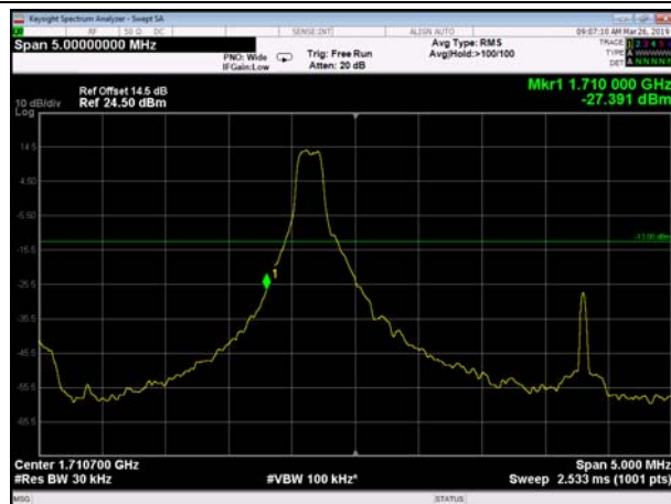
LowRange_FDD66_5MHz_1712.5_fullRB _Low_QPSK 241
