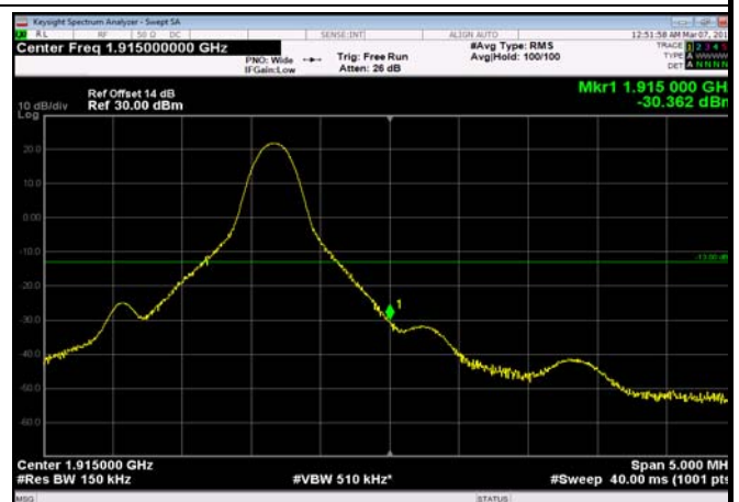
HighRange_FDD25_15MHz_1907.5_OneRB _high_Q16
