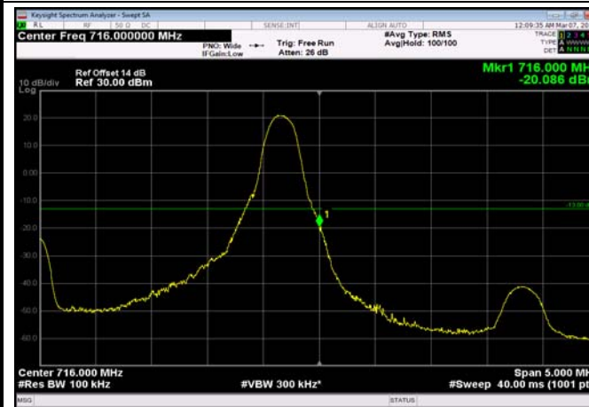
HighRange_FDD17_5MHz_713.5_fullRB _High_QPSK
