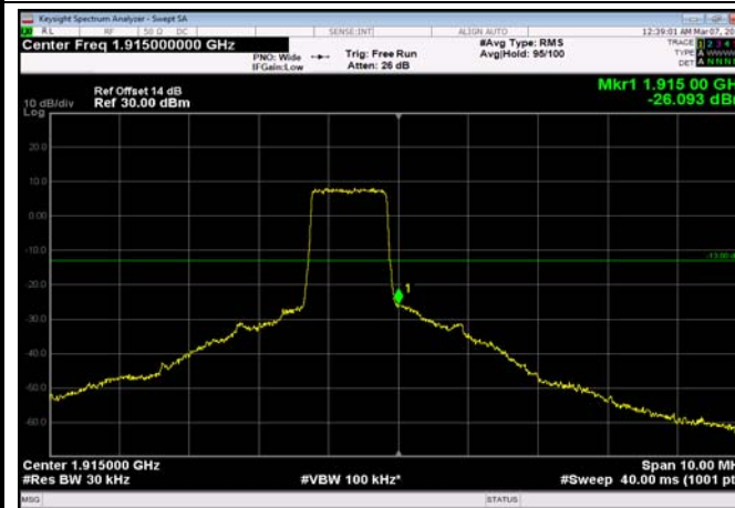
HighRange_FDD25_5MHz_1912.5_OneRB _high_QPSK
