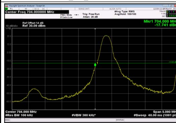
LowRange_FDD17_5MHz_706.5_OneRB _low_QPSK
