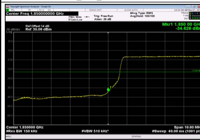
LowRange_FDD25_15MHz_1857.5_fullRB _Low_QPSK
