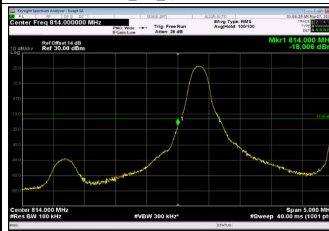
LowRange_FDD26_5MHz_816.5_OneRB _low_QPSK
