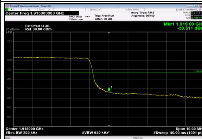
HighRange_FDD25_20MHz_1905_fullRB _High_QPSK
