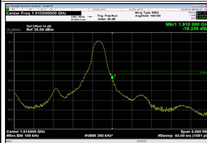
HighRange_FDD25_5MHz_1912.5_fullRB _High_QPSK
