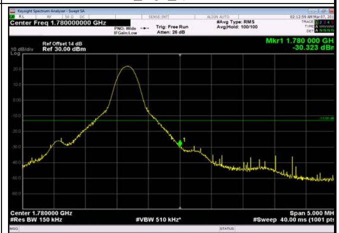
HighRange_FDD66_15MHz_1772.5_OneRB _high_Q16
