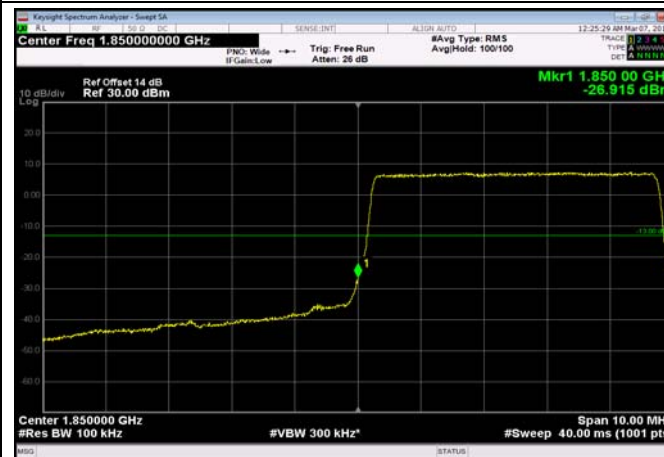
LowRange_FDD25_10MHz_1855_OneRB _low_QPSK
