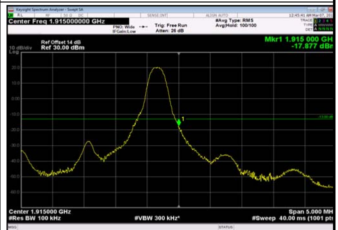
HighRange_FDD25_5MHz_1912.5_fullRB _High_Q16
