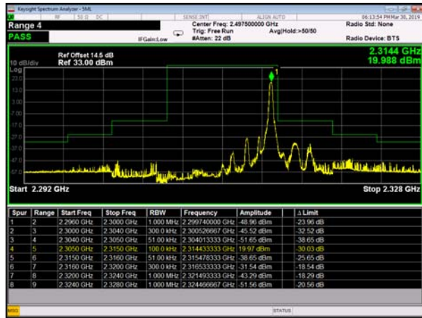
HighRange_FDD30_10MHz_2310_fullRB _High_QPSK
