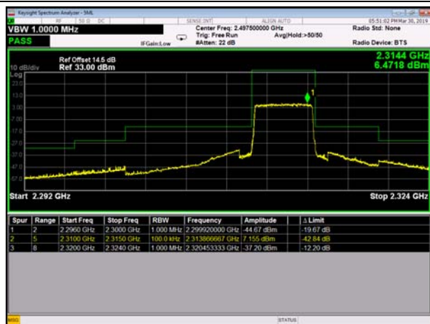
HighRange_FDD30_5MHz_2312.5_fullRB _High_QPSK
