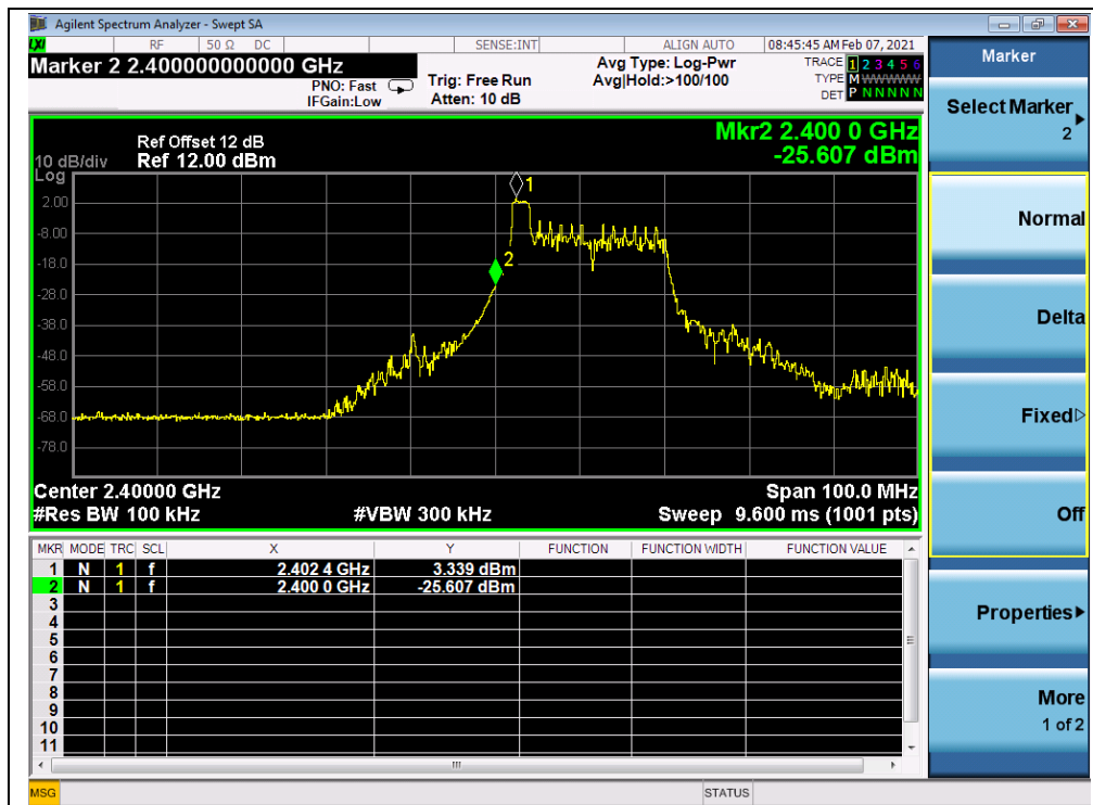
(Band Edge, Channel 1, 802.11ax (HEW20)(RU26))
