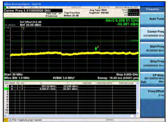
Band19 / 15MHz / High CH / 16QAM
