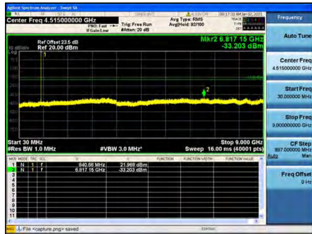
Band19 / 5MHz / High CH / 64QAM
