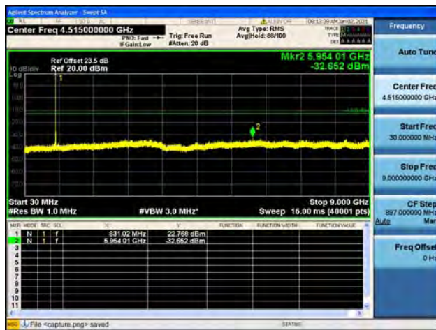
Band19 / 15MHz / High CH / 64QAM
