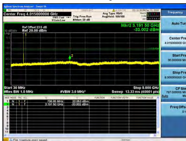
Band12 / 10MHz / High CH / 64QAM
