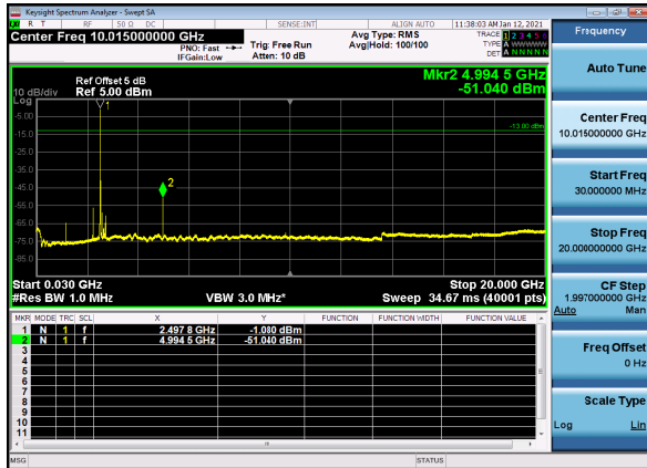
N41(40M)_DFT-s-OFDM_BPSK_Edge_1RB_Low_CH
