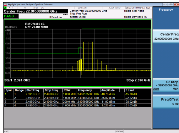
N41(20M)_DFT-s-OFDM_BPSK_Edge_1RB_High_CH
