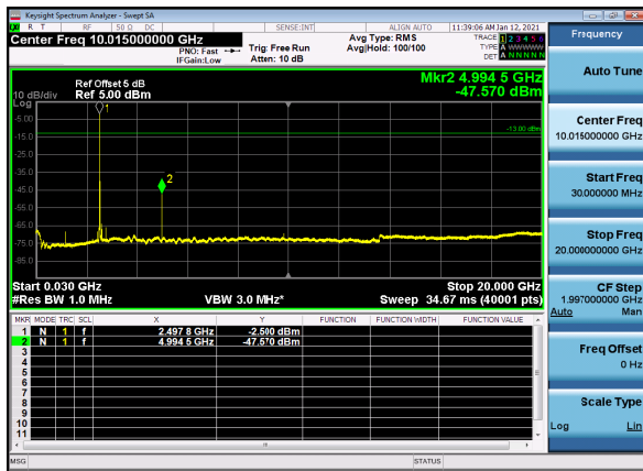
N41(40M)_DFT-s-OFDM_QPSK_Edge_1RB_Low_CH
