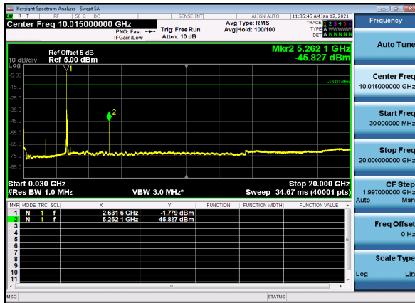
N41(60M)_DFT-s-OFDM_BPSK_Edge_1RB_High_CH
