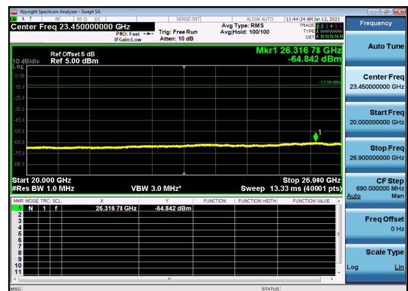
N41(40M)_DFT-s-OFDM_QPSK_Edge_1RB_High_CH
