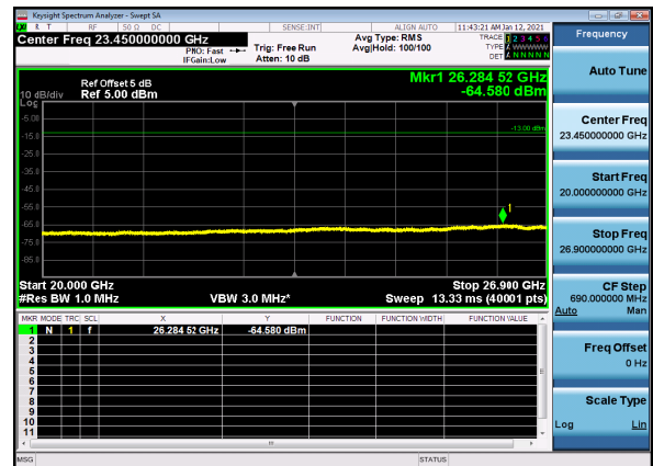
N41(40M)_DFT-s-OFDM_BPSK_Edge_1RB_High_CH
