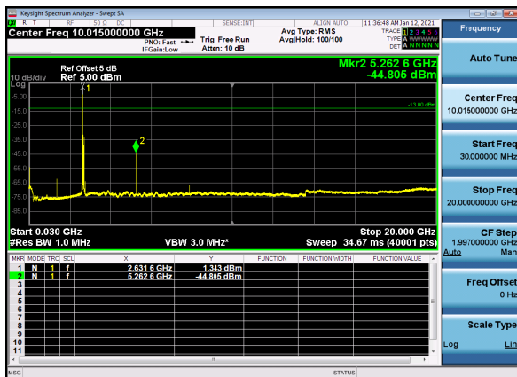
N41(60M)_DFT-s-OFDM_QPSK_Edge_1RB_High_CH
