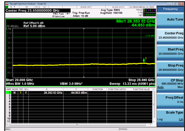
N41(40M)_DFT-s-OFDM_QPSK_Edge_1RB_Left_Low_CH
