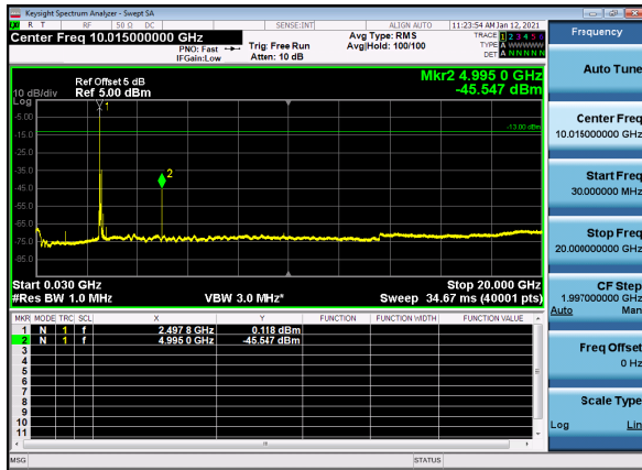
N41(80M)_DFT-s-OFDM_BPSK_Edge_1RB_Low_CH
