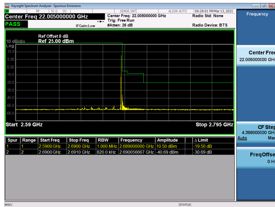
N41(40M)_DFT-s-OFDM_BPSK_Outer_Full_High_CH
