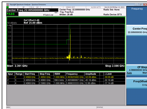
N41(40M)_DFT-s-OFDM_BPSK_Outer_Full_Low_CH
