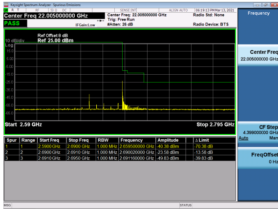
N41(60M)_DFT-s-OFDM_BPSK_Outer_Full_High_CH
