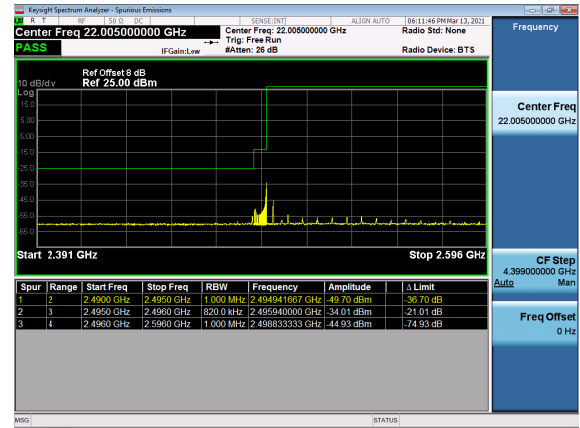
N41(80M)_DFT-s-OFDM_QPSK_Outer_Full_Low_CH
