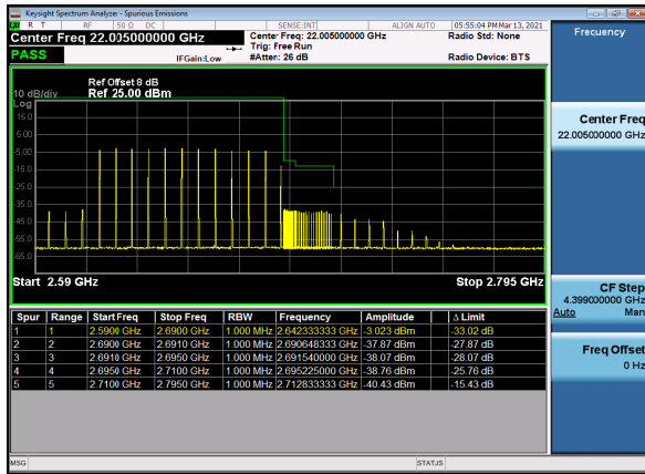
N41(60M)_DFT-s-OFDM_BPSK_Edge_1RB_Low_CH
