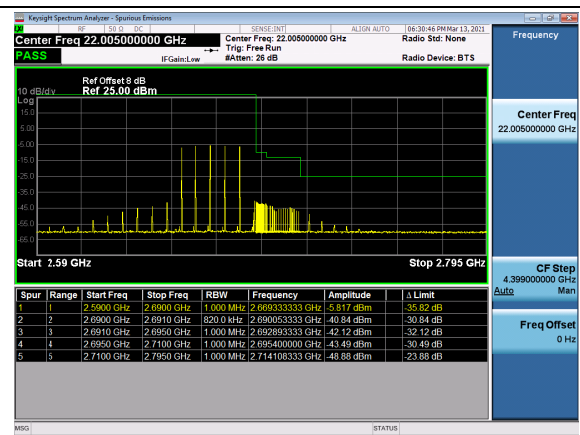
N41(20M)_DFT-s-OFDM_QPSK_Edge_1RB_Low_CH
