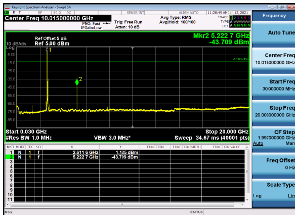
N41(80M)_DFT-s-OFDM_BPSK_Edge_1RB_High_CH
