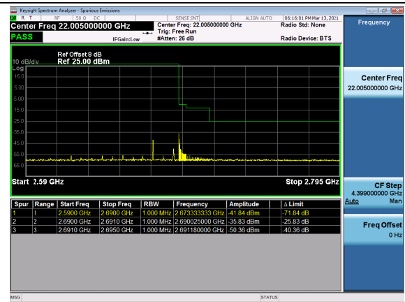
N41(80M)_DFT-s-OFDM_QPSK_Outer_Full_High_CH
