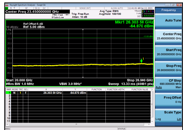
N41(40M)_DFT-s-OFDM_BPSK_Edge_1RB_Mid_CH
