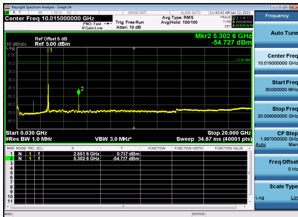
N41(40M)_DFT-s-OFDM_BPSK_Edge_1RB_High_CH
