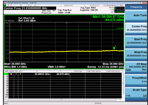
N41(60M)_DFT-s-OFDM_QPSK_Edge_1RB_Mid_CH
