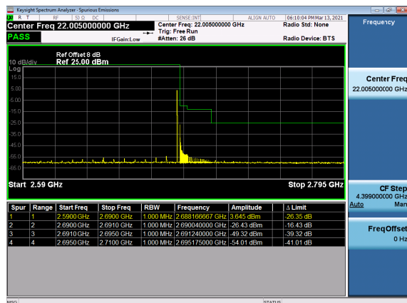
N41(100M)_DFT-s-OFDM_BPSK_Outer_Full_ High_CH
