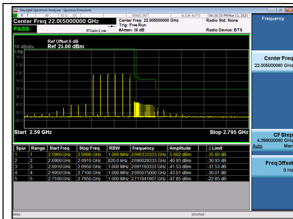
N41(20M)_DFT-s-OFDM_BPSK_Edge_1RB_Low_CH
