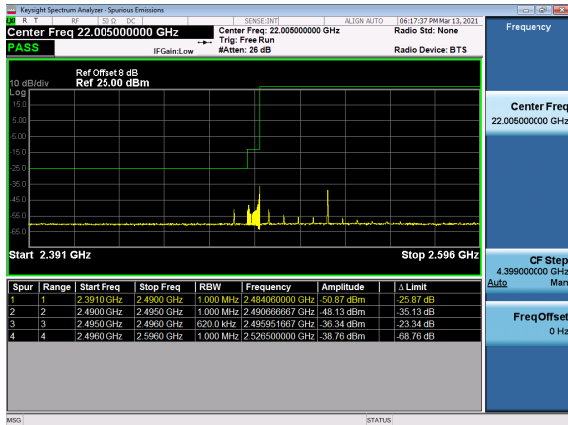
N41(60M)_DFT-s-OFDM_BPSK_Outer_Full_Low_CH
