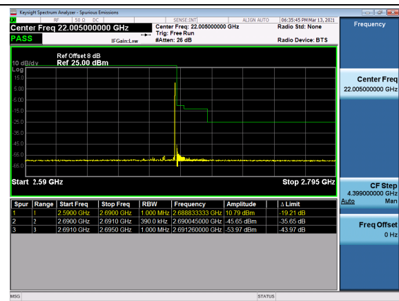
N41(20M)_DFT-s-OFDM_QPSK_Outer_Full_High_CH
