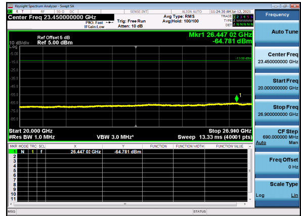
N41(80M)_DFT-s-OFDM_BPSK_Edge_1RB_Low_CH
