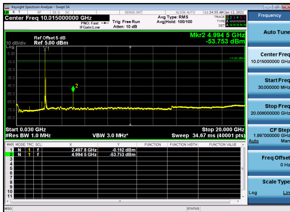
N41(80M)_DFT-s-OFDM_QPSK_Edge_1RB_Low_CH
