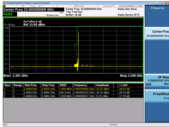
N41(20M)_DFT-s-OFDM_BPSK_Outer_Full_Low_CH
