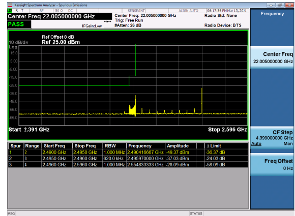
N41(60M)_DFT-s-OFDM_QPSK_Outer_Full_Low_CH
