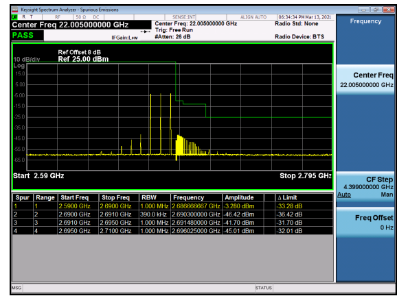
N41(20M)_DFT-s-OFDM_QPSK_Outer_Full_High_CH
