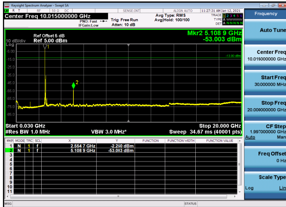
N41(80M)_DFT-s-OFDM_QPSK_Edge_1RB_Mid_CH
