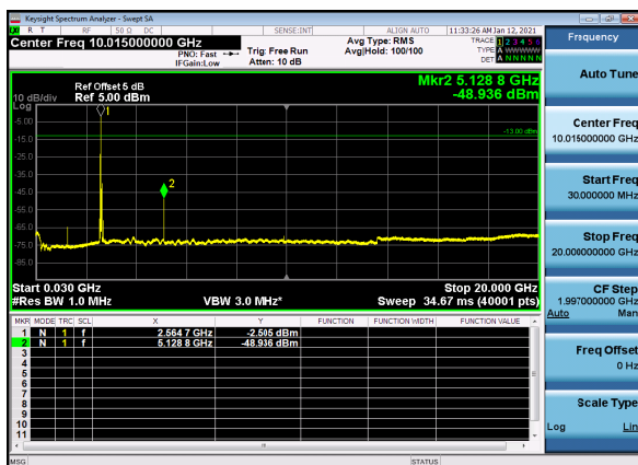
N41(60M)_DFT-s-OFDM_BPSK_Edge_1RB_Left_Mid_CH
