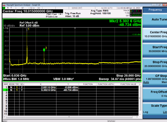
N41(40M)_DFT-s-OFDM_QPSK_Edge_1RB_High_CH
