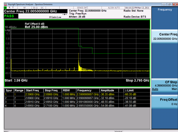
N41(100M)_DFT-s-OFDM_QPSK_Outer_Full_ High_CH
