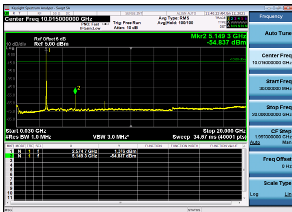
N41(40M)_DFT-s-OFDM_BPSK_Edge_1RB_Mid_CH
