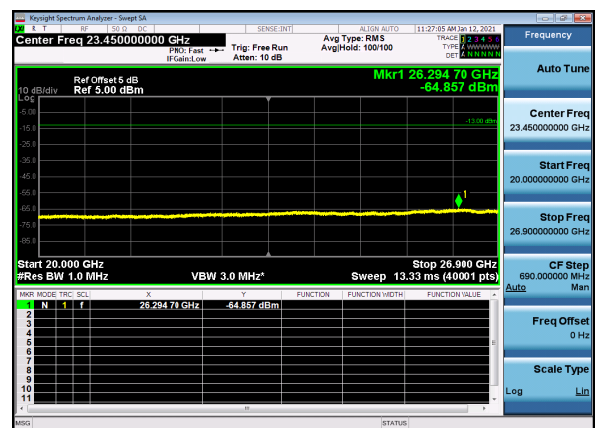
N41(80M)_DFT-s-OFDM_BPSK_Edge_1RB_Mid_CH
