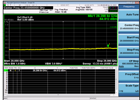
N41(80M)_DFT-s-OFDM_QPSK_Edge_1RB_Mid_CH
