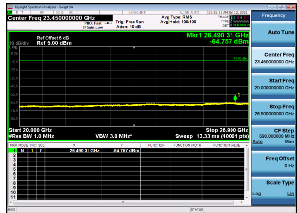
N41(80M)_DFT-s-OFDM_QPSK_Edge_1RB_Low_CH
