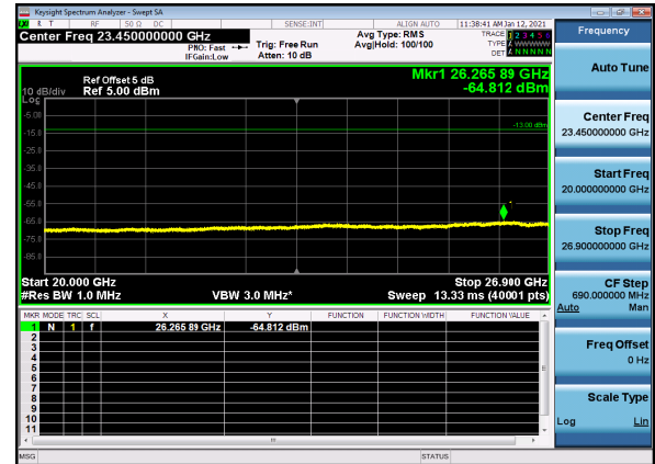
N41(40M)_DFT-s-OFDM_BPSK_Edge_1RB_Low_CH
