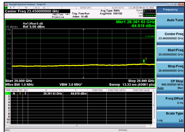
N41(80M)_DFT-s-OFDM_BPSK_Edge_1RB_High_CH
