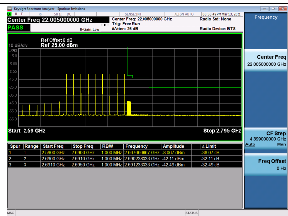
N41(60M)_DFT-s-OFDM_QPSK_Edge_1RB_High_CH
