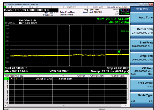
N41(80M)_DFT-s-OFDM_QPSK_Edge_1RB_High_CH
