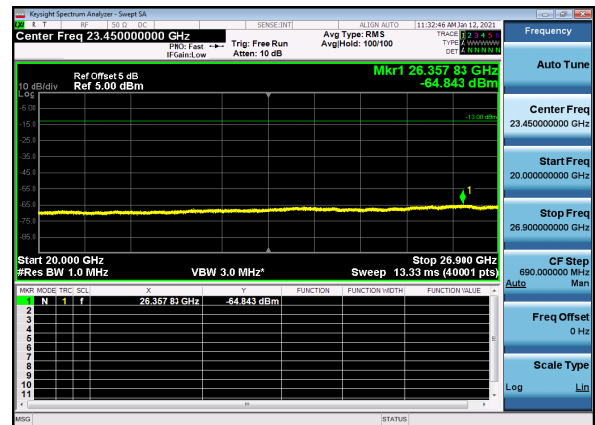
N41(60M)_DFT-s-OFDM_QPSK_Edge_1RB_Low_CH
