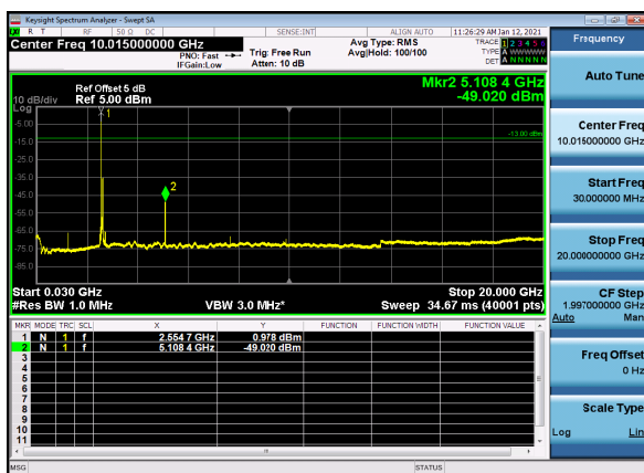
N41(80M)_DFT-s-OFDM_BPSK_Edge_1RB_Left_Mid_CH
