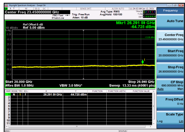
N41(60M)_DFT-s-OFDM_BPSK_Edge_1RB_Mid_CH
