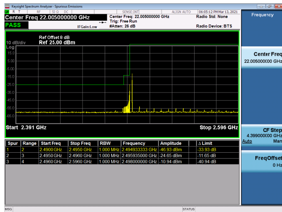
N41(100M)_DFT-s-OFDM_BPSK_Outer_Full_ Low_CH
