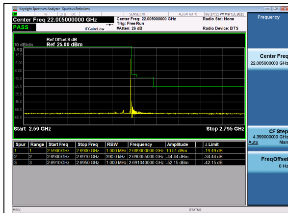
N41(20M)_DFT-s-OFDM_BPSK_Outer_Full_High_CH
