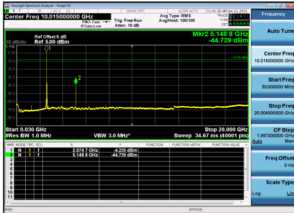
N41(40M)_DFT-s-OFDM_QPSK_Edge_1RB_Mid_CH
