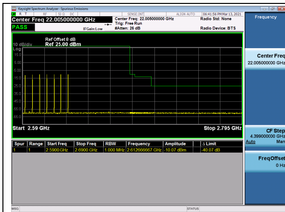
N41(80M)_DFT-s-OFDM_BPSK_Edge_1RB_Low_CH
