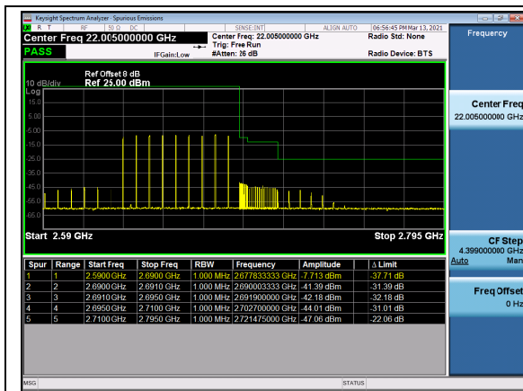
N41(60M)_DFT-s-OFDM_BPSK_Edge_1RB_High_CH
