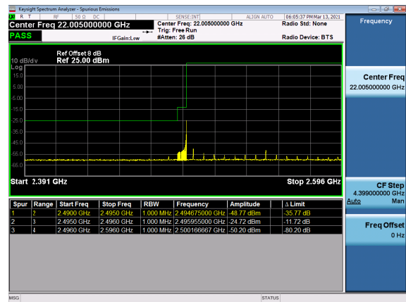
N41(100M)_DFT-s-OFDM_QPSK_Outer_Full_ Low_CH
