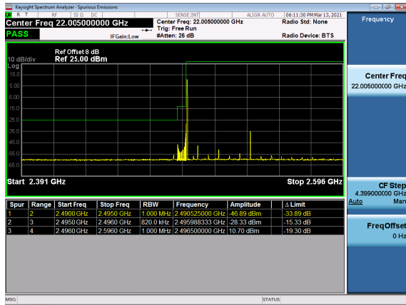
N41(80M)_DFT-s-OFDM_BPSK_Outer_Full_Low_CH
