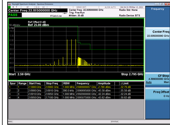
N41(20M)_DFT-s-OFDM_BPSK_Outer_Full_High_CH
