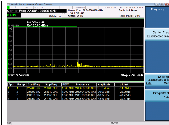
N41(80M)_DFT-s-OFDM_BPSK_Outer_Full_High_CH
