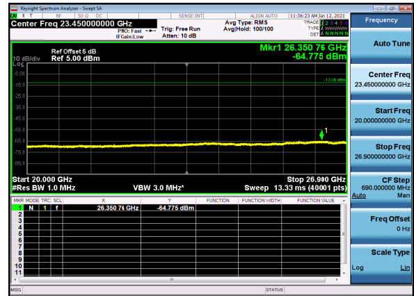
N41(60M)_DFT-s-OFDM_BPSK_Edge_1RB_High_CH
