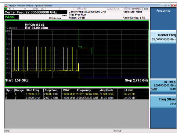
N41(80M)_DFT-s-OFDM_QPSK_Edge_1RB_Low_CH
