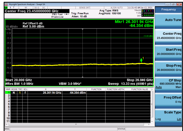
N41(60M)_DFT-s-OFDM_BPSK_Edge_1RB_Low_CH
