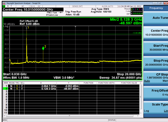
N41(60M)_DFT-s-OFDM_QPSK_Edge_1RB_Mid_CH
