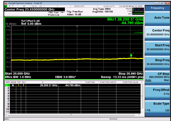
N41(40M)_DFT-s-OFDM_QPSK_Edge_1RB_Mid_CH
