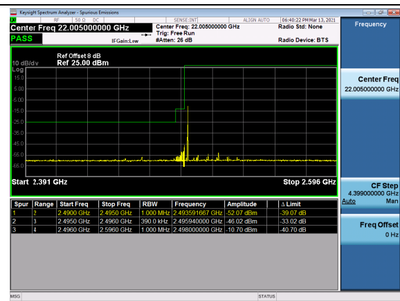
N41(40M)_DFT-s-OFDM_QPSK_Outer_Full_Low_CH
