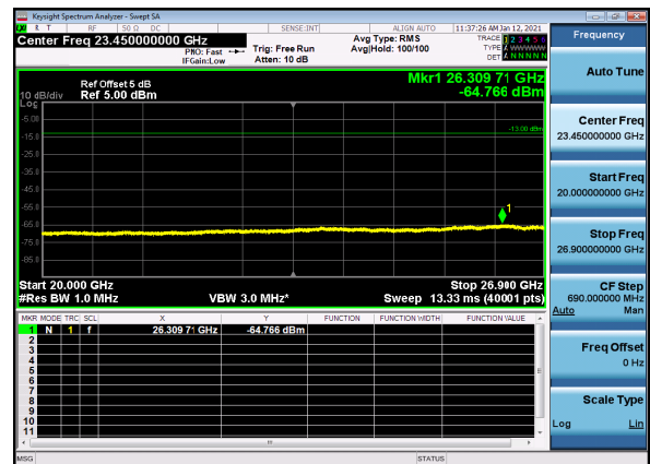
N41(60M)_DFT-s-OFDM_QPSK_Edge_1RB_High_CH
