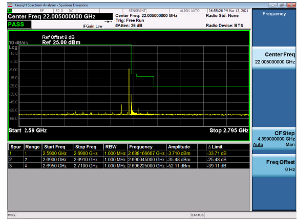
N41(60M)_DFT-s-OFDM_QPSK_Outer_Full_High_CH
