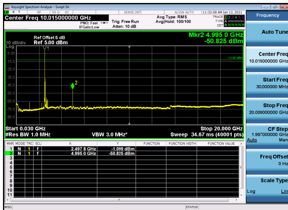
N41(60M)_DFT-s-OFDM_QPSK_Edge_1RB_Low_CH
