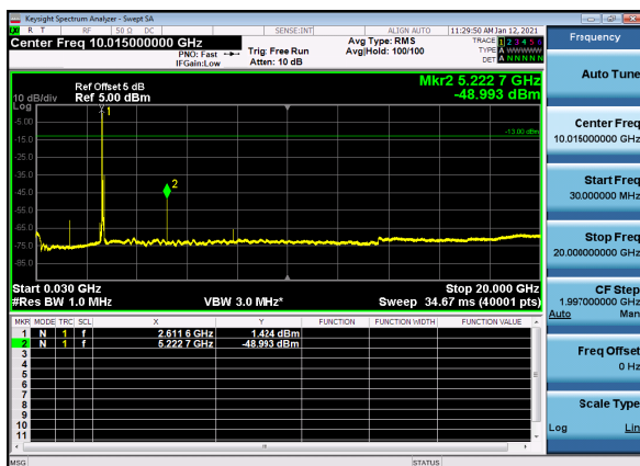
N41(80M)_DFT-s-OFDM_QPSK_Edge_1RB_High_CH
