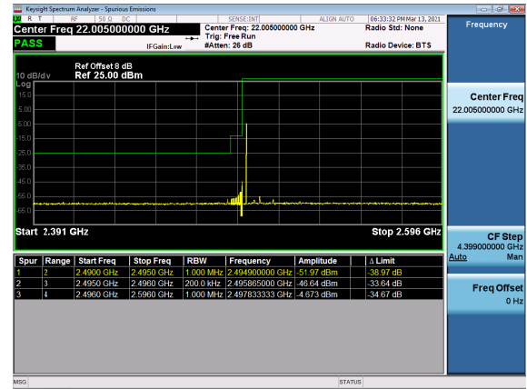
N41(20M)_DFT-s-OFDM_QPSK_Outer_Full_Low_CH
