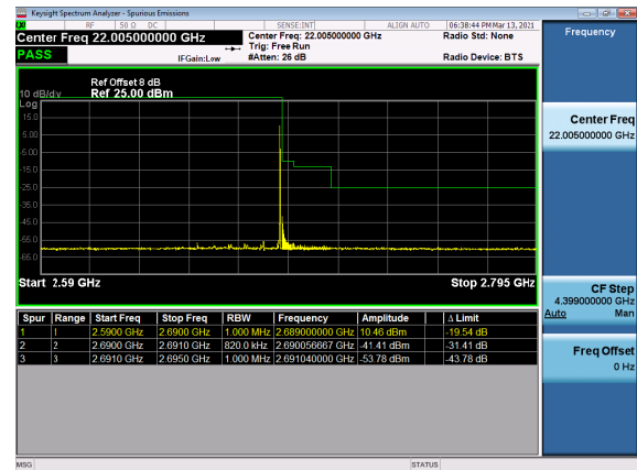
N41(40M)_DFT-s-OFDM_QPSK_Outer_Full_High_CH
