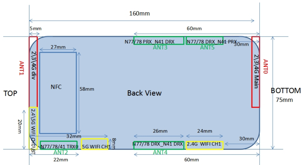
Antenna Location
