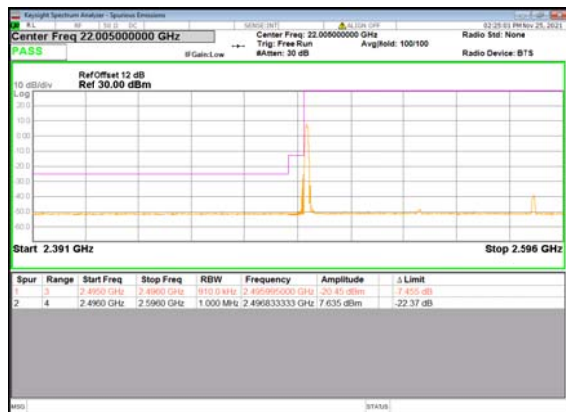
B2_N41(90M)_DFT-s-OFDM_BPSK_Edge_1R B_Left_Low_CH
