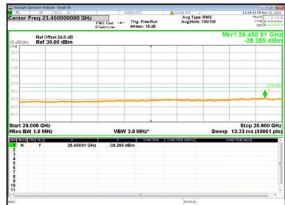
B2_N41(100M)_DFT-s-OFDM_BPSK_Edge_1 RB_Left_High_CH
