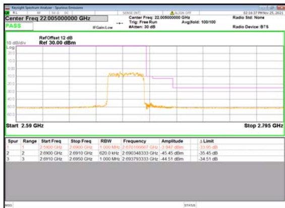
B2_N41(30M)_DFT-s-OFDM_BPSK_Outer_Ful I_High_CH
