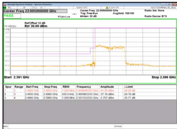
B2_N41(40M)_DFT-s-OFDM_BPSK_Outer_Ful I_Low_CH
