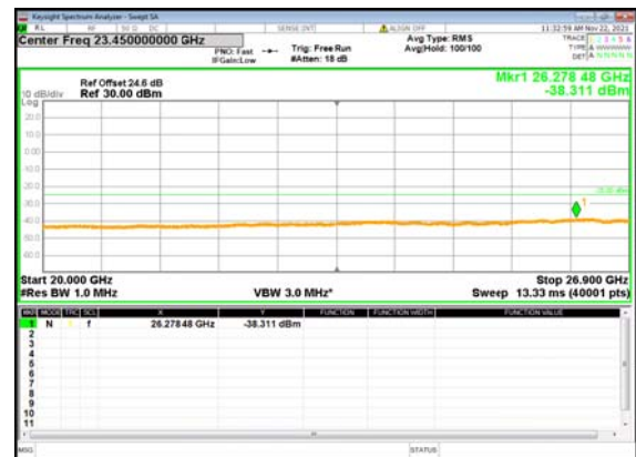
B2_N41(50M)_DFT-s-OFDM_BPSK_Edge_1R B_Left_High_CH
