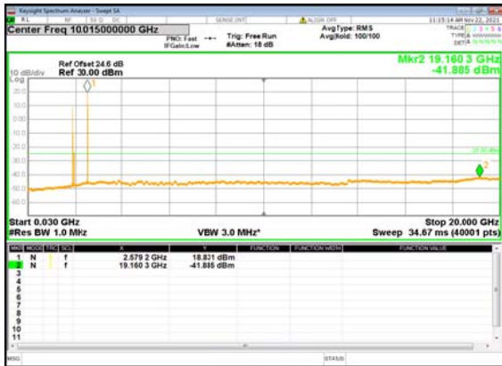
B2_N41(30M)_DFT-s-OFDM_QPSK_Edge_1R B_Left_Mid_CH
