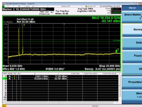
2A_N41(70M)_DFT-s-OFDM_QPSK_Edge_1R B_Left_High_CH
