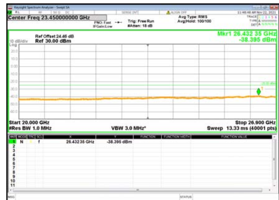
B2_N41(80M)_DFT-s-OFDM_BPSK_Edge_1R B_Left_High_CH
