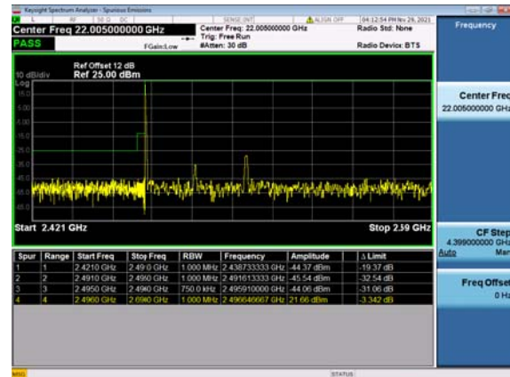
2A_N41(70M)_DFT-s-OFDM_QPSK_Edge_1R B_Left_Low_CH
