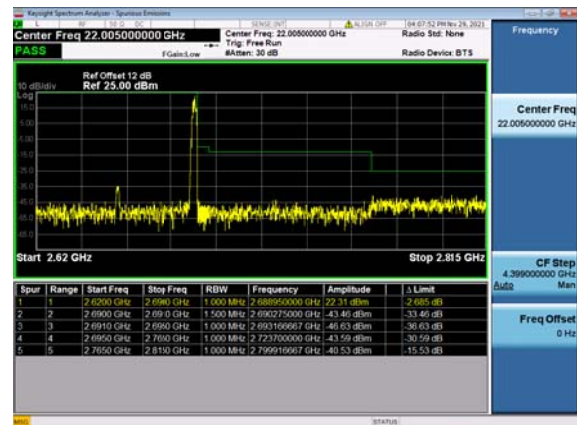
2A_N41(70M)_DFT-s-OFDM_QPSK_Edge_1R B_Right_High_CH
