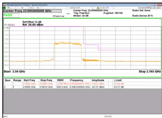
B2_N41(40M)_DFT-s-OFDM_BPSK_Outer_Ful I_High_CH
