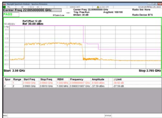
B2_N41(80M)_DFT-s-OFDM_BPSK_Outer_Ful I_High_CH
