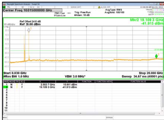
B2_N41(80M)_DFT-s-OFDM_QPSK_Edge_1R B_Left_Mid_CH
