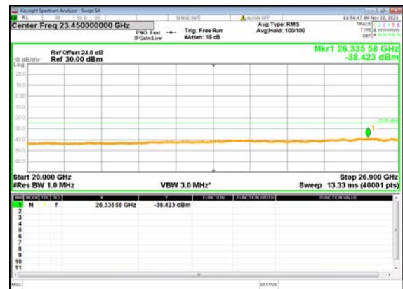
B2_N41(90M)_DFT-s-OFDM_BPSK_Edge_1R B_Left_High_CH
