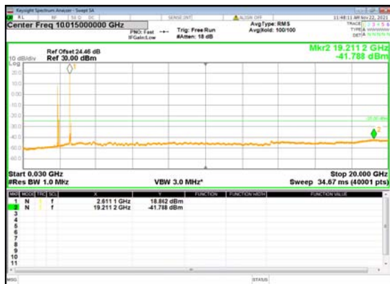
B2_N41(80M)_DFT-s-OFDM_BPSK_Edge_1R B_Left_High_CH
