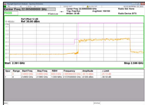
B2_N41(80M)_DFT-s-OFDM_QPSK_Outer_Ful I_Low_CH
