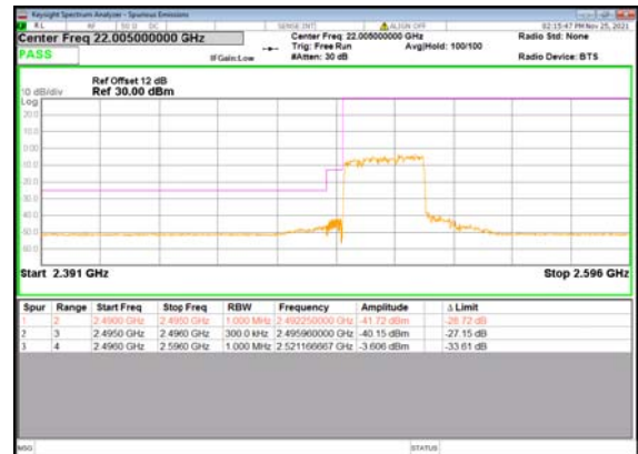
B2_N41(30M)_DFT-s-OFDM_QPSK_Outer_Ful I_Low_CH
