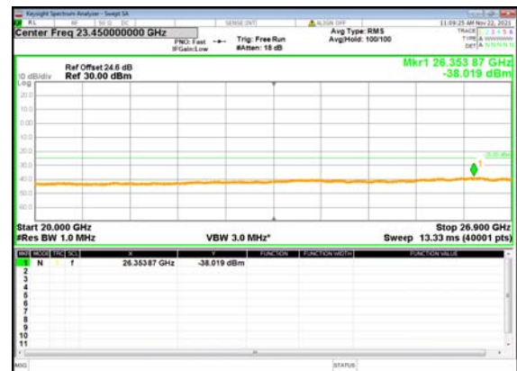
B2_N41(20M)_DFT-s-OFDM_BPSK_Edge_1R B_Left_High_CH
