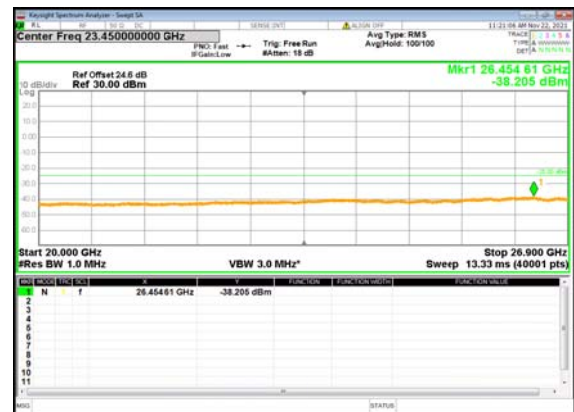
B2_N41(40M)_DFT-s-OFDM_QPSK_Edge_1R B_Left_Low_CH
