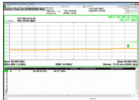
B2_N41(40M)_DFT-s-OFDM_BPSK_Edge_1R B_Left_Mid_CH
