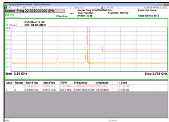
B2_N41(40M)_DFT-s-OFDM_QPSK_Edge_1R B_Right_High_CH
