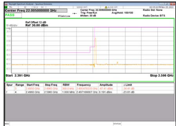
B2_N41(30M)_DFT-s-OFDM_QPSK_Edge_1R B_Left_Low_CH
