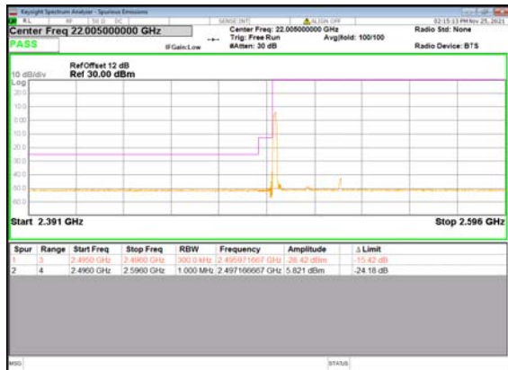
B2_N41(30M)_DFT-s-OFDM_BPSK_Edge_1R B_Left_Low_CH
