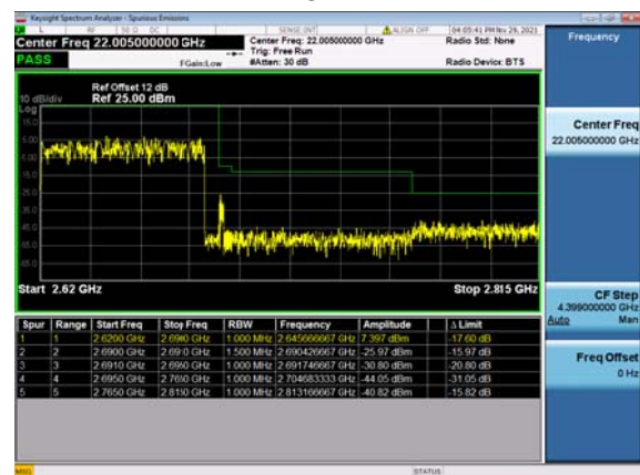
2A_N41(70M)_DFT-s-OFDM_QPSK_Outer_Ful I_High_CH
