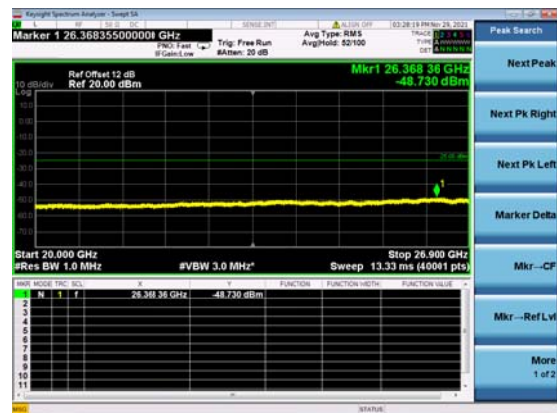
2A_N41(70M)_DFT-s-OFDM_BPSK_Edge_1R B_Left_Mid_CH
