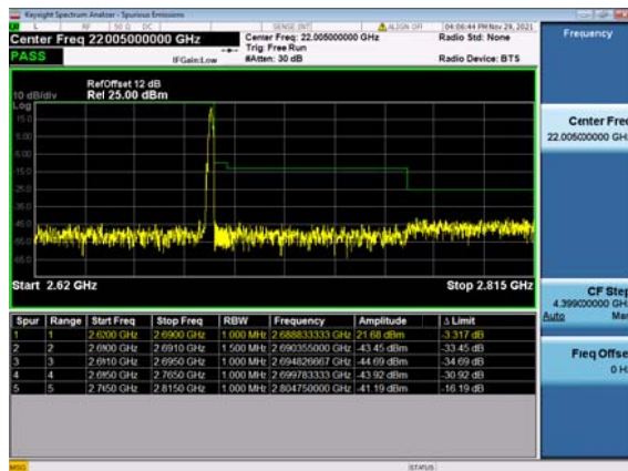
2A_N41(70M)_DFT-s-OFDM_BPSK_Edge_1R B_Right_High_CH
