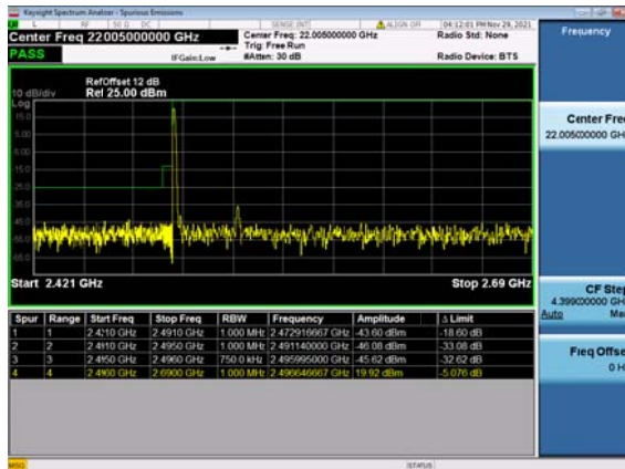
2A_N41(70M)_DFT-s-OFDM_BPSK_Edge_1R B_Left_Low_CH
