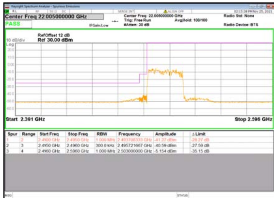
B2_N41(30M)_DFT-s-OFDM_BPSK_Outer_Ful I_Low_CH
