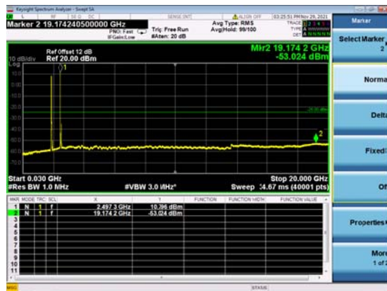
2A_N41(70M)_DFT-s-OFDM_QPSK_Edge_1R B_Left_Low_CH
