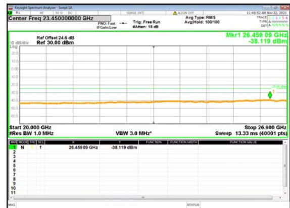
B2_N41(60M)_DFT-s-OFDM_BPSK_Edge_1R B_Left_High_CH
