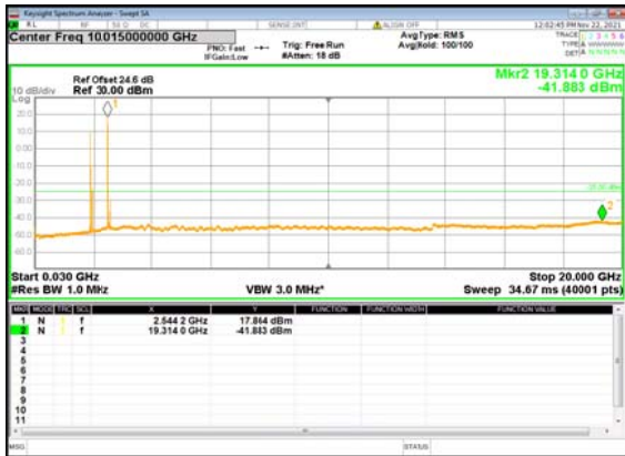
B2_N41(100M)_DFT-s-OFDM_QPSK_Edge_1 RB_Left_Mid_CH
