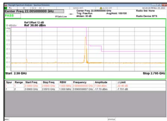
B2_N41(80M)_DFT-s-OFDM_QPSK_Edge_1R B_Right_High_CH
