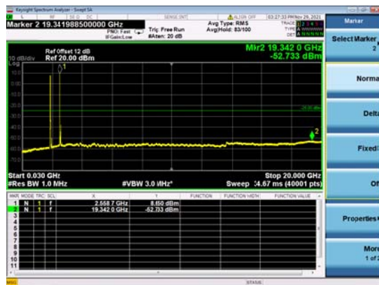
2A_N41(70M)_DFT-s-OFDM_BPSK_Edge_1R B_Left_Mid_CH
