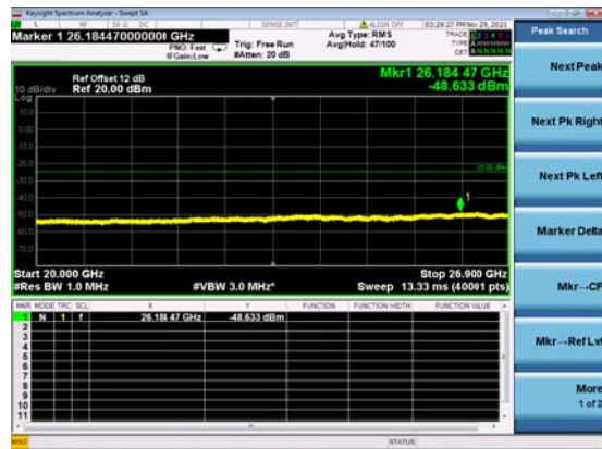
2A_N41(70M)_DFT-s-OFDM_QPSK_Edge_1R B_Left_Mid_CH
