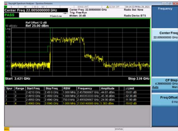
2A_N41(70M)_DFT-s-OFDM_QPSK_Outer_Ful I_Low_CH
