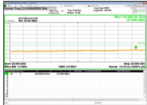
B2_N41(40M)_DFT-s-OFDM_BPSK_Edge_1R B_Left_Low_CH
