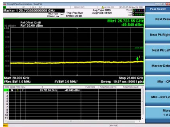
2A_N41(70M)_DFT-s-OFDM_BPSK_Edge_1R B_Left_High_CH
