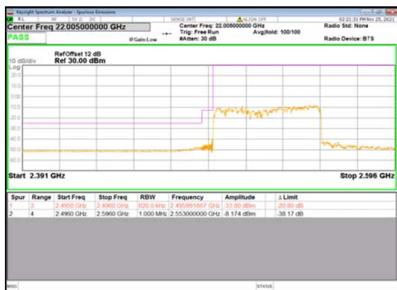
B2_N41(60M)_DFT-s-OFDM_BPSK_Outer_Ful I_Low_CH
