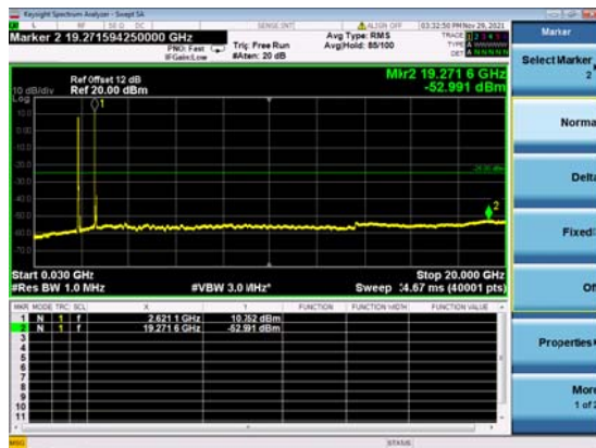
2A_N41(70M)_DFT-s-OFDM_BPSK_Edge_1R B_Left_High_CH
