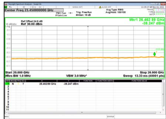
B2_N41(60M)_DFT-s-OFDM_BPSK_Edge_1R B_Left_Low_CH
