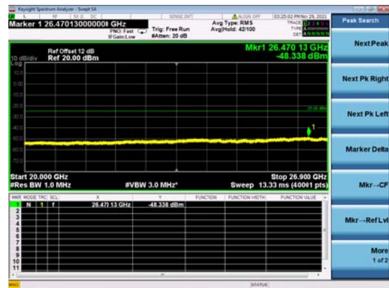
2A_N41(70M)_DFT-s-OFDM_QPSK_Edge_1R B_Left_Low_CH
