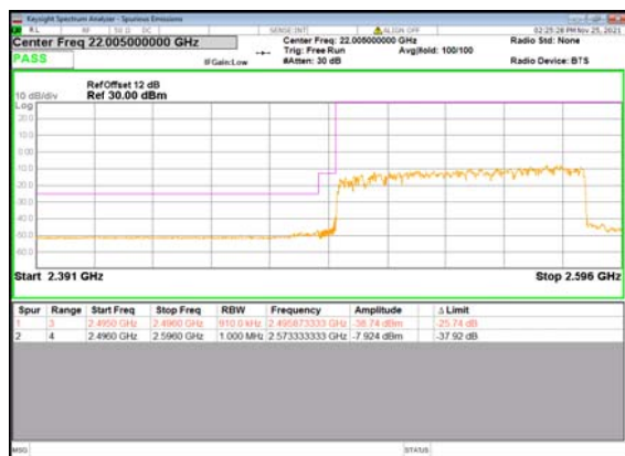
B2_N41(90M)_DFT-s-OFDM_BPSK_Outer_Ful I_Low_CH
