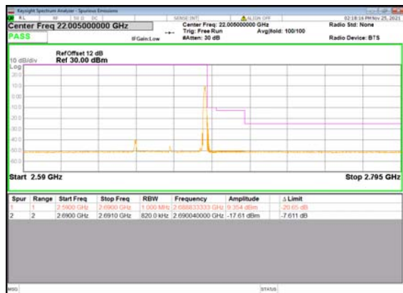
B2_N41(40M)_DFT-s-OFDM_BPSK_Edge_1R B_Right_High_CH
