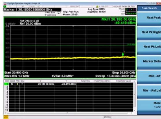
2A_N41(70M)_DFT-s-OFDM_BPSK_Edge_1R B_Left_Low_CH
