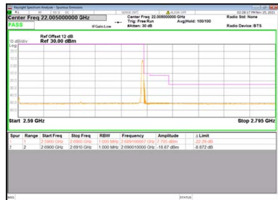
B2_N41(100M)_DFT-s-OFDM_QPSK_Edge_1 RB_Right_High_CH
