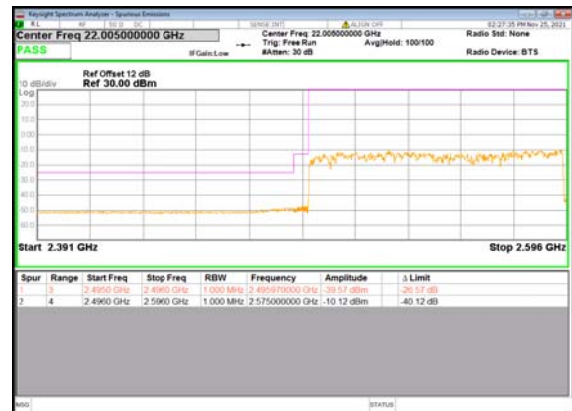
B2_N41(100M)_DFT-s-OFDM_QPSK_Outer_F ull_Low_CH
