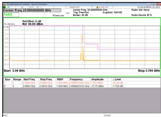
B2_N41(100M)_DFT-s-OFDM_BPSK_Edge_1 RB_Right_High_CH
