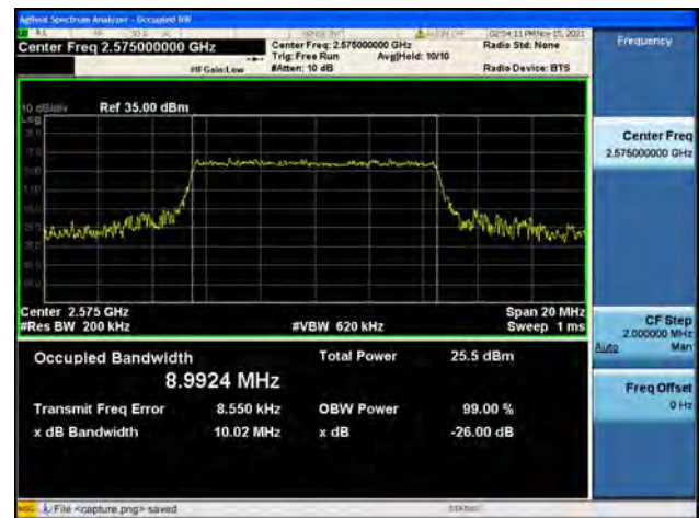
Band38 / 10MHz / Low CH / 64QAM
