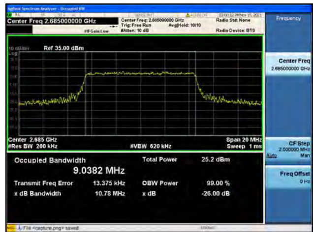
Band41 / 10MHz / High CH / 64QAM
