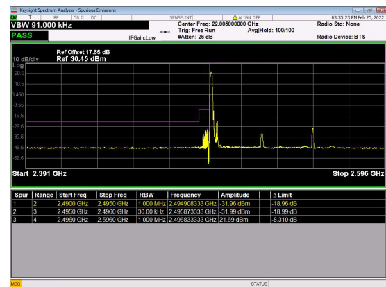
n41(60M)_DFT-s-OFDM_QPSK_Edge_1RB_ Left_Low_CH
