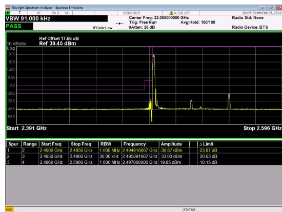
n41(60M)_DFT-s-OFDM_BPSK_Edge_1RB_ Left_Low_CH
