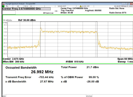
n41(30M)_DFT-s-OFDM_256QAM_Outer_Full_ High_CH
