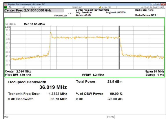
n41(40M)_DFT-s-OFDM_QPSK_Outer_Full_ Low_CH
