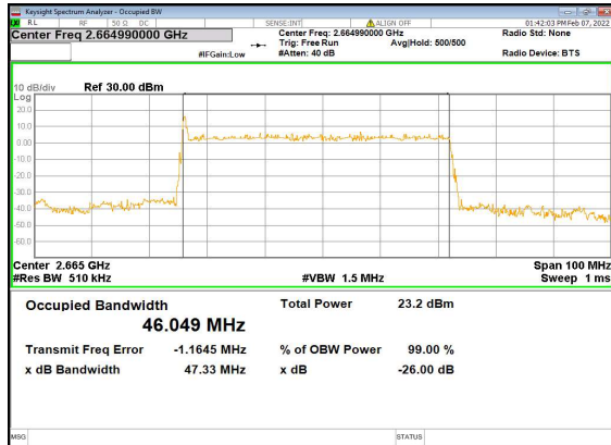
n41(50M)_DFT-s-OFDM_PI_2-BPSK_Outer_ Full_High_CH
