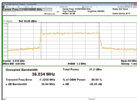
n41(40M)_DFT-s-OFDM_256QAM_Outer_Full_ Low_CH
