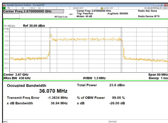
n41(40M)_DFT-s-OFDM_16QAM_Outer_Full_ High_CH
