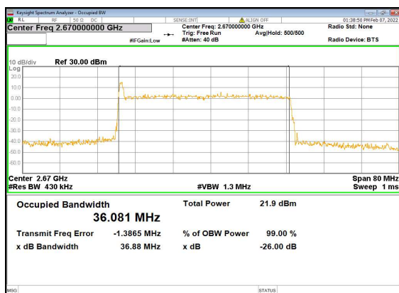
n41(40M)_DFT-s-OFDM_256QAM_Outer_Full_ High_CH
