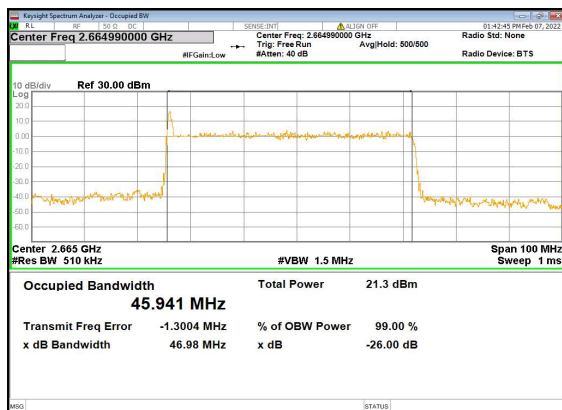
n41(50M)_DFT-s-OFDM_256QAM_Outer_Full_ High_CH
