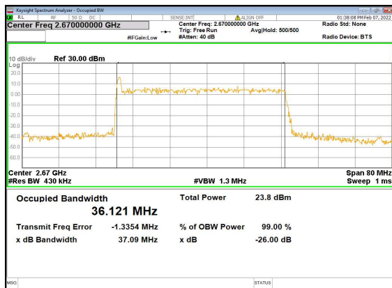
n41(40M)_DFT-s-OFDM_PI_2-BPSK_Outer_ Full_High_CH
