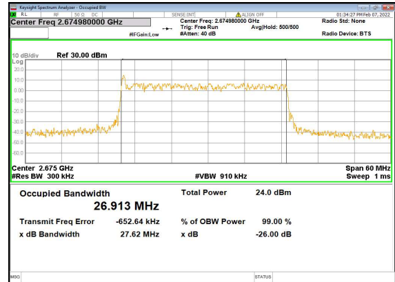
n41(30M)_DFT-s-OFDM_QPSK_Outer_Full_ High_CH
