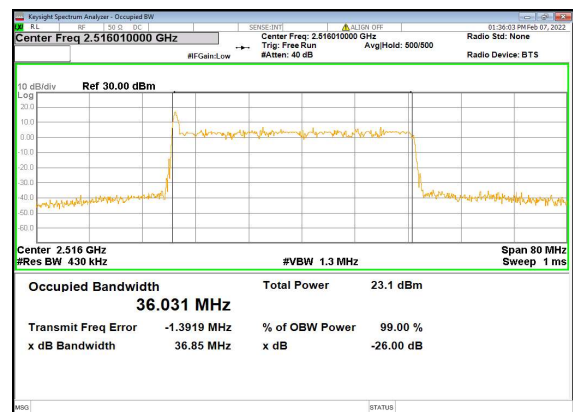
n41(40M)_DFT-s-OFDM_64QAM_Outer_ Full_Low_CH
