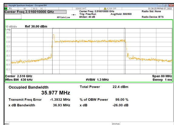
n41(40M)_CP-OFDM_QPSK_Outer_Full_ Low_CH
