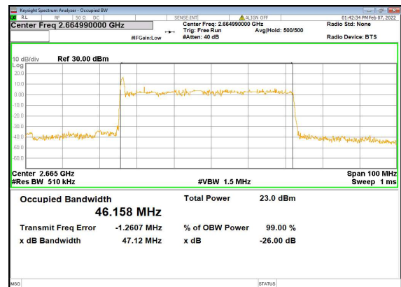
n41(50M)_DFT-s-OFDM_64QAM_Outer_ Full_High_CH
