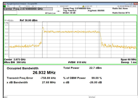
n41(30M)_CP-OFDM_QPSK_Outer_Full_ High_CH
