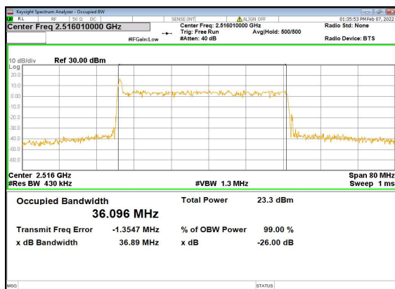
n41(40M)_DFT-s-OFDM_16QAM_Outer_Full_ Low_CH
