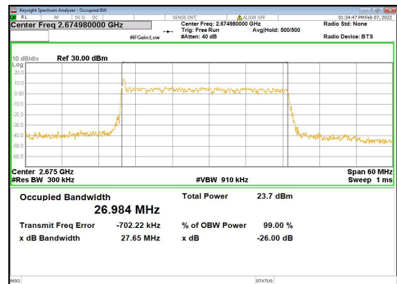
n41(30M)_DFT-s-OFDM_64QAM_Outer_ Full_High_CH
