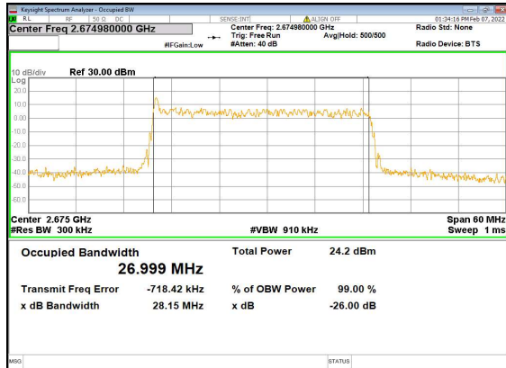
n41(30M)_DFT-s-OFDM_PI_2-BPSK_Outer_ Full_High_CH
