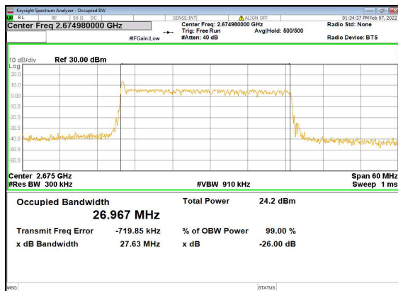
n41(30M)_DFT-s-OFDM_16QAM_Outer_Full_ High_CH
