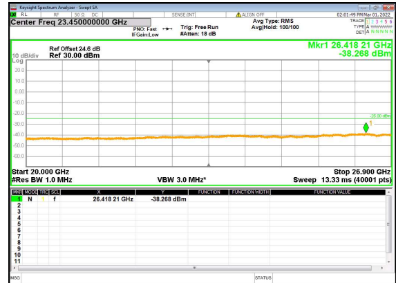
B2_n41(40M)_DFT-s-OFDM_QPSK_Edge_ 1RB_Left_Mid_CH
