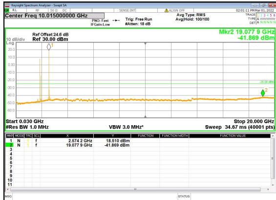
B2_n41(40M)_DFT-s-OFDM_QPSK_Edge_ 1RB_Left_Mid_CH
