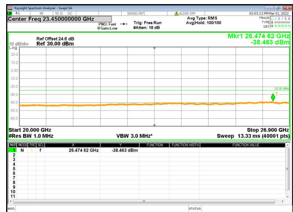
B2_n41(40M)_DFT-s-OFDM_BPSK_Edge_ 1RB_Left_High_CH
