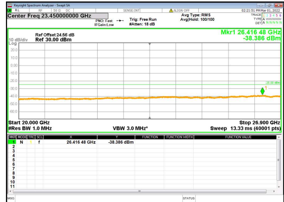
B2_n41(80M)_DFT-s-OFDM_BPSK_Edge_ 1RB_Left_Low_CH
