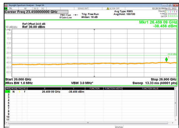
B2_n41(80M)_DFT-s-OFDM_QPSK_Edge_ 1RB_Left_High_CH
