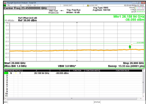
B2_n41(80M)_DFT-s-OFDM_QPSK_Edge_ 1RB_Left_Mid_CH
