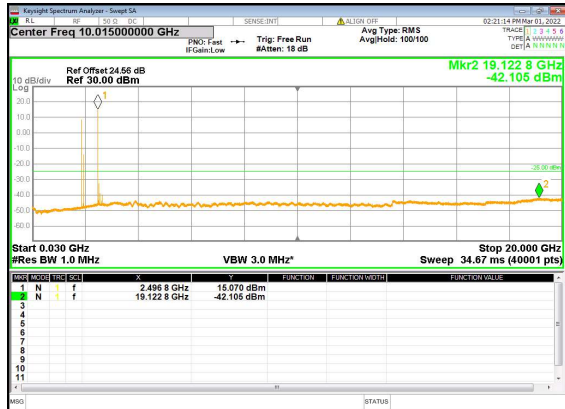
B2_n41(80M)_DFT-s-OFDM_BPSK_Edge_ 1RB_Left_Low_CH
