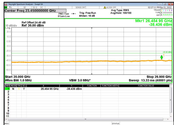
B2_n41(80M)_DFT-s-OFDM_BPSK_Edge_ 1RB_Left_High_CH
