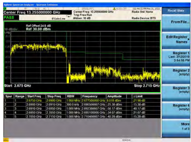
Band41 / 15MHz / High CH / QPSK / FULL RB
