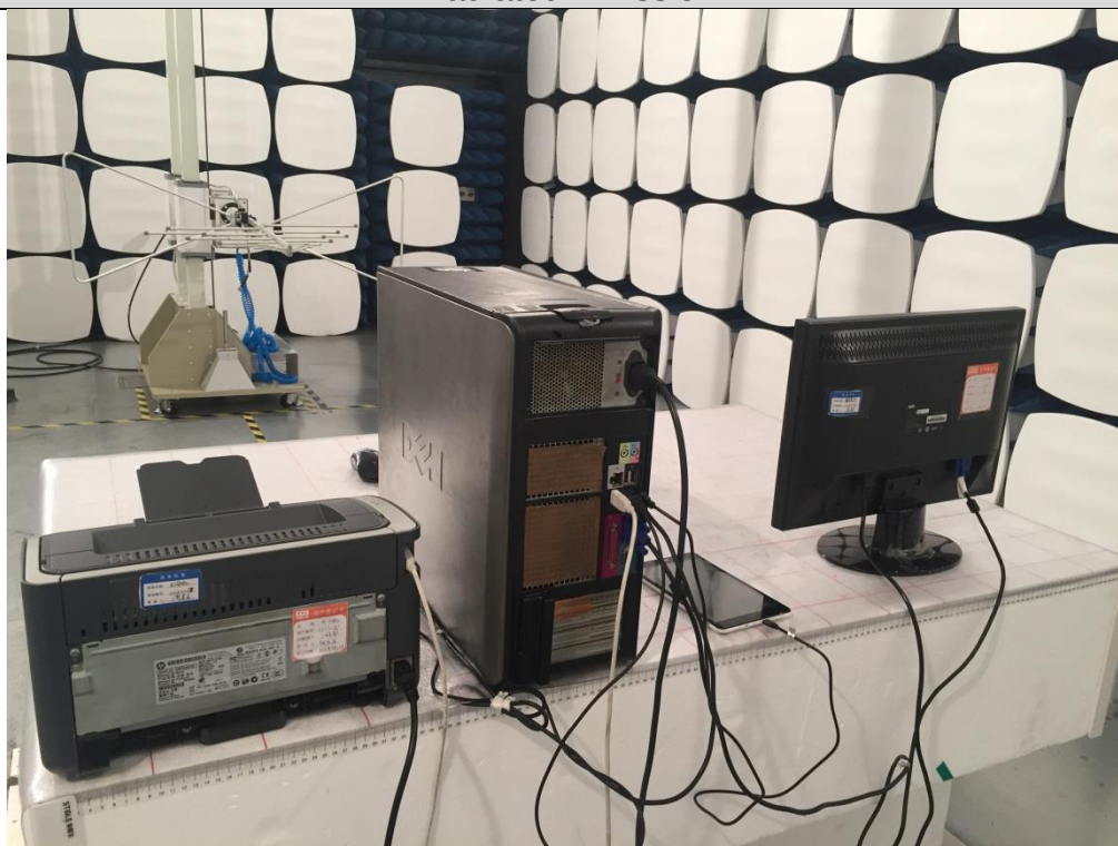
Test setup photo for PC mode Radiated Emission
