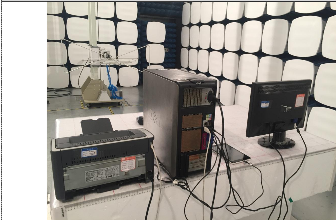
Radiated Emission
