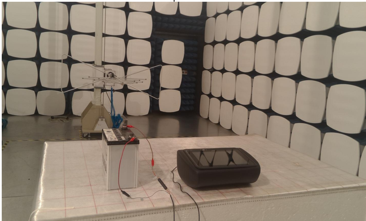
Radiated Spurious Emission
