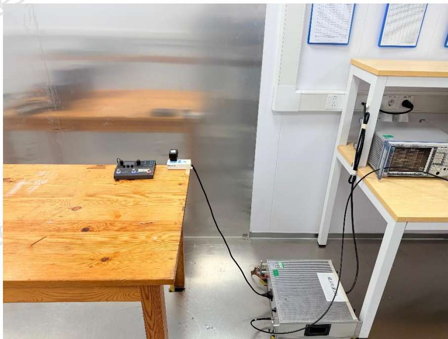
RF Tests
