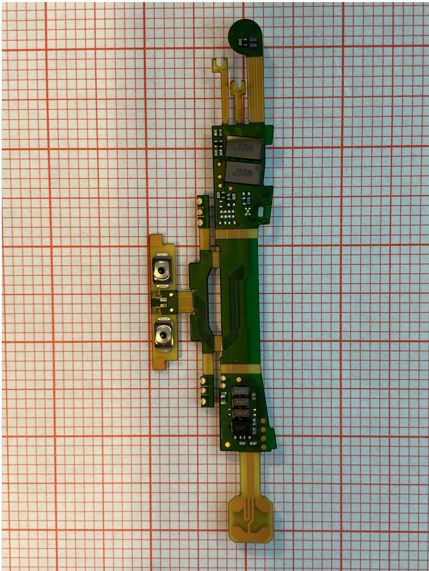
Sentio 1 PCB_Bottom_view
