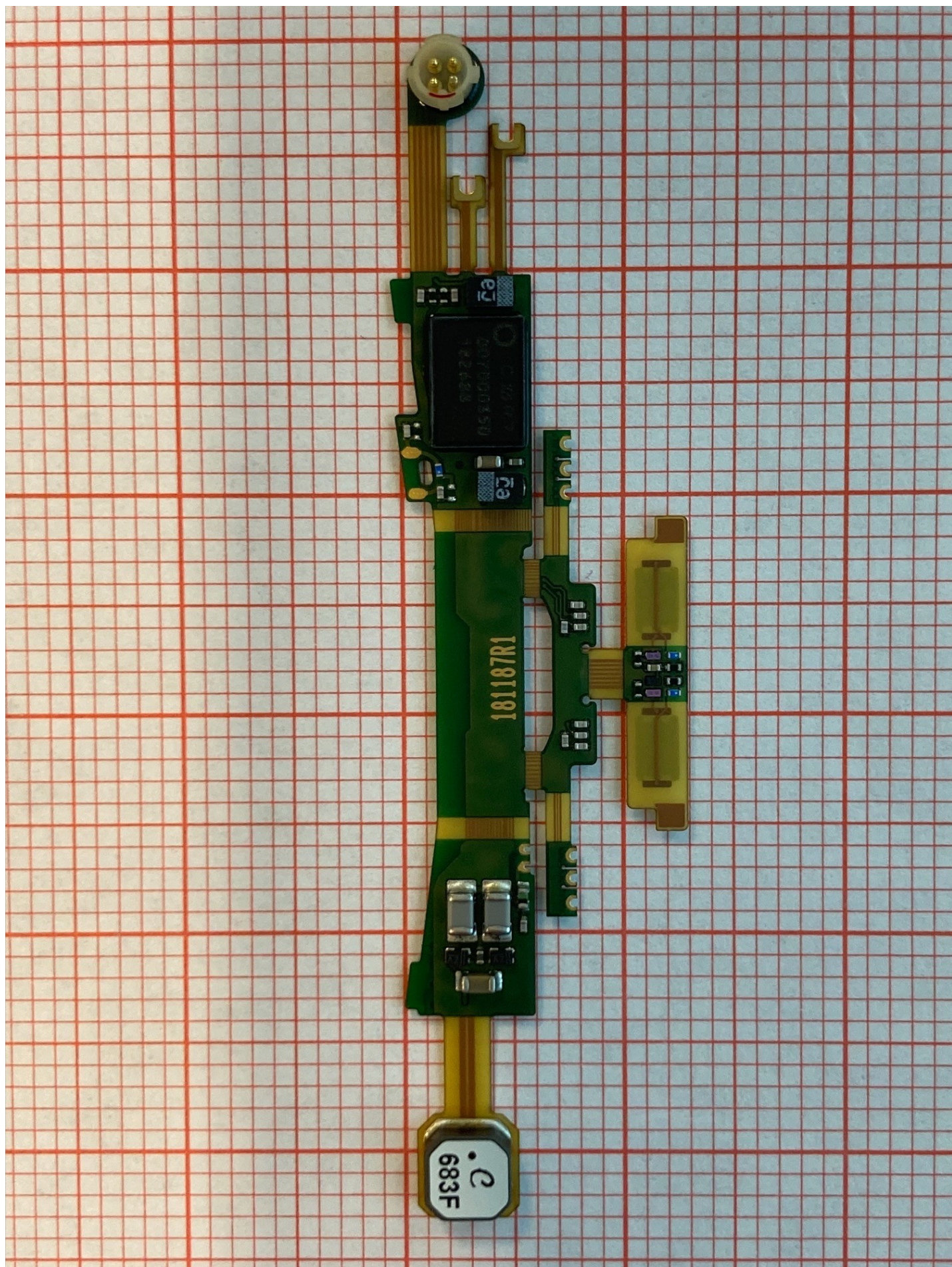
Sentio 1 PCB_Top_view
