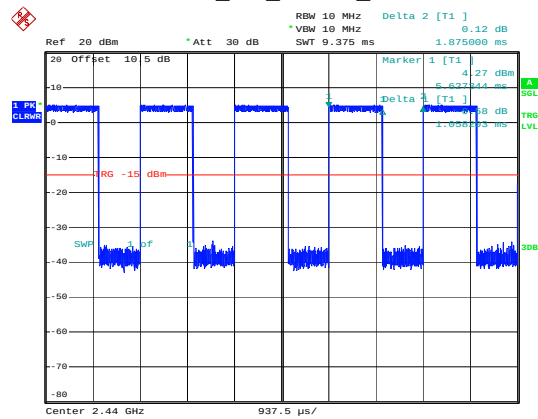
BLE_2M_Middle_Channel
