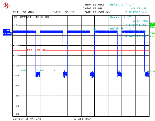
BLE_1M_Middle_Channel
