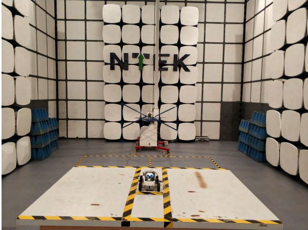
Radiated Measurement Photos (Power by alkaline battery)
