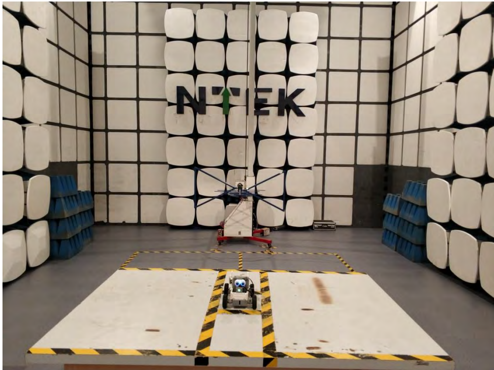
Radiated Measurement Photos(Power by li-ion battery)
