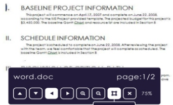
* Text Interface
