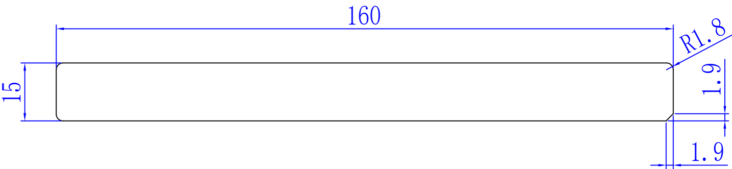
尺寸图(Die cut)
