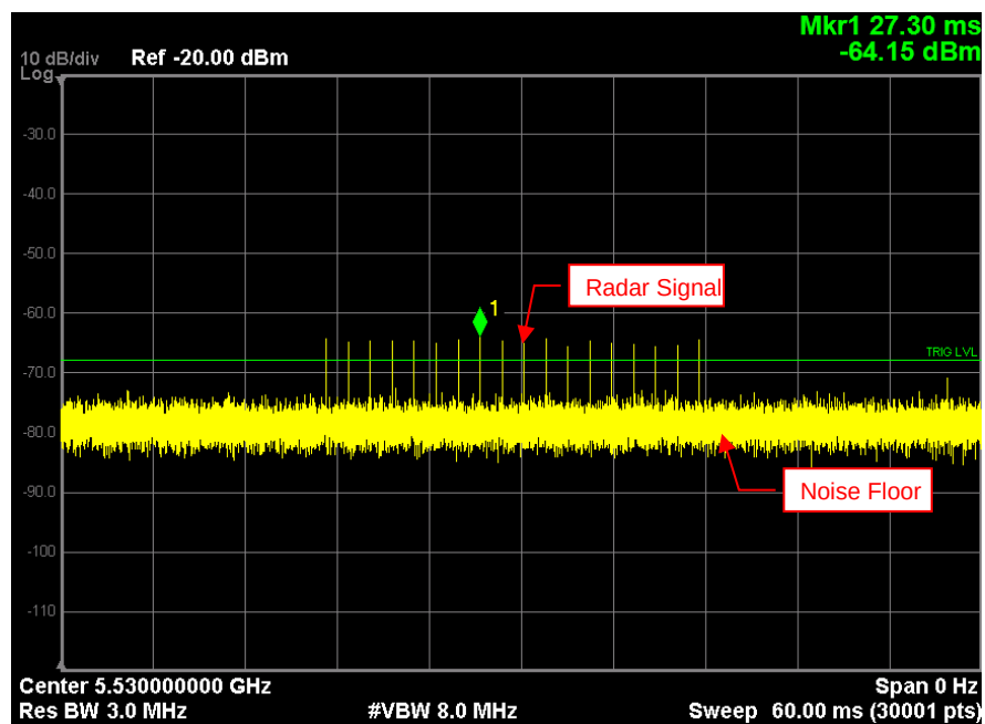
Radar Signal 0
