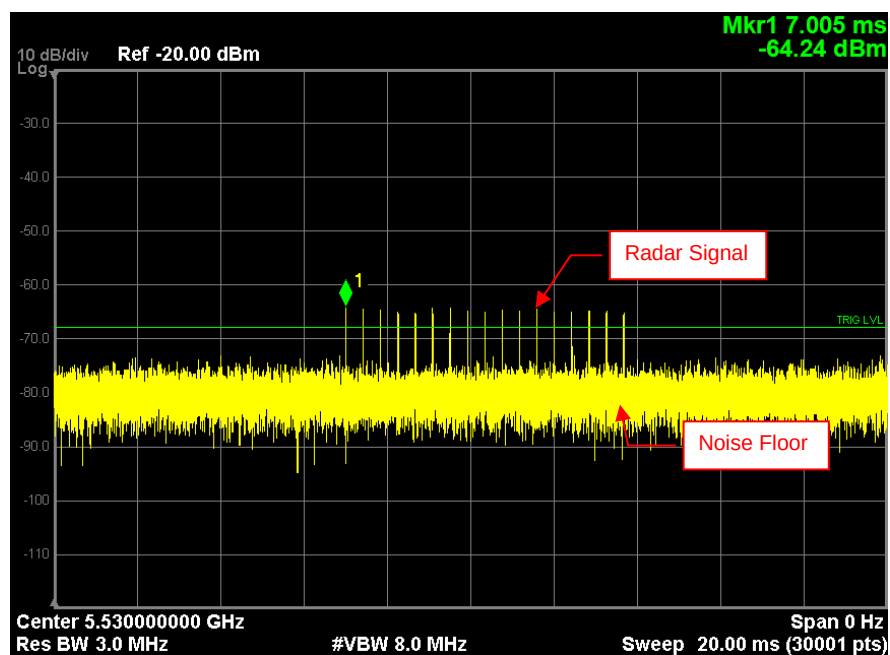
Radar Signal 3
