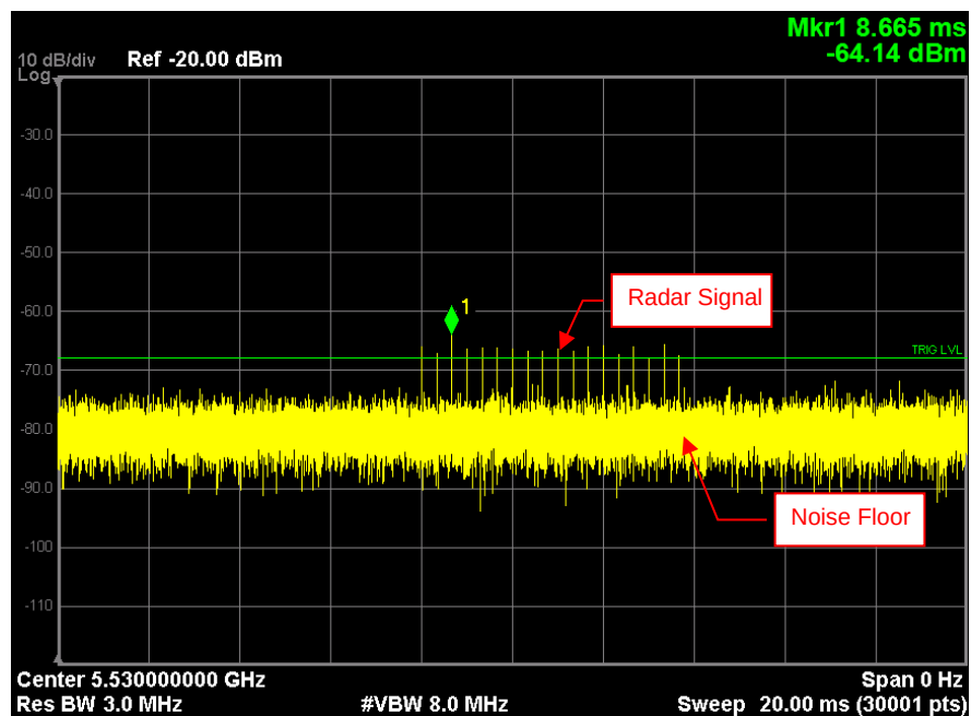
Radar Signal 6
