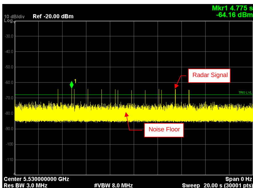
Radar Signal 5
