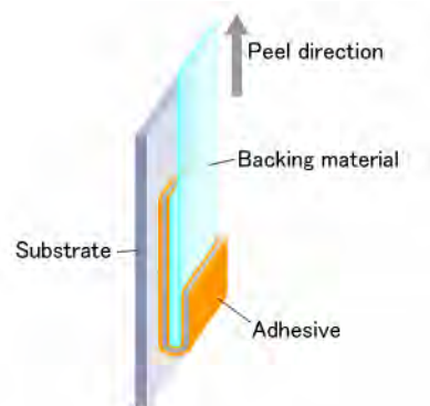
<180° peeling strength test>
