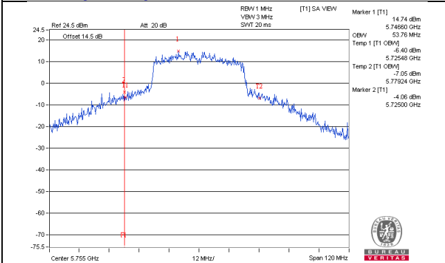
802.11ac(VHT40)_Chain2 / CH151
