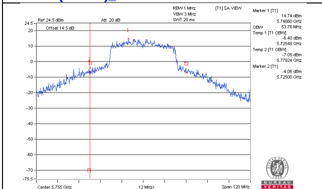
802.11ac(VHT40)_Chain2 / CH151
