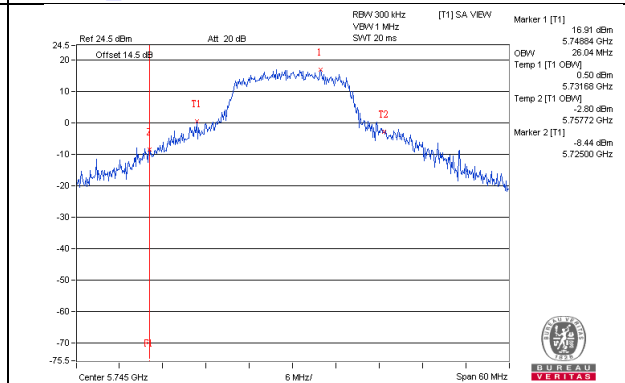
802.11ac(VHT20)_Chain1 / CH149
