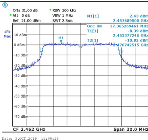
Figure 73. 2462.0 MHz, Wi-fi/g(54Mbit/s)
