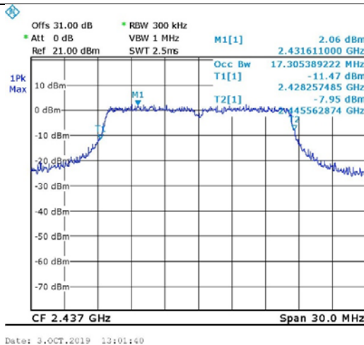
Figure 71. 2437.0 MHz, Wi-fi/g(54Mbit/s)
