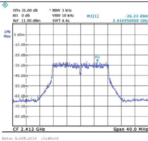
Figure 55. 2412.0 MHz, Wi-fi/g(54Mbit/s)
