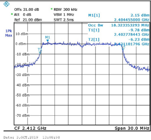
Figure 70. 2412.0 MHz, Wi-fi/n(65Mbit/s)
