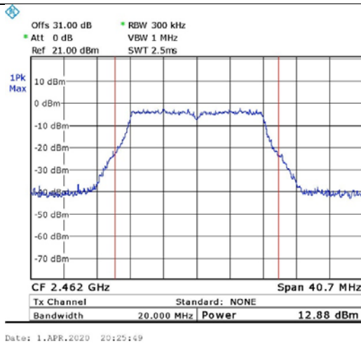
Figure 29. 2462.0 MHz, Wi-fi/g(6Mbit/s)
