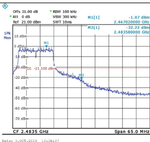
Figure 45. 2462.0 MHz, Wi-fi/g(54Mbit/s)
