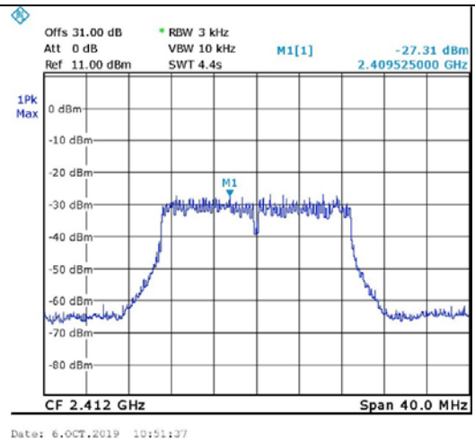
Figure 56. 2412.0 MHz, Wi-fi/n(65Mbit/s)
