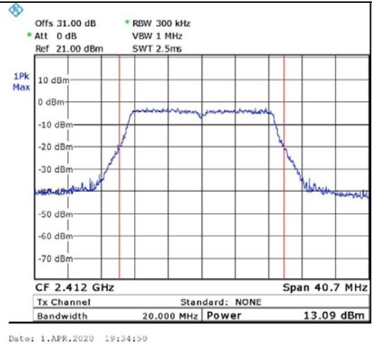
Figure 26. 2412.0 MHz, Wi-fi/n(6.5Mbit/s)
