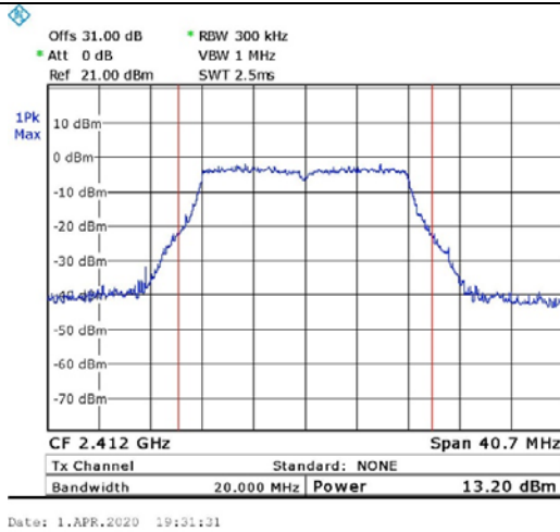
Figure 25. 2412.0 MHz, Wi-fi/g(6Mbit/s)
