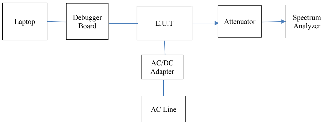
Figure 2. Configuration of Tested System Conducted
