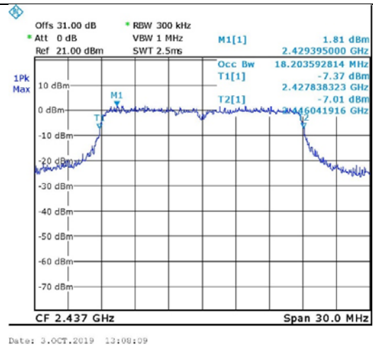
Figure 72. 2437.0 MHz, Wi-fi/n(65Mbit/s)
