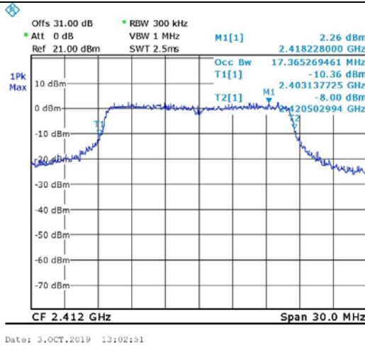
Figure 69. 2412.0 MHz, Wi-fi/g(54Mbit/s)
