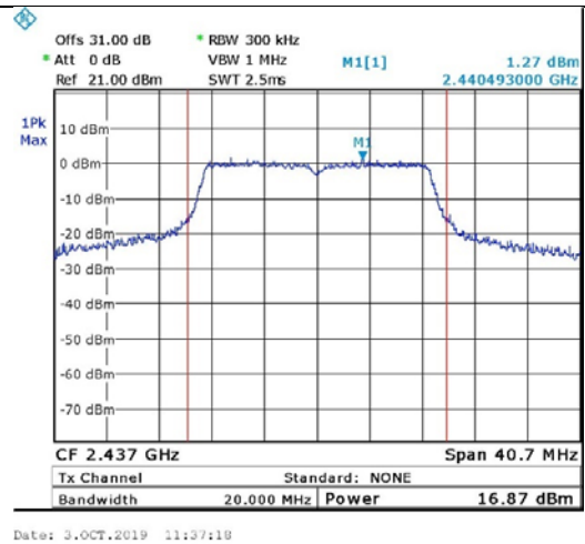
Figure 28. 2437.0 MHz, Wi-fi/n(6.5Mbit/s)
