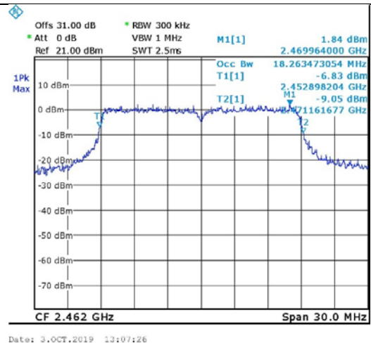
Figure 74. 2462.0 MHz, Wi-fi/n(65Mbit/s)
