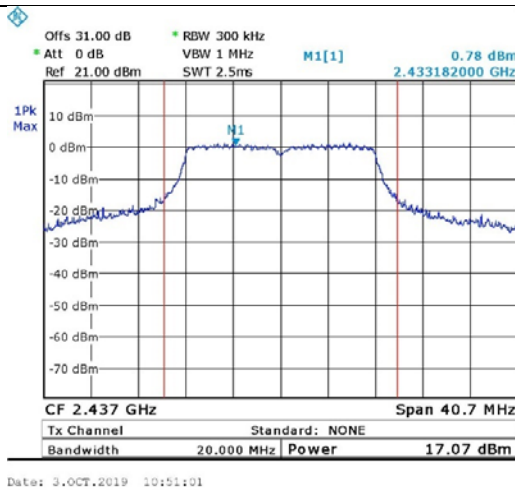
Figure 27. 2437.0 MHz, Wi-fi/g(6Mbit/s)
