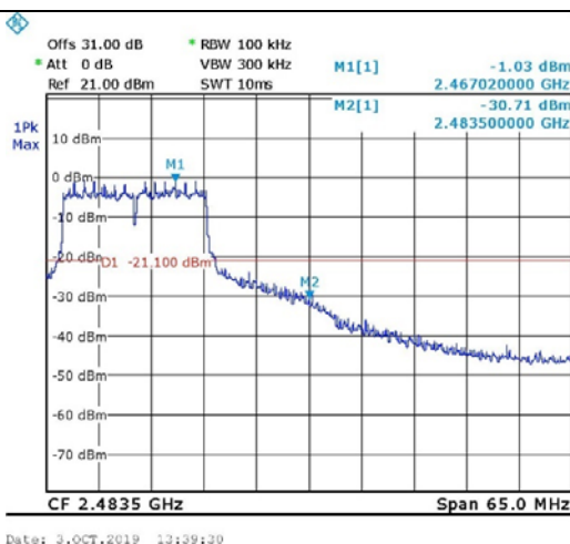
Figure 46. 2462.0 MHz, Wi-fi/n(65Mbit/s)
