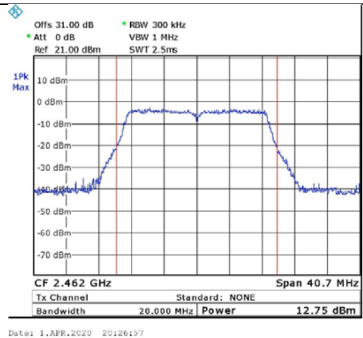
Figure 30. 2462.0 MHz, Wi-fi/n(6.5Mbit/s)
