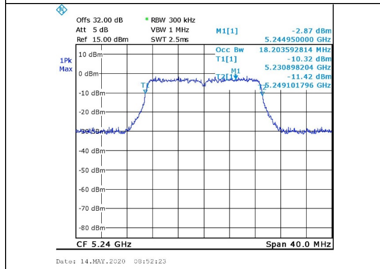
Figure 53. 5240.0 MHz, Wi-fi/n(65Mbit/s)
