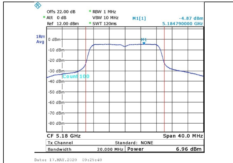
Figure 16. 5180.0 MHz, Wi-fi/n(65Mbit/s)
