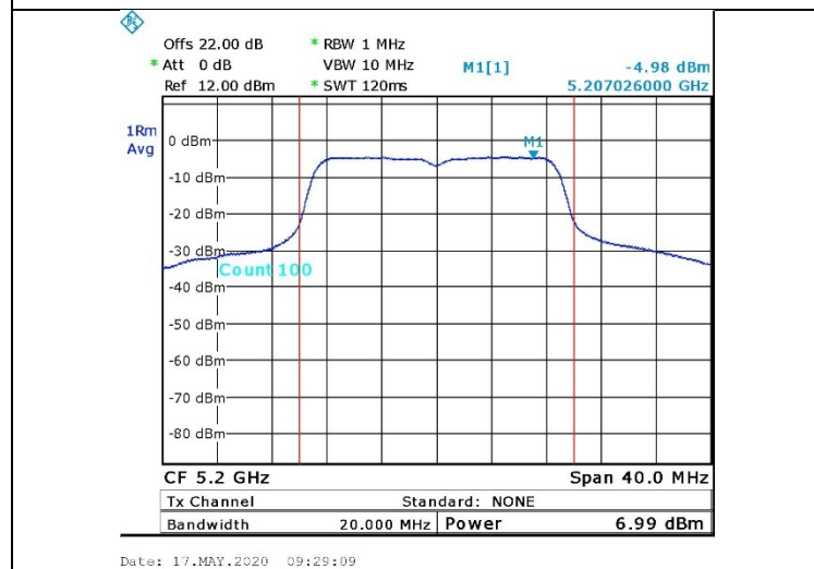
Figure 17. 5200.0 MHz, Wi-fi/n(65Mbit/s)
