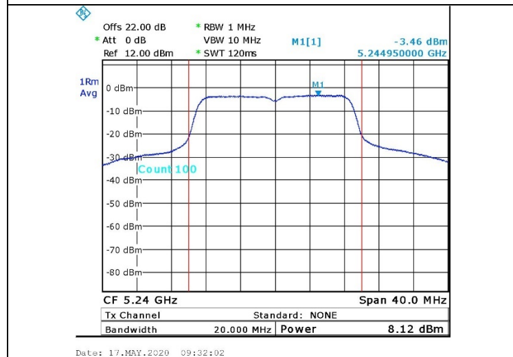
Figure 18. 5240.0 MHz, Wi-fi/n(65Mbit/s)
