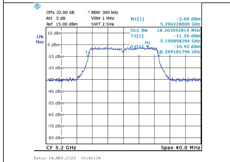
Figure 52. 5200.0 MHz, Wi-fi/n(65Mbit/s)
