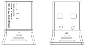
Nano receiver Model: CKM620R FCC ID: 2AHKSCKM620R size: 10.8x3.3mm Laser printing on Nano Receiver
