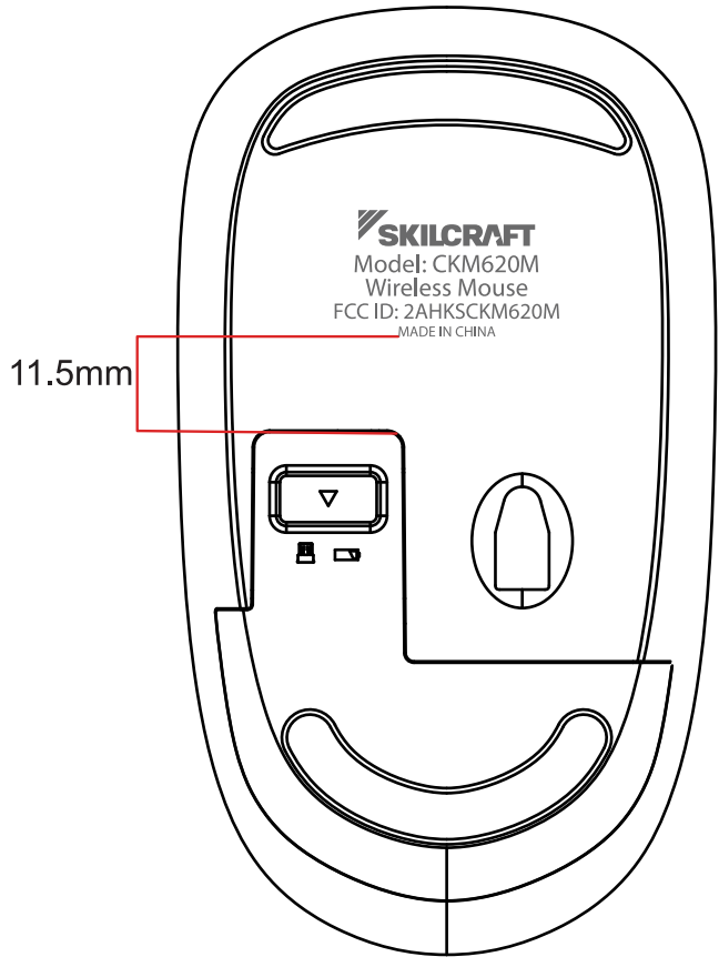
SKILCRAFT Model: CKM620M Wireless Mouse FCC ID: 2AHKSCKM620M MADE IN CHINA 26.7x15mm Silk printing color: Cool gray 6C
