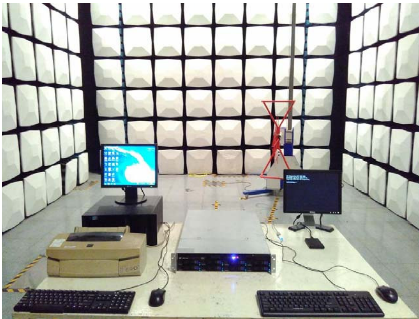
Radiated Emissions Test Setup - Front View (Below 1GHz)
