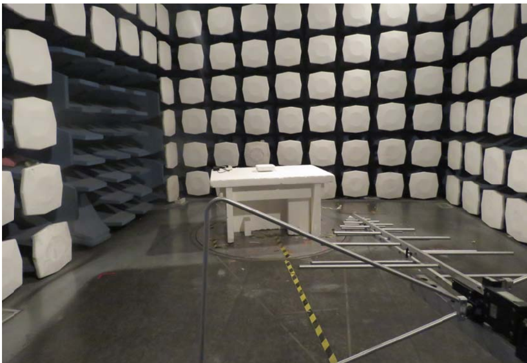
30MHz-1GHz
