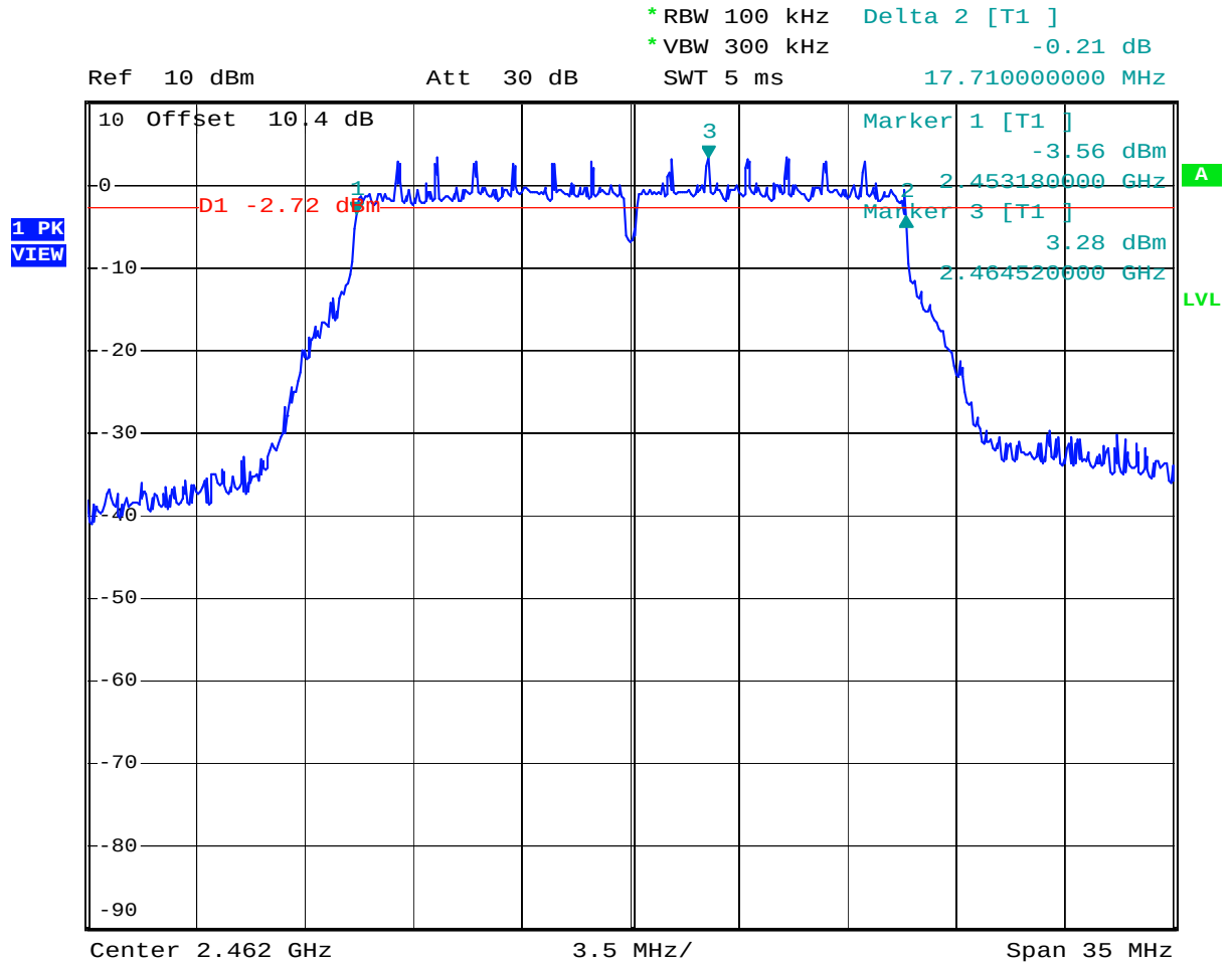
Plot 1.9 – 6dB Bandwidth (FCC)
