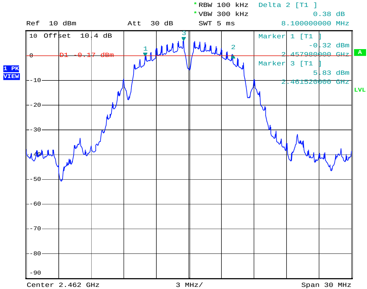
Plot 1 3 – 6dB Bandwidth (FCC)
