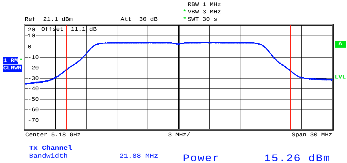
Plot 2. 1 802.11a, 5180MHz
