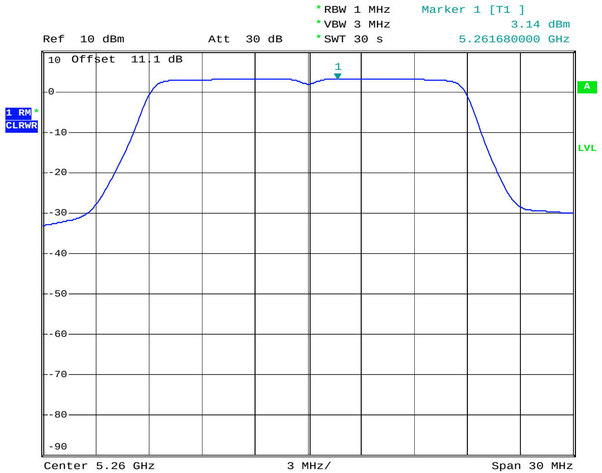
Plot 3. 10 802.11a, 5260MHz
