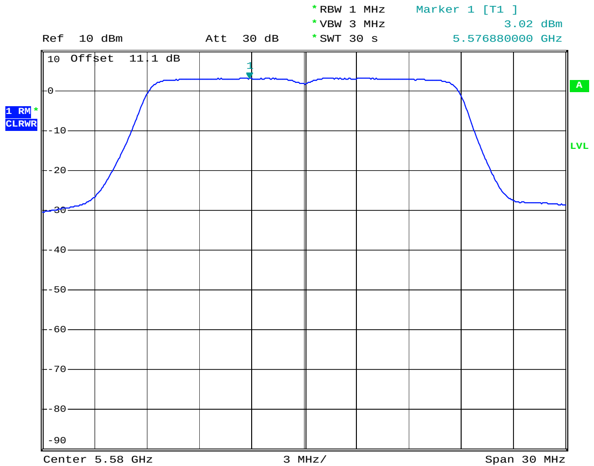
Plot 3.2 802.11a, 5580MHz
