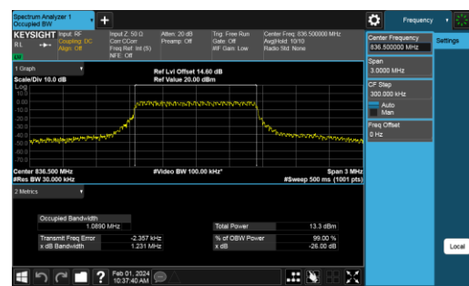
B5-1.4M-Mid CH-OBW-Q16
