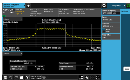
B5-1.4M-Mid CH-OBW-QPSK
