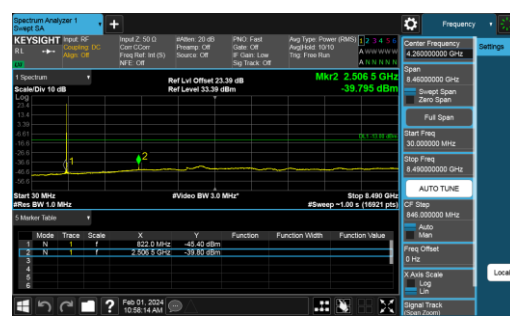
B5-3M-Mid CH-CSE-1-QPSK-1 RB 0
