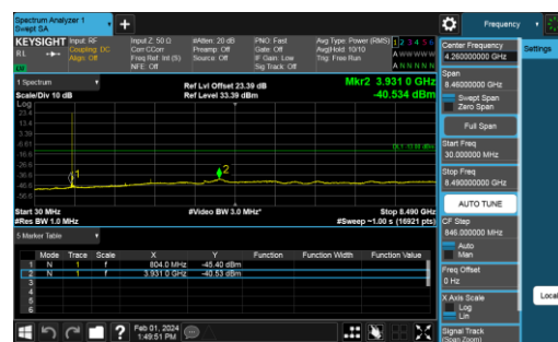
B5-5M-Mid CH-CSE-1-QPSK-1 RB 0
