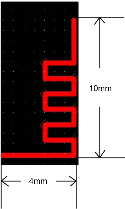
Antenna Photo & Length (mm)
