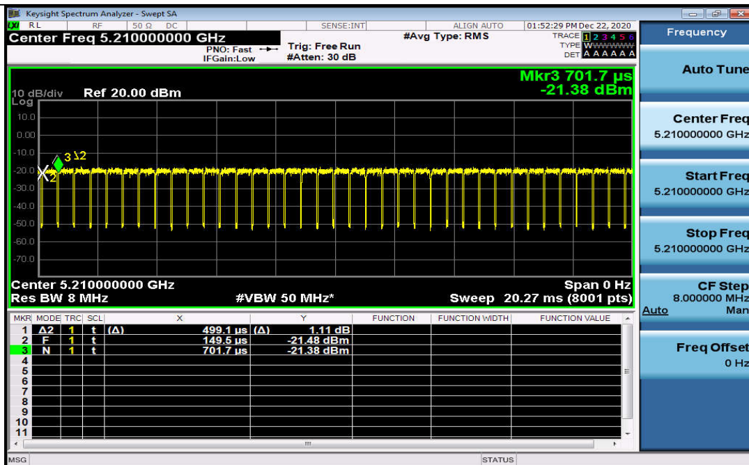
Duty Cycle_11AC80MIMO_5210_Ant2
