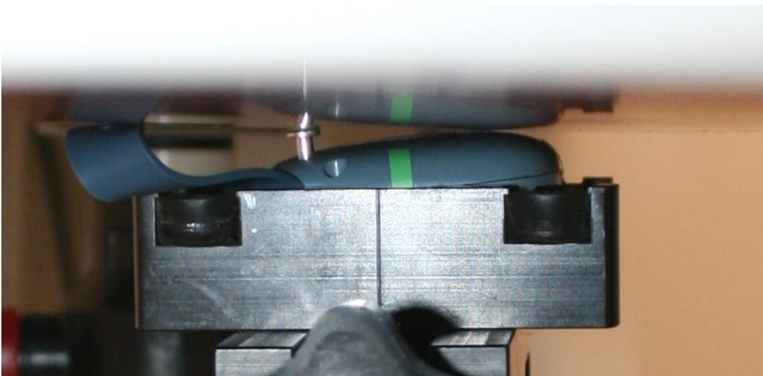
Guardian module: Back side of the device against the phantom, 0mm separation
