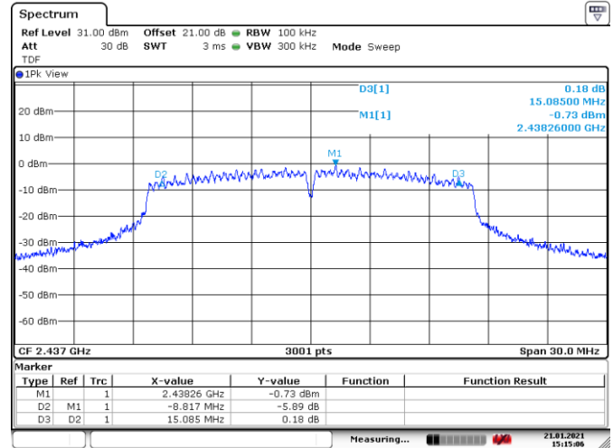
Figure 8.8-2: PSD on mid channel
