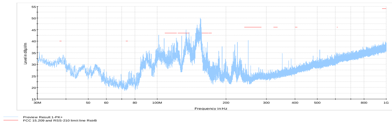
Figure 8.7-17: Cabinet radiated Spurious emissions within 30 to 1000 MHz, Tx @ mid channel
