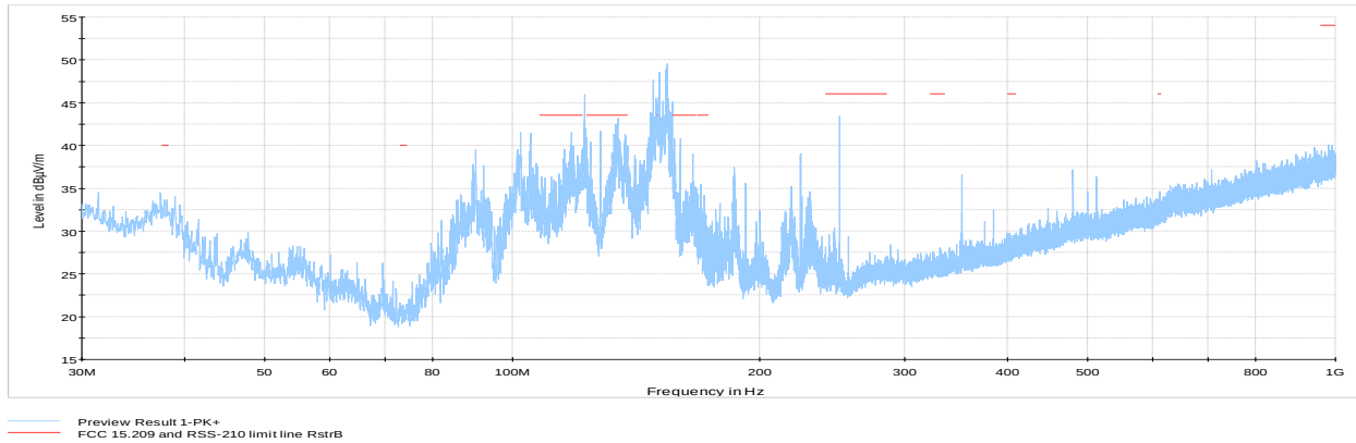
Figure 8.7-16: Cabinet radiated Spurious emissions within 30 to 1000 MHz, Tx @ low channel
