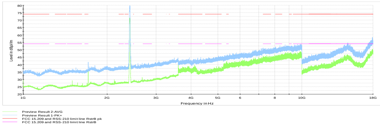
Figure 8.7-19: Cabinet radiated Spurious emissions 1 to 18 GHz, Tx @ low channel
