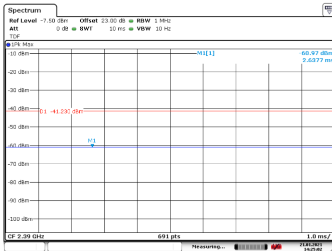
Figure 8.7-8: Conducted spurious emissions on 2390 MHz, average, Tx on low channel
