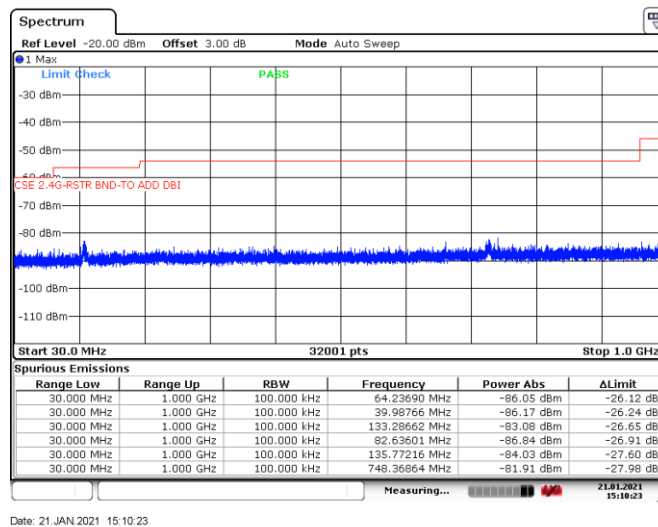
Figure 8.7-12: Conducted spurious emissions 30 MHz to 1 GHz within restricted bands, Tx on high channel
