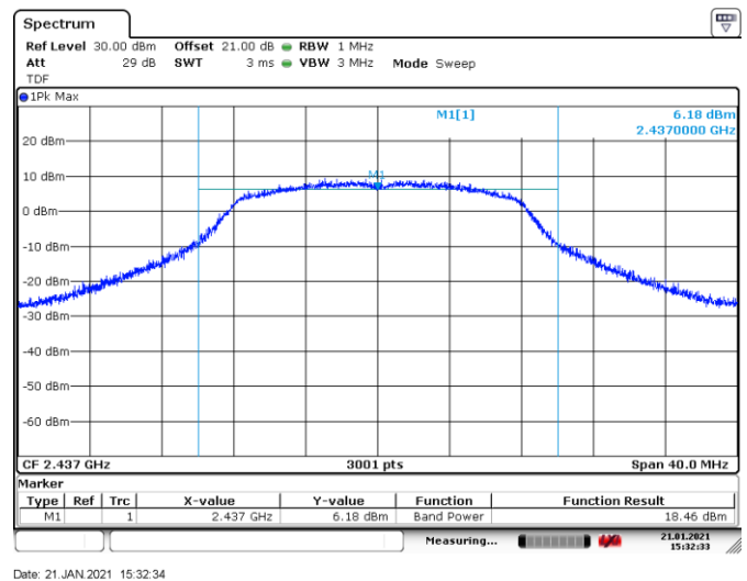
Figure 8.6-2: Output power on mid channel
