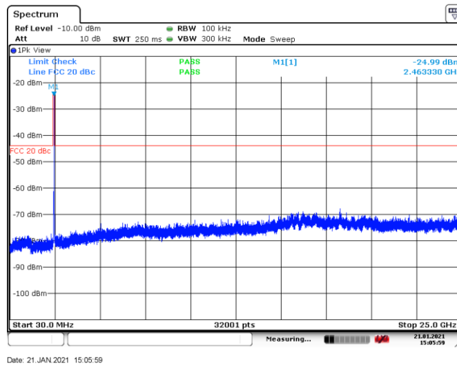
Figure 8.7-5: Conducted spurious emissions, Tx on high channel
