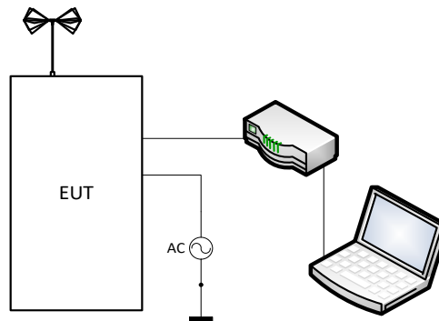
Figure 5.6-1: Testing block diagram
