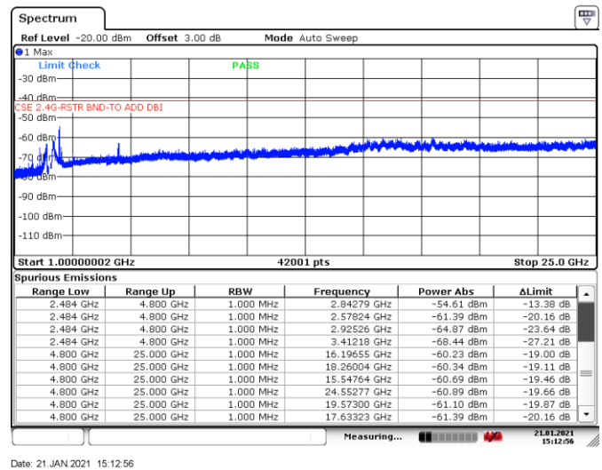
Figure 8.7-14: Conducted spurious emissions above 1 GHz within restricted bands, Tx on mid channel
