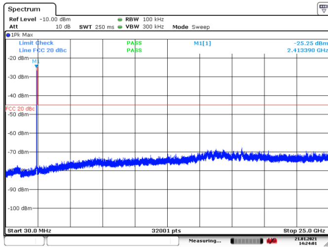
Figure 8.7-3: Conducted spurious emissions, Tx on low channel
