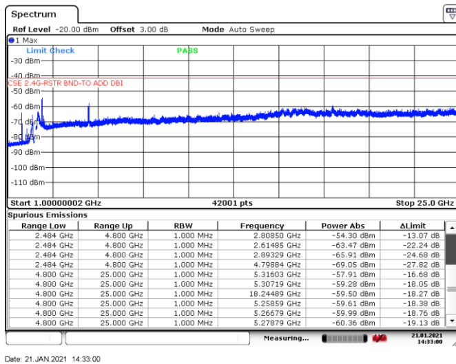
Figure 8.7-13: Conducted spurious emissions above 1 GHz within restricted bands, Tx on low channel
