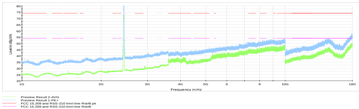
Figure 8.7-20: Cabinet radiated Spurious emissions 1 to 18 GHz, Tx @ mid channel
