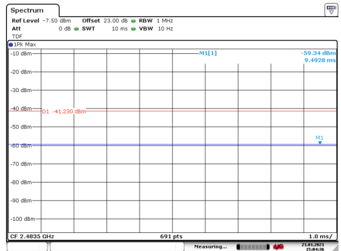
Figure 8.7-9: Conducted spurious emissions on 2483.5 MHz, average, Tx on high channel
