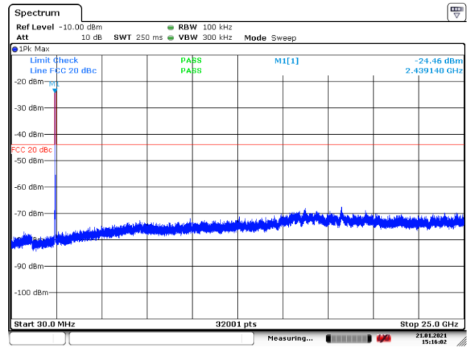
Figure 8.7-4: Conducted spurious emissions, Tx on mid channel
