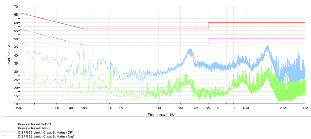
Plot 8.4-1: Conducted emissions on phase line
