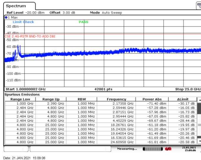
Figure 8.7-15: Conducted spurious emissions above 1 GHz within restricted bands, Tx on high channel
