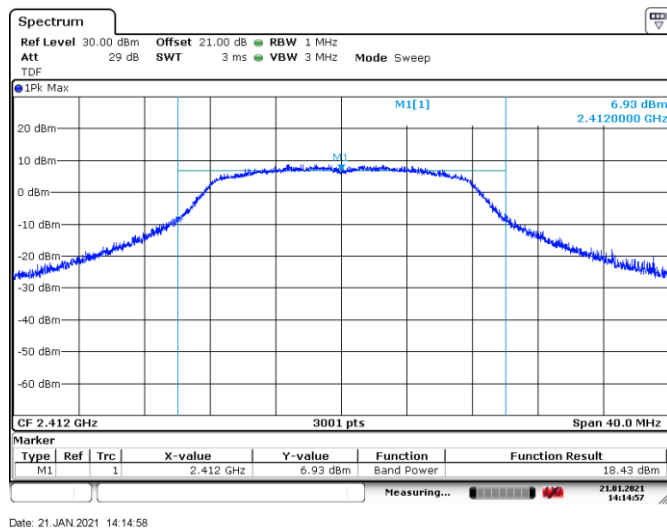
Figure 8.6-1: Output power on low channel
