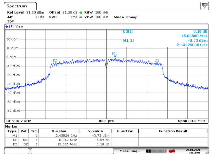
Figure 8.5-2: 6 dB bandwidth on Mid Channel
