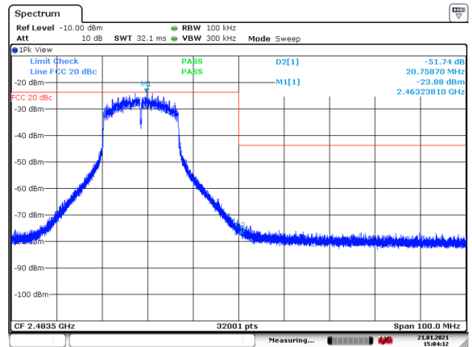
Figure 8.7-2: Conducted Band edge spurious emissions at 2483.5 MHz, Tx on high channel
