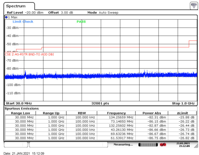
Figure 8.7-11: Conducted spurious emissions 30 MHz to 1 GHz within restricted bands, Tx on mid channel
