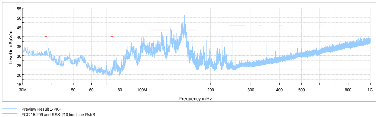
Figure 8.7-18: Cabinet radiated Spurious emissions within 30 to 1000 MHz, Tx @ high channel
