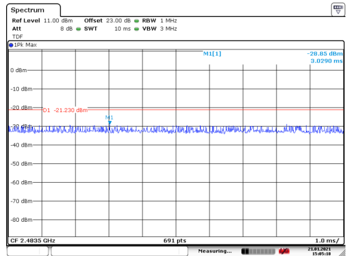
Figure 8.7-7: Conducted spurious emissions on 2483.5 MHz, peak, Tx on high channel
