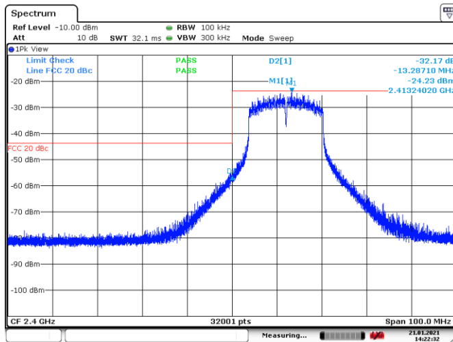
Figure 8.7-1: Conducted Band edge spurious emissions at 2400 MHz, Tx on low channel
