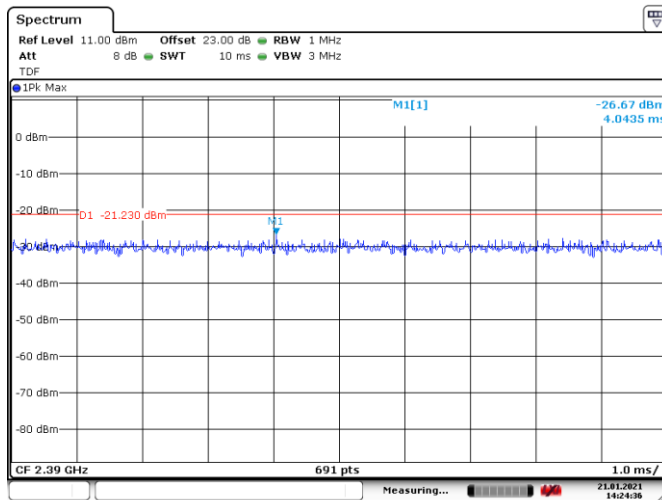
Figure 8.7-6: Conducted spurious emissions on 2390 MHz, peak, Tx on low channel
