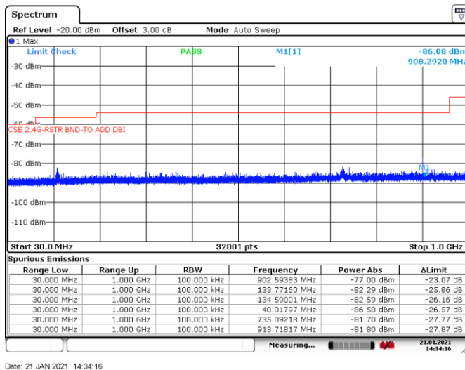
Figure 8.7-10: Conducted spurious emissions 30 MHz to 1 GHz within restricted bands, Tx on low channel
