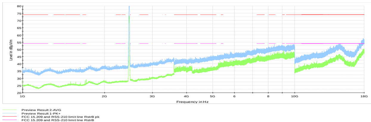
Figure 8.7-21: Cabinet radiated Spurious emissions 1 to 18 GHz, Tx @ high channel
