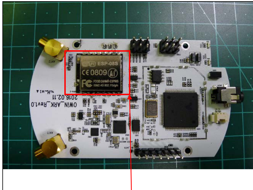
Remove shield can(WLAN Module)
