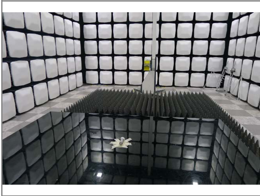
Photo of radiated spurious emission at above 1 000MHz (DC 3.7 V)
