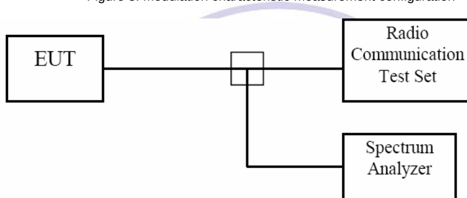
Figure 3: Modulation characteristic measurement configuration
