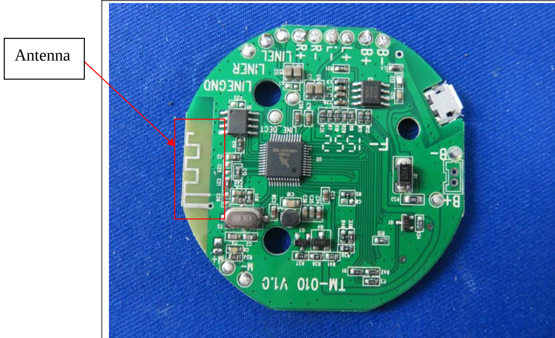
PCB of the EUT-Front View
